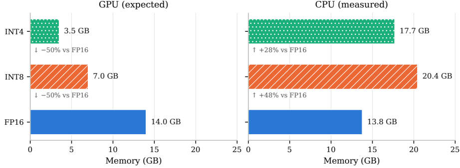
Fig. 1 Memory paradox: GPU quantization reduces memory by 50% while CPU quantization increases it by 48% through dual-representation overhead
