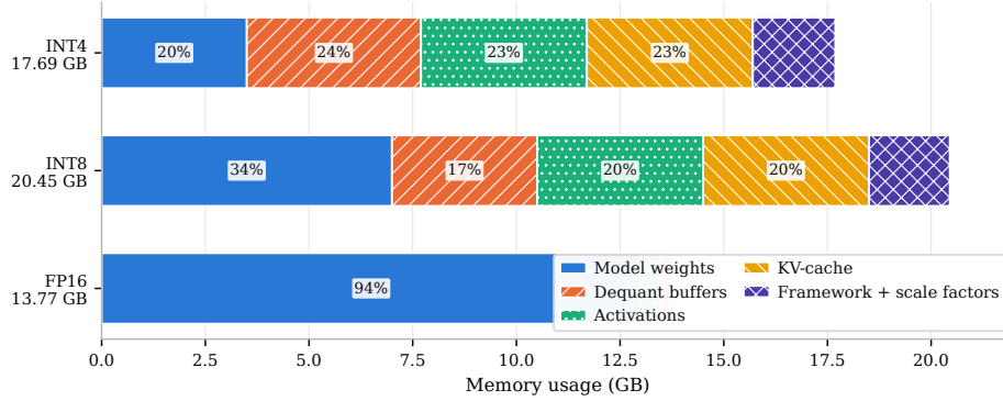
Fig. 2 Estimated memory decomposition for Mistral-7B, plotting the Table 3 values with scale factors folded into the framework segment. Quantization shrinks weights but adds buffers and overhead, raising the total. Only the total is measured
