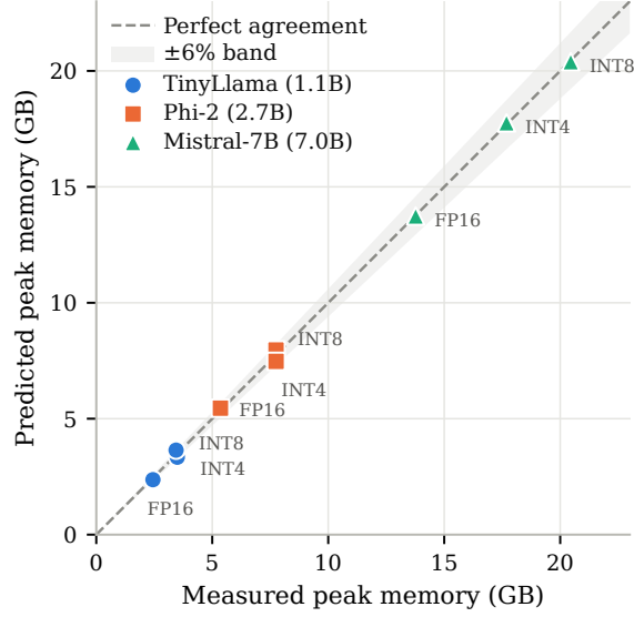
Fig. 3 Predicted versus measured peak memory for all nine configurations. The dashed line marks perfect agreement and the shaded band 6%. All points fall inside the band, and accuracy improves with model size
