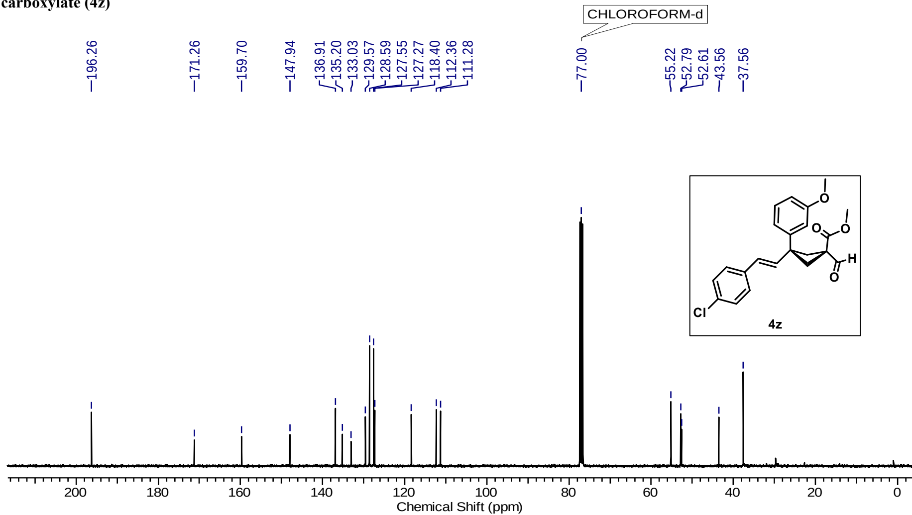
^{13}\text{C}\{^1\text{H}\} NMR (101 MHz, \text{CDCl}_3 ) spectrum of Methyl (1s,3s)-3-((E)-4-chlorostyryl)-1-formyl-3-(3-methoxyphenyl)cyclobutane-1-carboxylate (4z)
