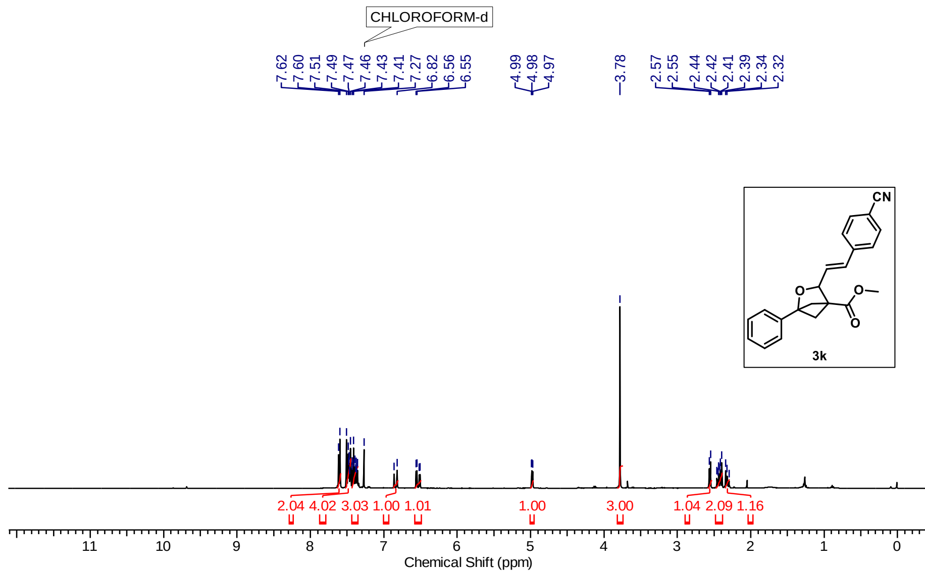
1 H NMR (400 MHz, CDCl 3 ) spectrum of Methyl (E)-3-(4-cyanostyryl)-1-phenyl-2-oxabicyclo[2.1.1]hexane-4-carboxylate (3k)
