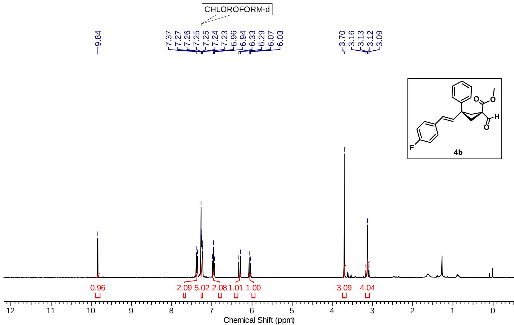
1 H NMR (400 MHz, CDCl 3 ) spectrum of Methyl (1s,3s)-3-((E)-4-fluorostyryl)-1-formyl-3-phenylcyclobutane-1-carboxylate (4b)
