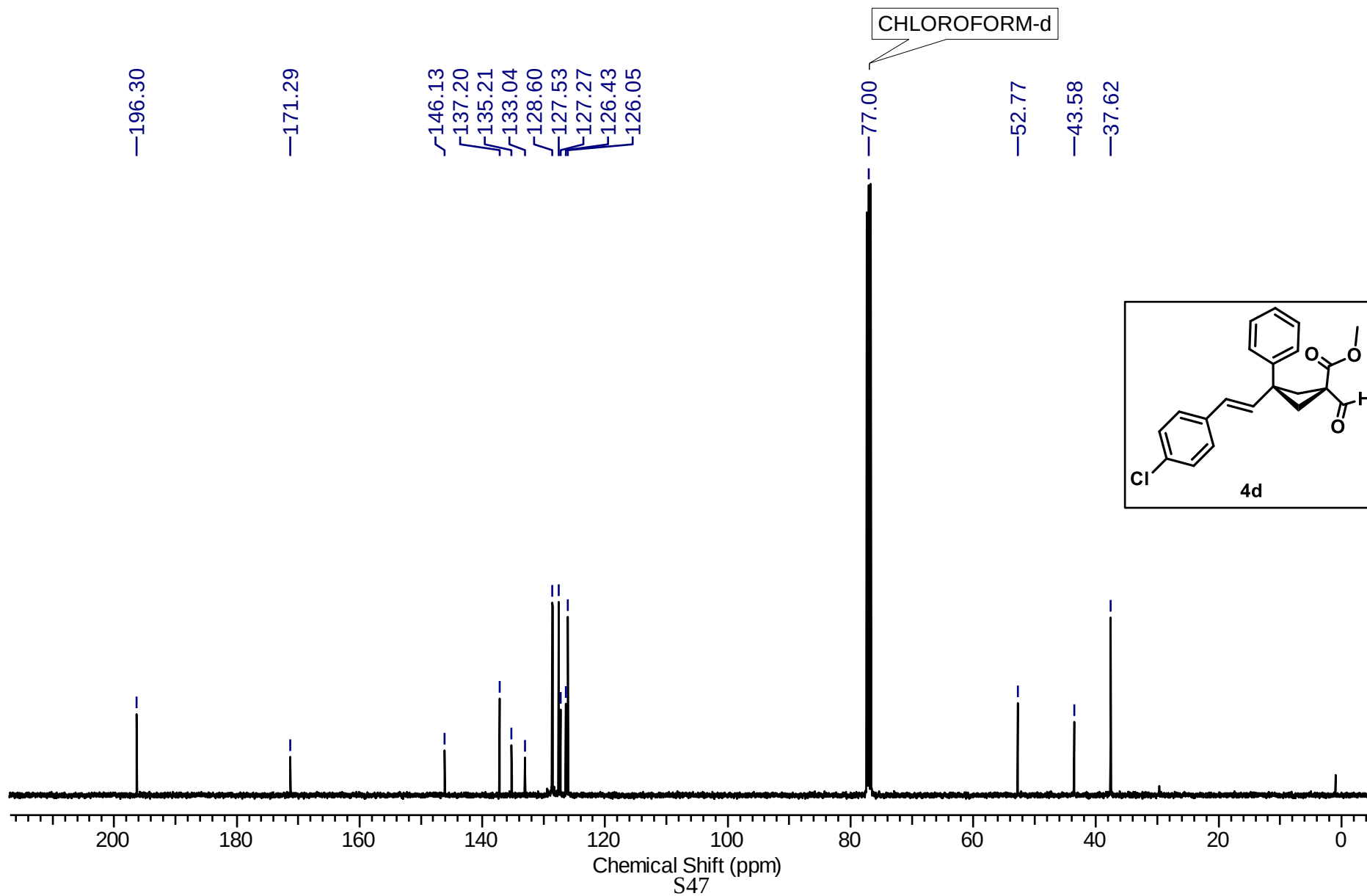
^{13}\text{C}\{^1\text{H}\} NMR (101 MHz, \text{CDCl}_3 ) spectrum of Methyl (1s,3s)-3-((E)-4-chlorostyryl)-1-formyl-3-phenylcyclobutane-1-carboxylate (4d)
