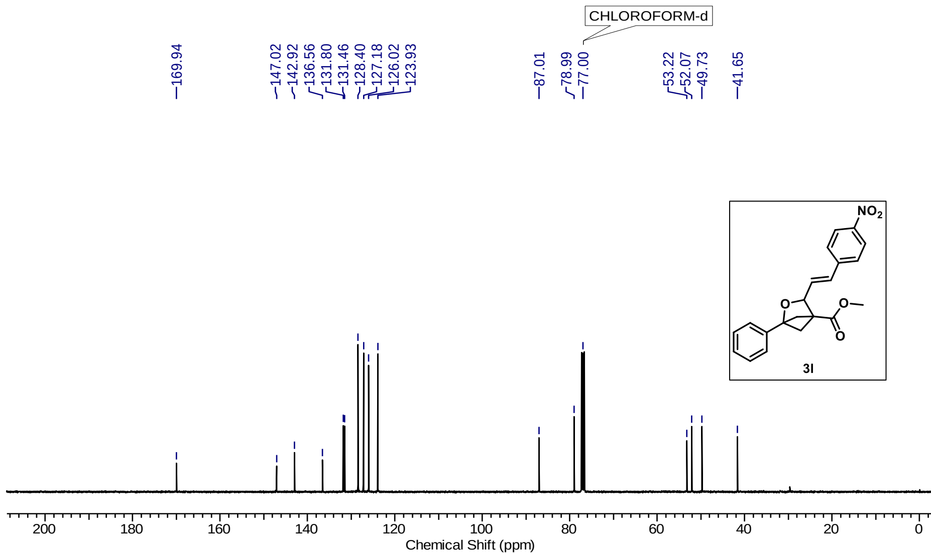
^{13}\text{C}\{^1\text{H}\} NMR (101 MHz, \text{CDCl}_3 ) spectrum of Methyl (E)-3-(4-nitrostyryl)-1-phenyl-2-oxabicyclo[2.1.1]hexane-4-carboxylate (3l)
