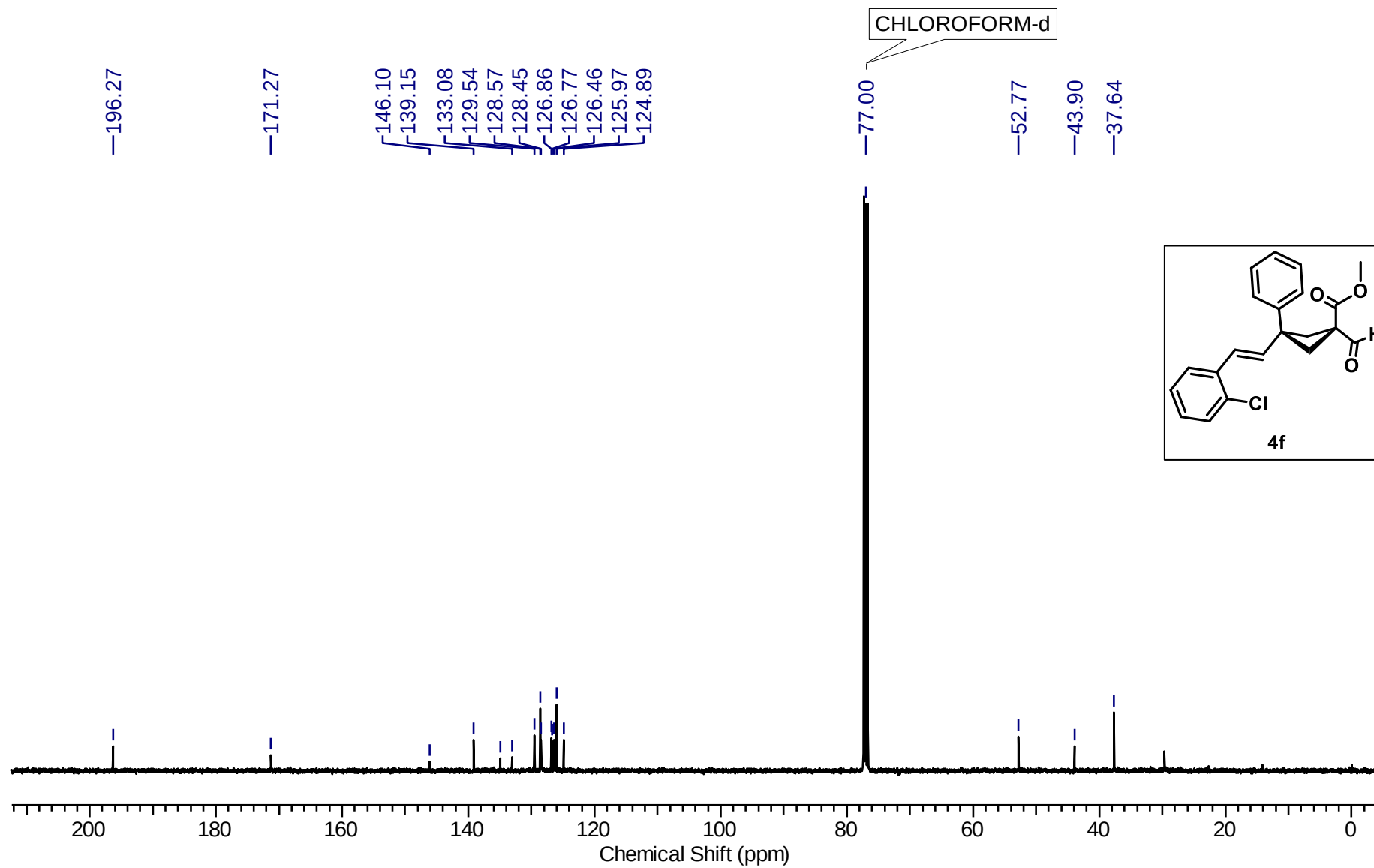
^{13}\text{C}\{^1\text{H}\} NMR (101 MHz, \text{CDCl}_3 ) spectrum of Methyl (1 s ,3 s )-3-(( E )-2-chlorostyryl)-1-formyl-3-phenylcyclobutane-1-carboxylate ( 4f )
