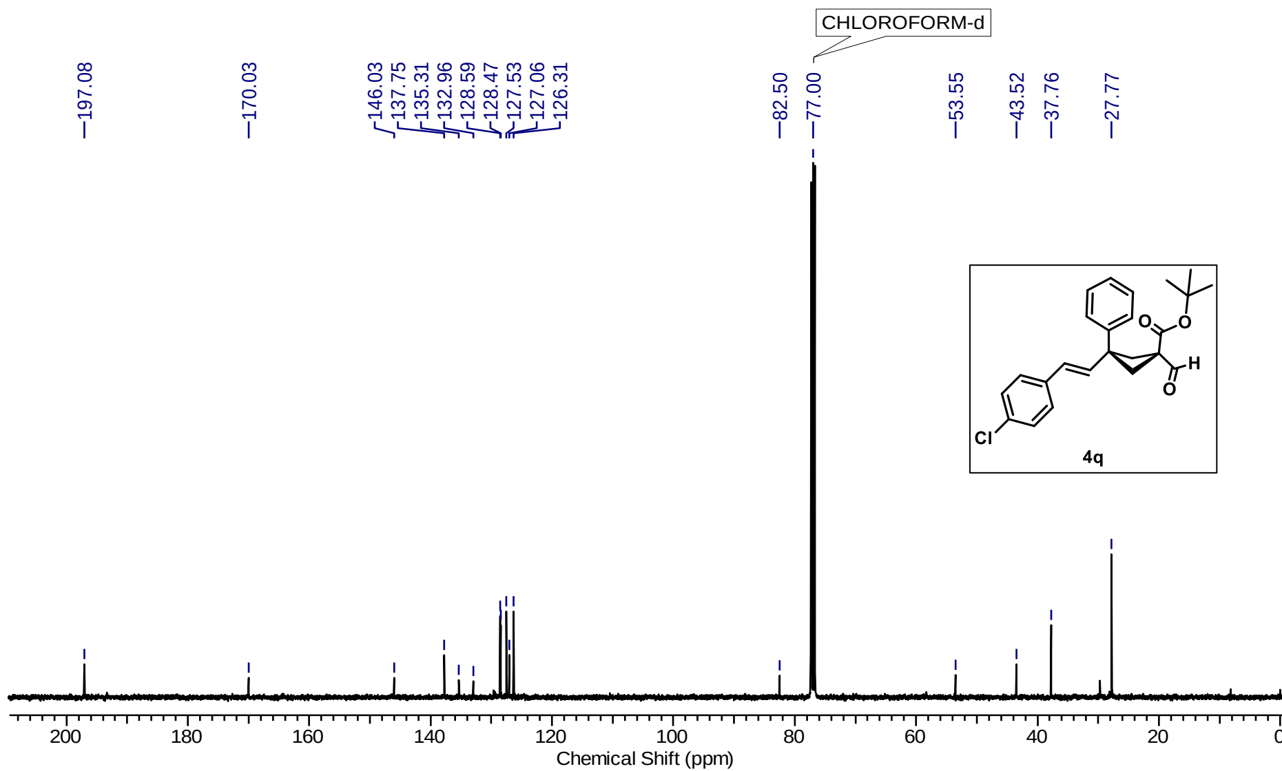
^{13}\text{C}\{^1\text{H}\} NMR (101 MHz, \text{CDCl}_3 ) spectrum of Tert-butyl (1s,3s)-3-((E)-4-chlorostyryl)-1-formyl-3-phenylcyclobutane-1-carboxylate ( 4q )
