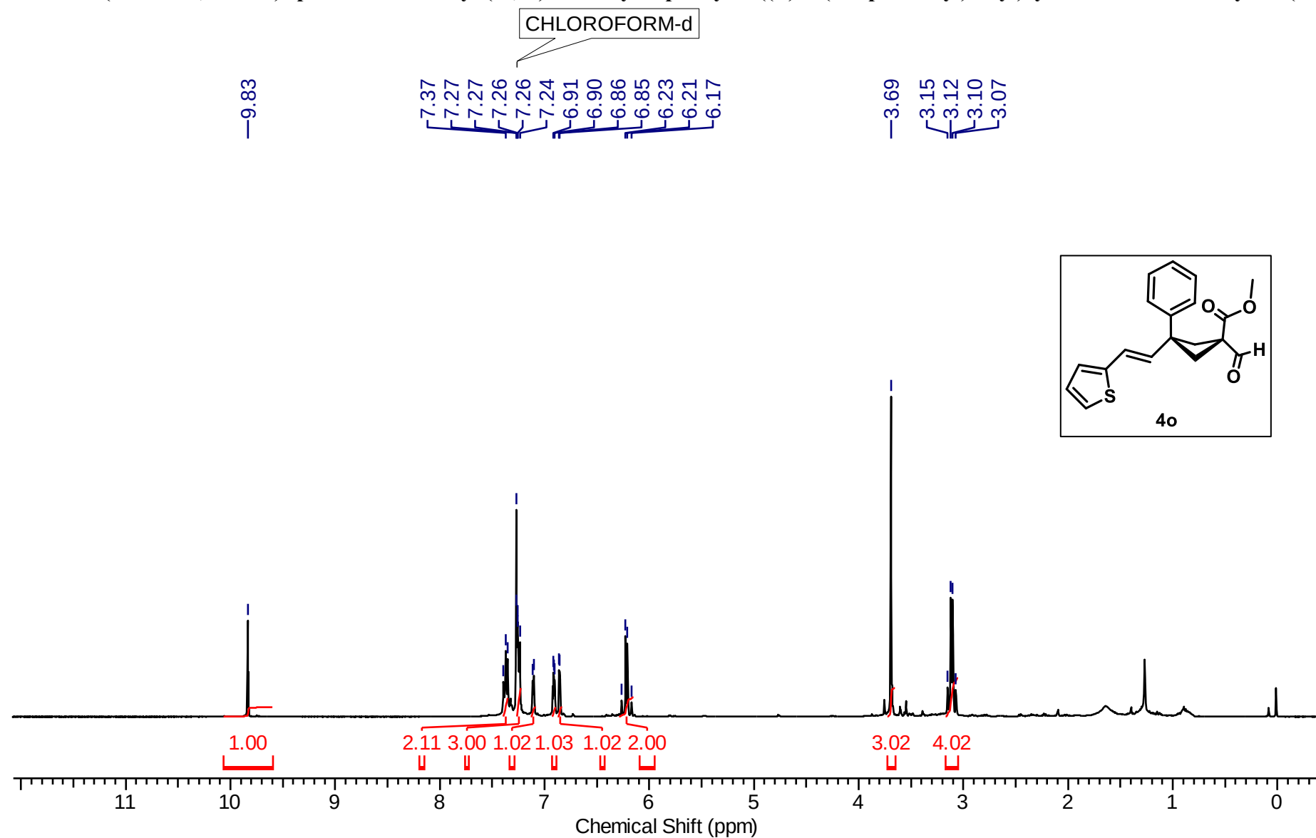
1 H NMR (400 MHz, CDCl 3 ) spectrum of Methyl (1s,3s)-1-formyl-3-phenyl-3-((E)-2-(thiophen-2-yl)vinyl)cyclobutane-1-carboxylate (4o)
