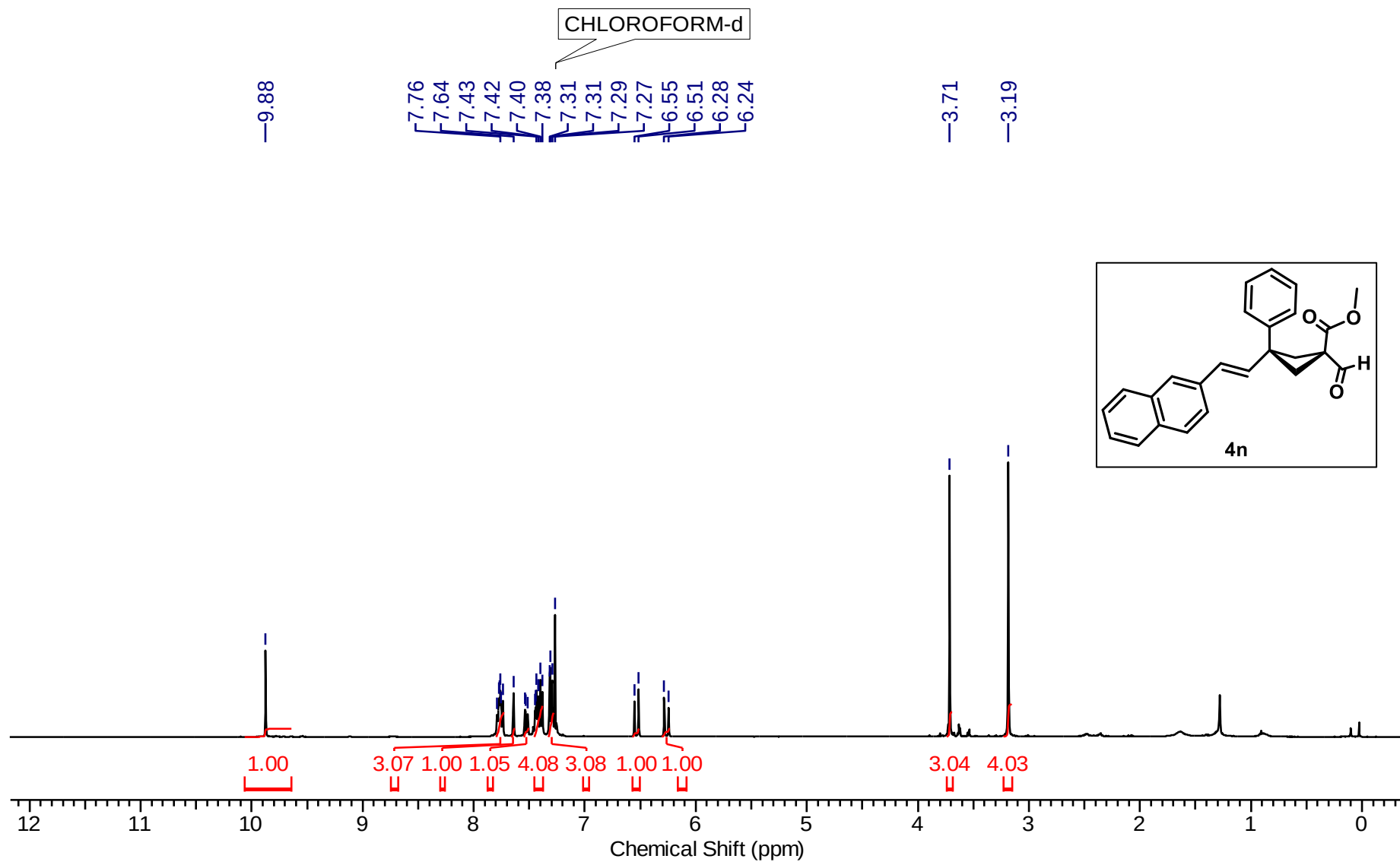
1 H NMR (400 MHz, CDCl 3 ) spectrum of Methyl (1s,3s)-1-formyl-3-((E)-2-(naphthalen-2-yl)vinyl)-3-phenylcyclobutane-1-carboxylate (4n)
