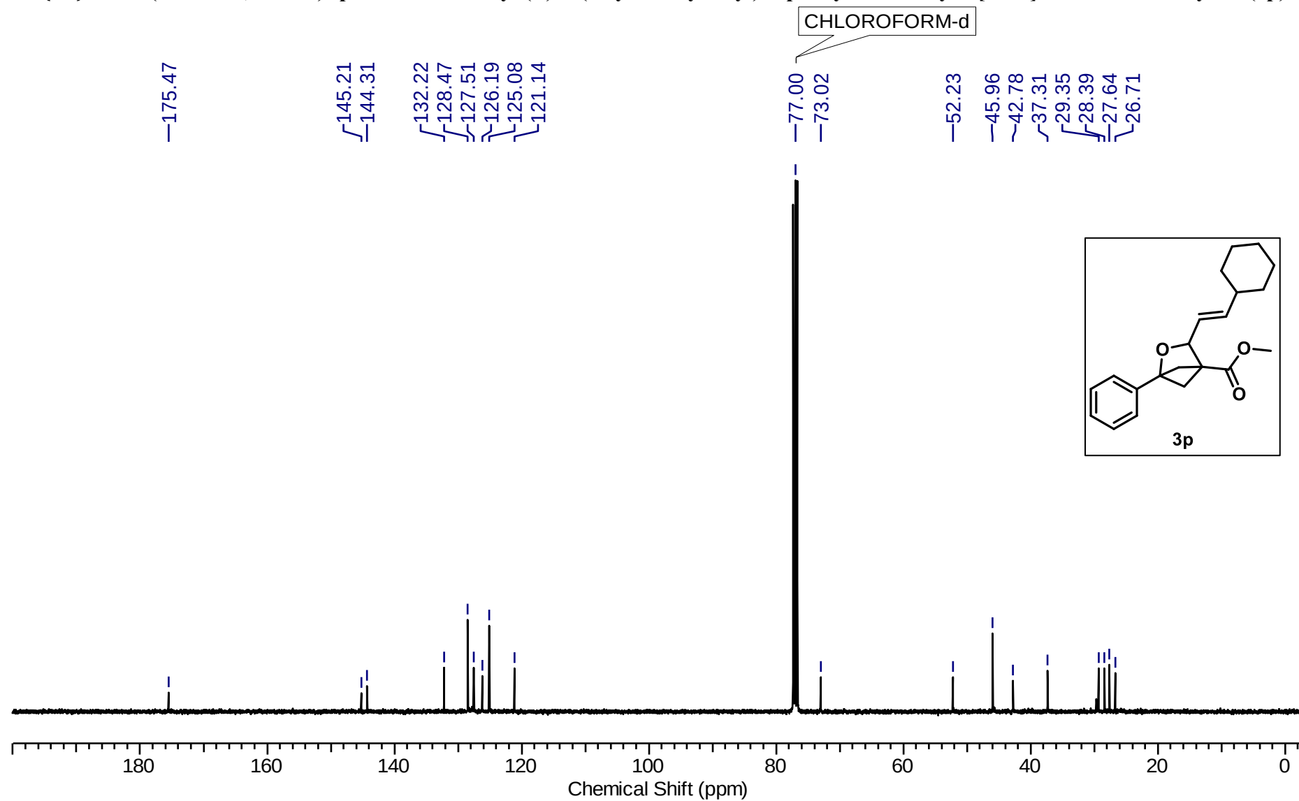
^{13}\text{C}\{^1\text{H}\} NMR (101 MHz, \text{CDCl}_3 ) spectrum of Methyl (E)-3-(2-cyclohexylvinyl)-1-phenyl-2-oxabicyclo[2.1.1]hexane-4-carboxylate (3p)
