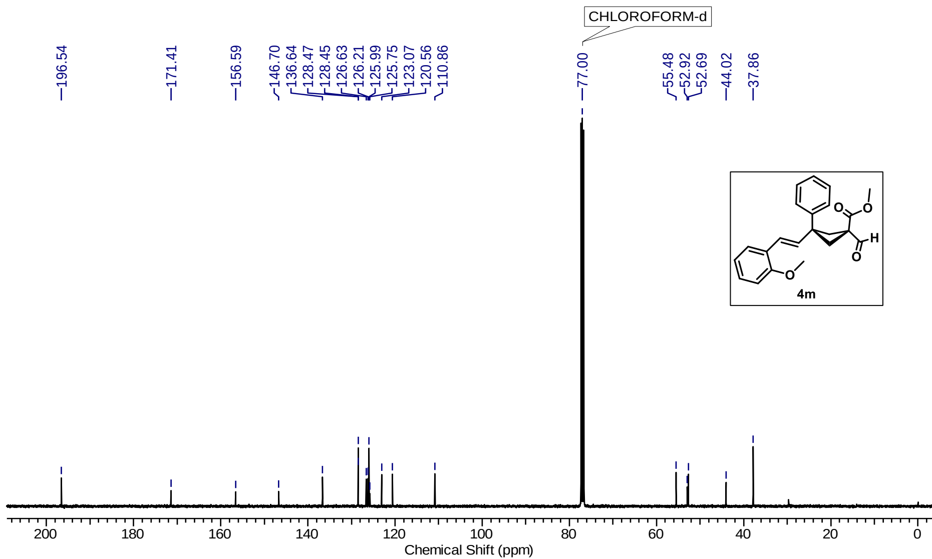
^{13}\text{C}\{^1\text{H}\} NMR (101 MHz, \text{CDCl}_3 ) spectrum of Methyl (1s,3s)-1-formyl-3-((E)-2-methoxystyryl)-3-phenylcyclobutane-1-carboxylate (4m)
