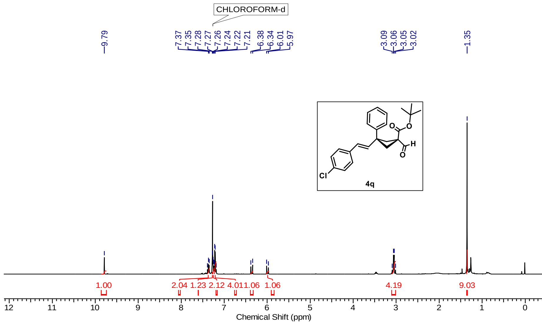
1 H NMR (400 MHz, CDCl 3 ) spectrum of Tert-butyl (1s,3s)-3-((E)-4-chlorostyryl)-1-formyl-3-phenylcyclobutane-1-carboxylate (4q)
