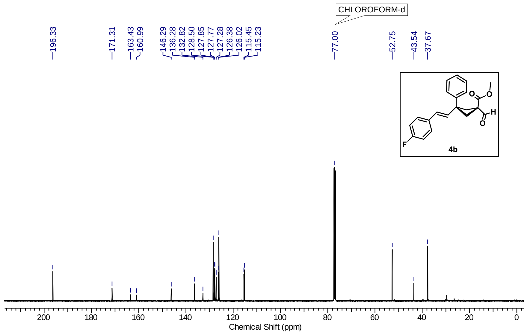
^{13}\text{C}\{^1\text{H}\} NMR (101 MHz, \text{CDCl}_3 ) spectrum of Methyl (1s,3s)-3-((E)-4-fluorostyryl)-1-formyl-3-phenylcyclobutane-1-carboxylate (4b)
