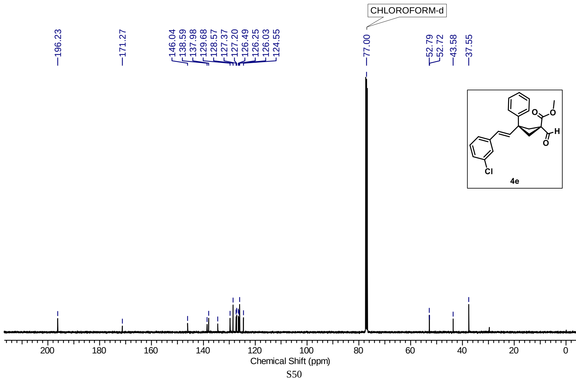
^{13}\text{C}\{^1\text{H}\} NMR (101 MHz, \text{CDCl}_3 ) spectrum of Methyl (1s,3s)-3-((E)-3-chlorostyryl)-1-formyl-3-phenylcyclobutane-1-carboxylate (4e)
