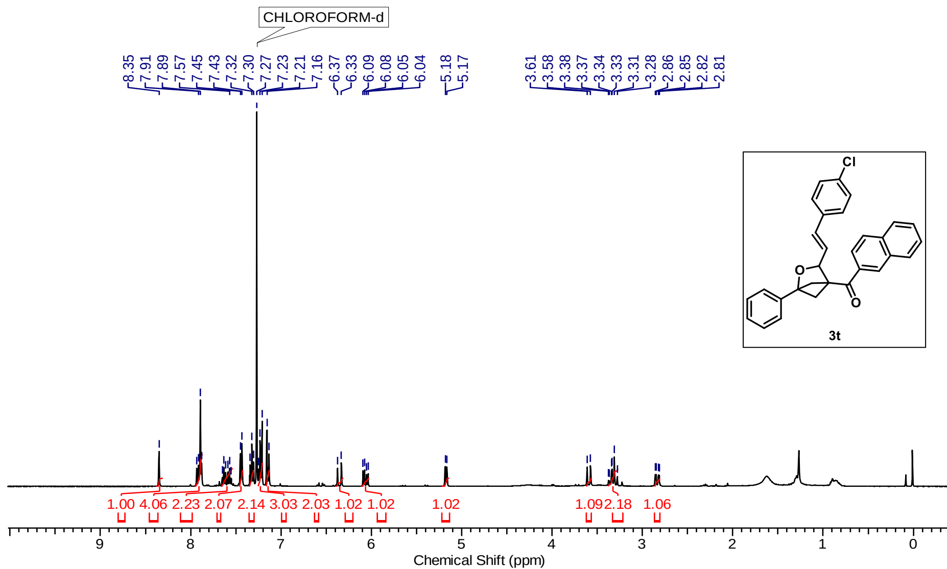
1 H NMR (400 MHz, CDCl 3 ) spectrum of (E)-(3-(4-chlorostyryl)-1-phenyl-2-oxabicyclo[2.1.1]hexan-4-yl)(naphthalen-2-yl)methanone (3t)
