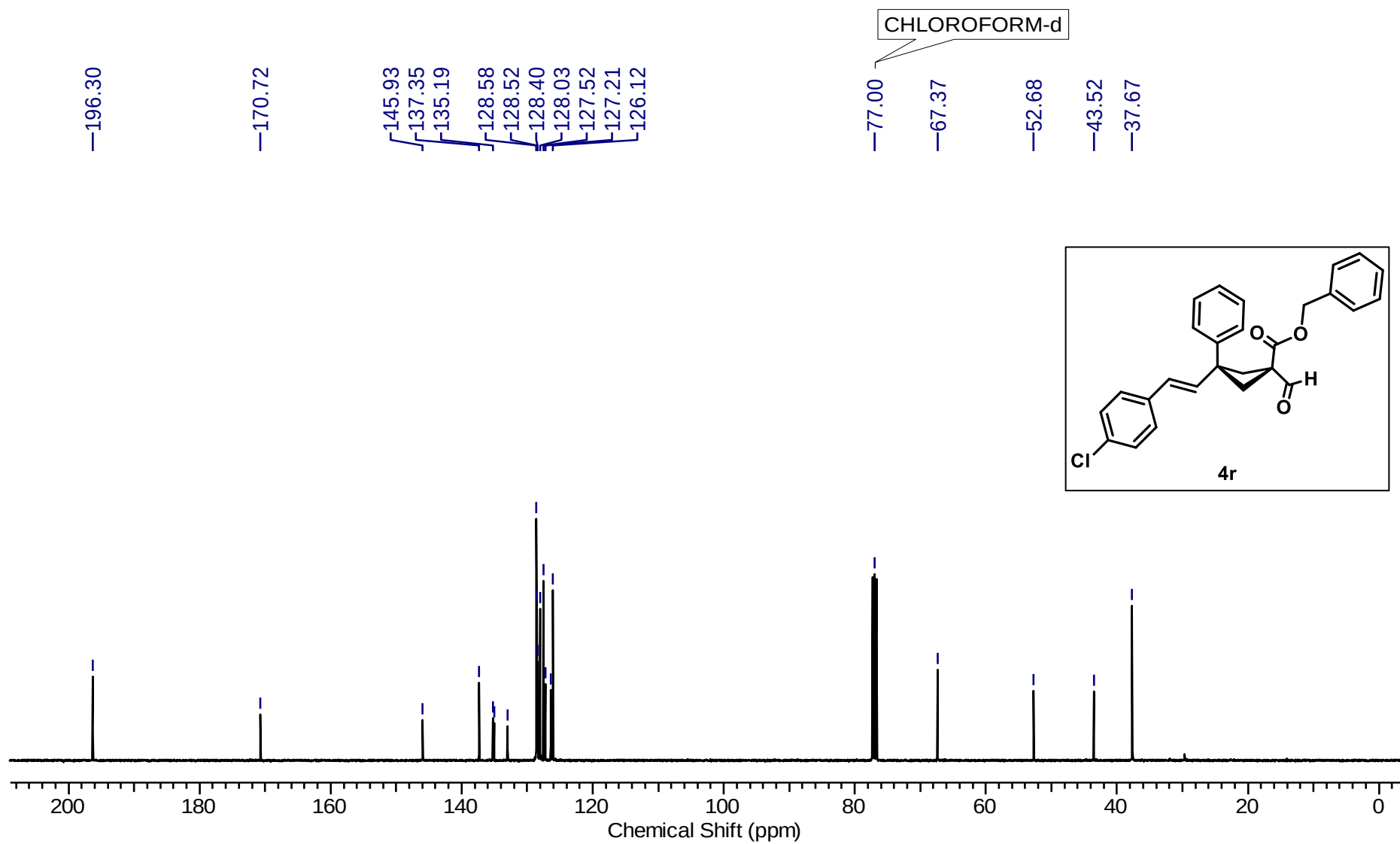
^{13}\text{C}\{^1\text{H}\} NMR (101 MHz, \text{CDCl}_3 ) spectrum of Benzyl (1s,3s)-3-((E)-4-chlorostyryl)-1-formyl-3-phenylcyclobutane-1-carboxylate (4r)
