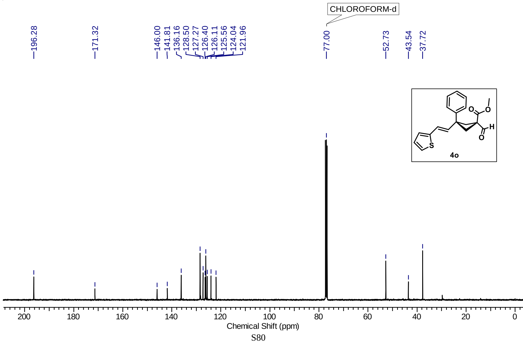
^{13}\text{C}\{^1\text{H}\} NMR (101 MHz, \text{CDCl}_3 ) spectrum of Methyl (1s,3s)-1-formyl-3-phenyl-3-((E)-2-(thiophen-2-yl)vinyl)cyclobutane-1-carboxylate (4o)
