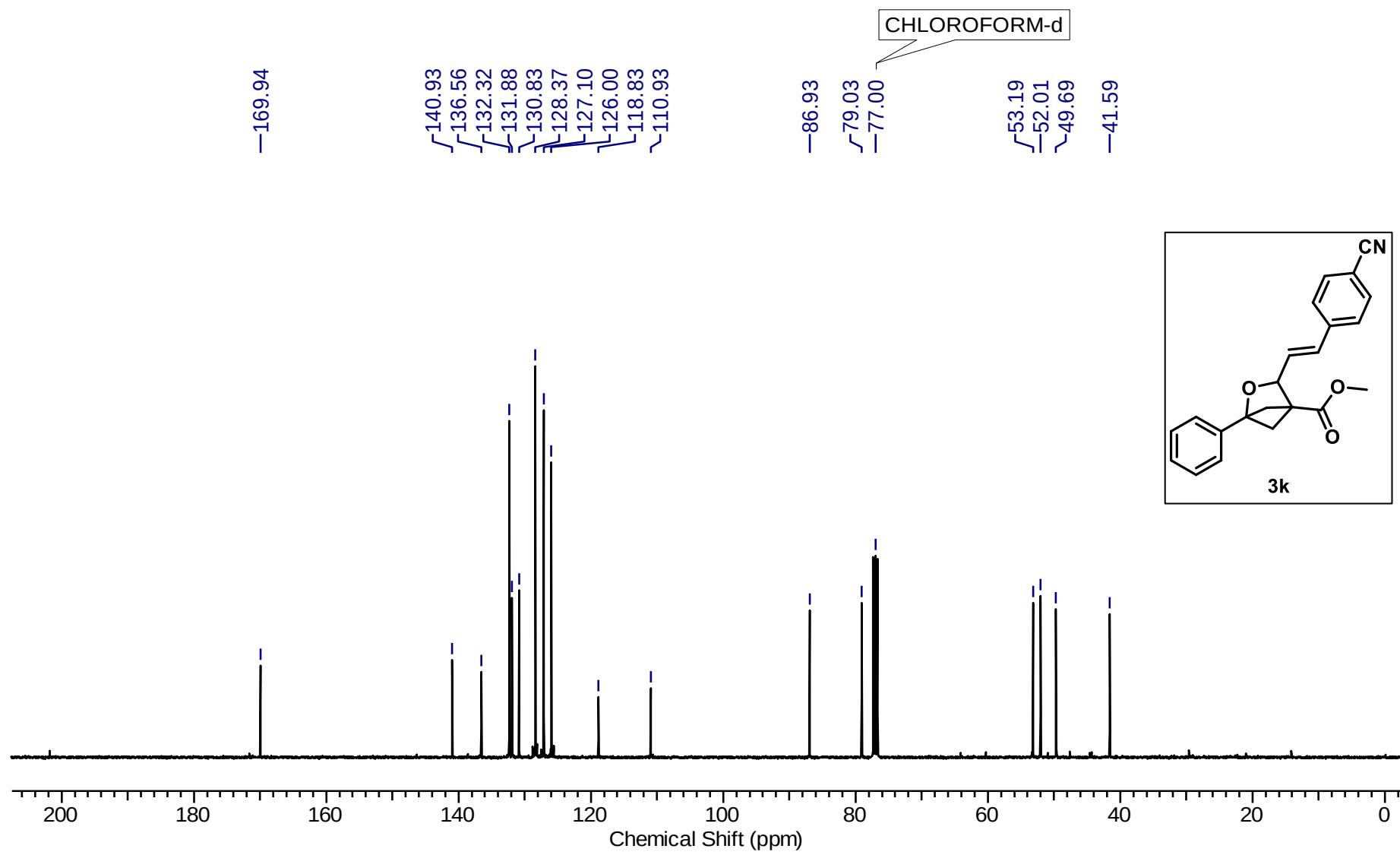
^{13}\text{C}\{^1\text{H}\} NMR (101 MHz, \text{CDCl}_3 ) spectrum of Methyl (E)-3-(4-cyanostyryl)-1-phenyl-2-oxabicyclo[2.1.1]hexane-4-carboxylate ( 3k )
