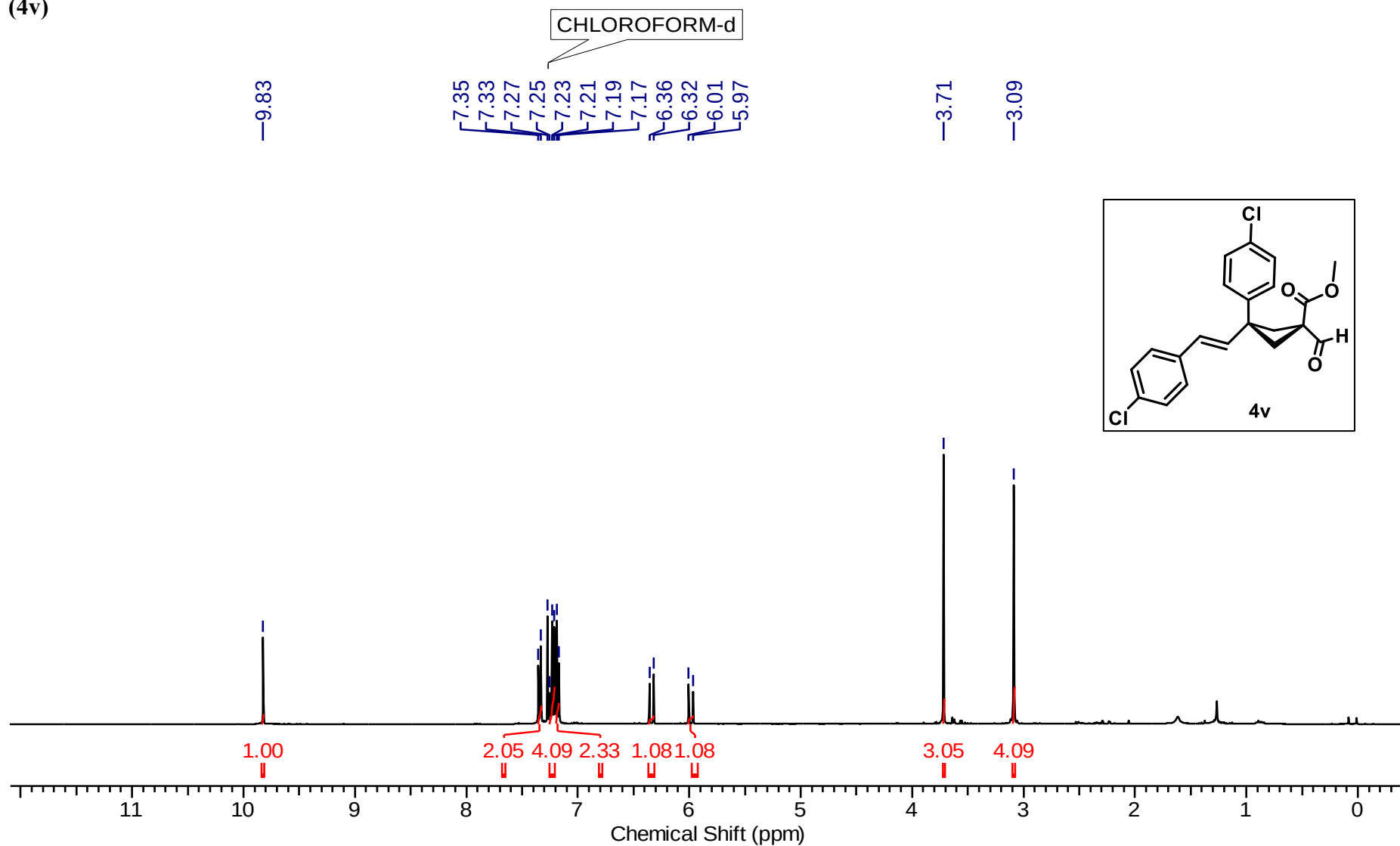
1 H NMR (400 MHz, CDCl 3 ) spectrum of Methyl (1s,3s)-3-(4-chlorophenyl)-3-((E)-4-chlorostyryl)-1-formylcyclobutane-1-carboxylate (4v)
