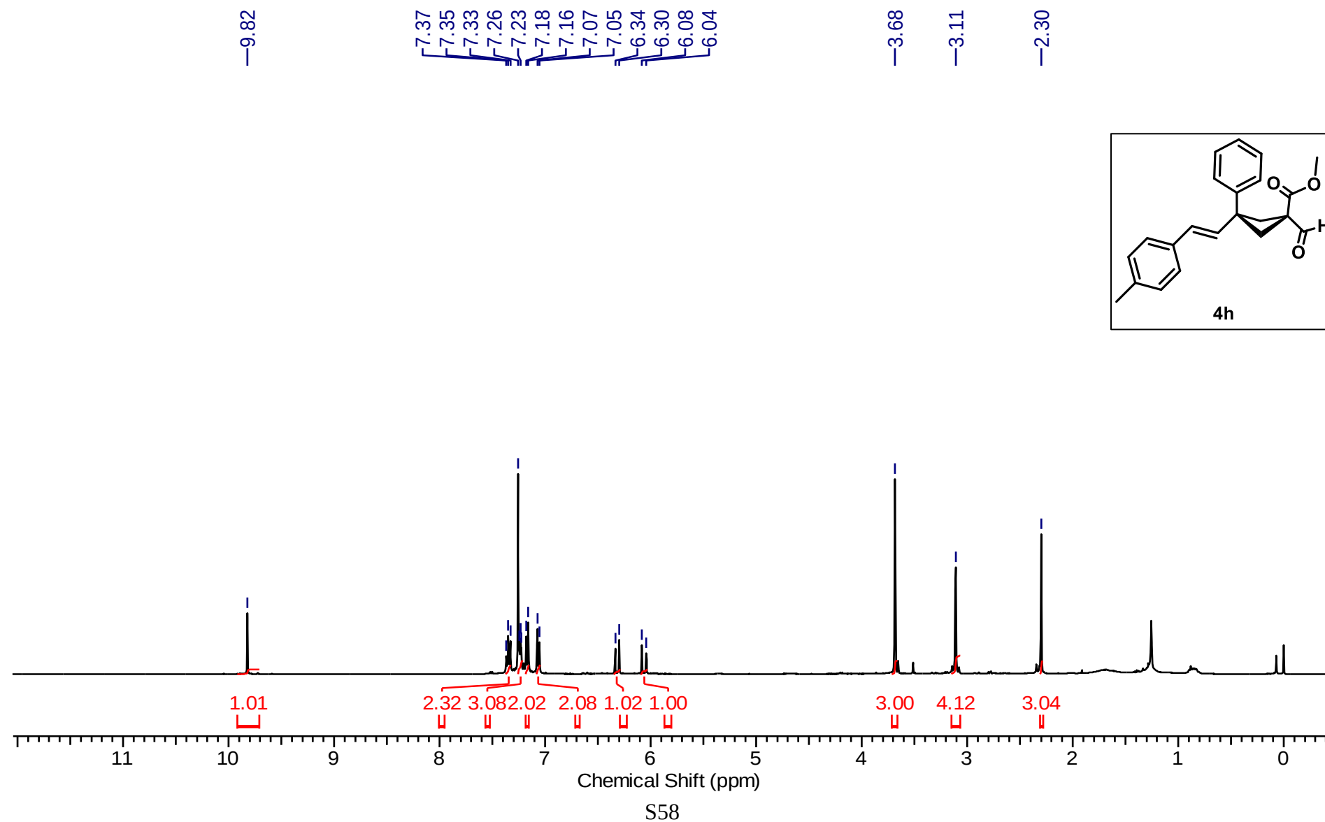
1 H NMR (400 MHz, CDCl 3 ) spectrum of Methyl (1s,3s)-1-formyl-3-((E)-4-methylstyryl)-3-phenylcyclobutane-1-carboxylate (4h)
