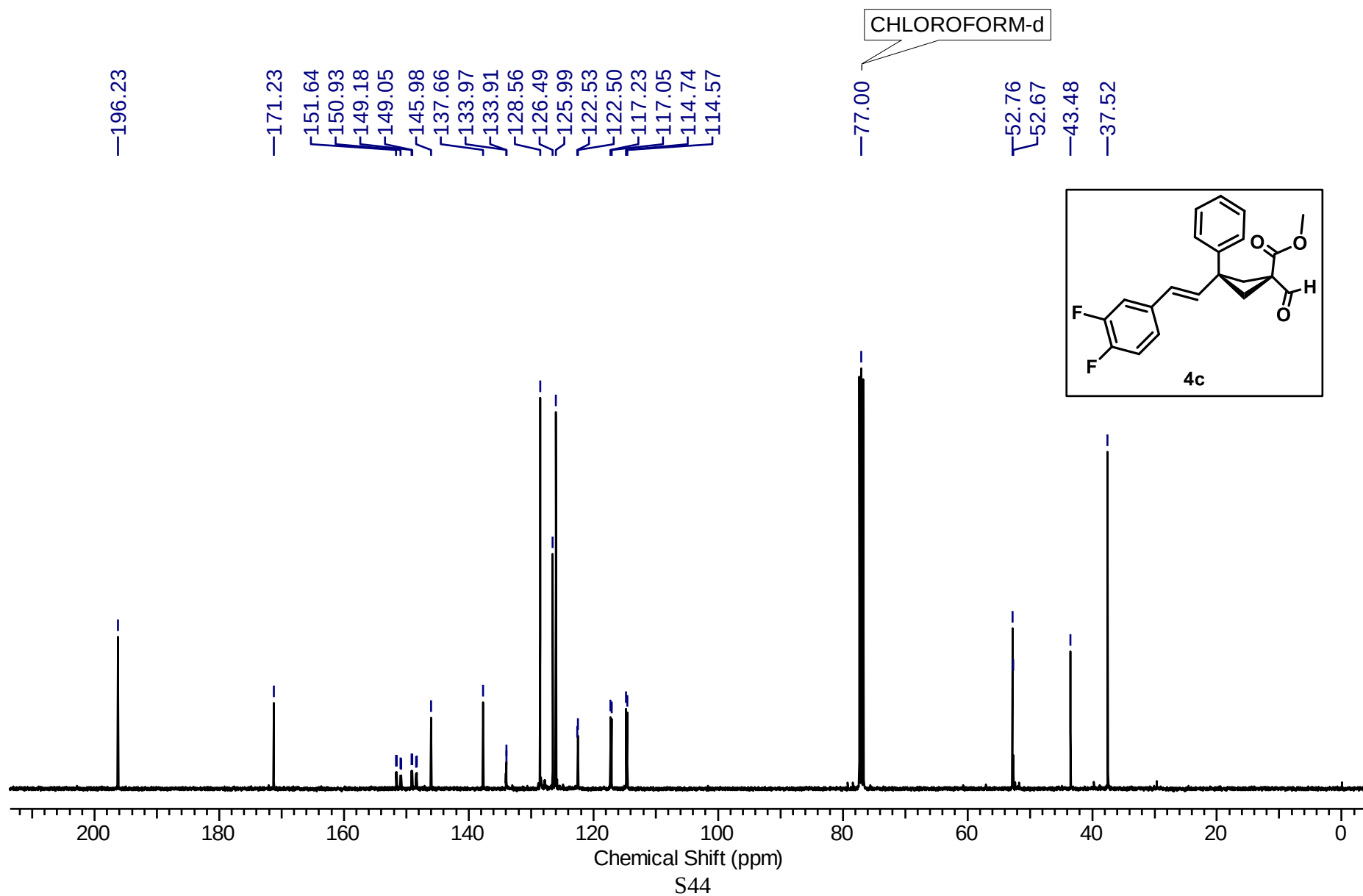
^{13}\text{C}\{^1\text{H}\} NMR (101 MHz, \text{CDCl}_3 ) spectrum of Methyl (1 s ,3 s )-3-(( E )-3,4-difluorostyryl)-1-formyl-3-phenylcyclobutane-1-carboxylate ( 4c )
