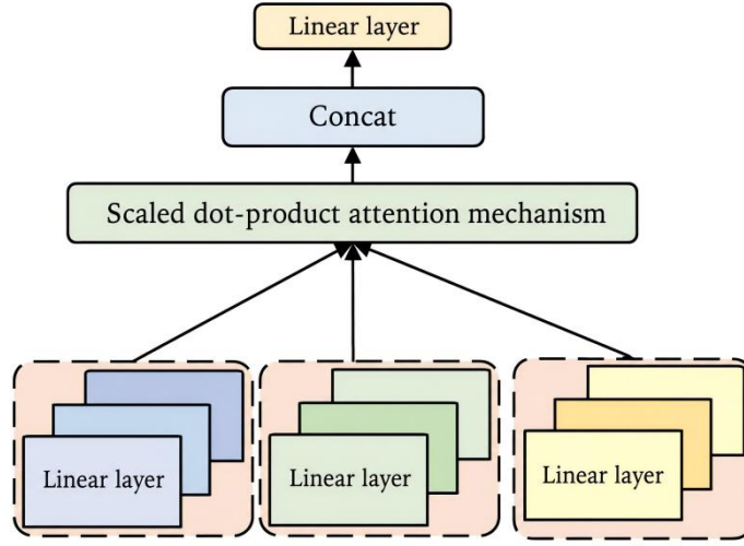
Fig.2 The attention mechanism of the Transformer model
