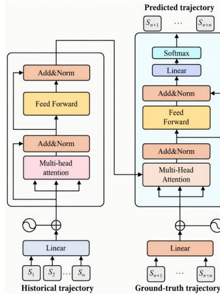
Fig.3 Schematic diagram of the Transformer model structure framework based on the fusion of spatiotemporal features
