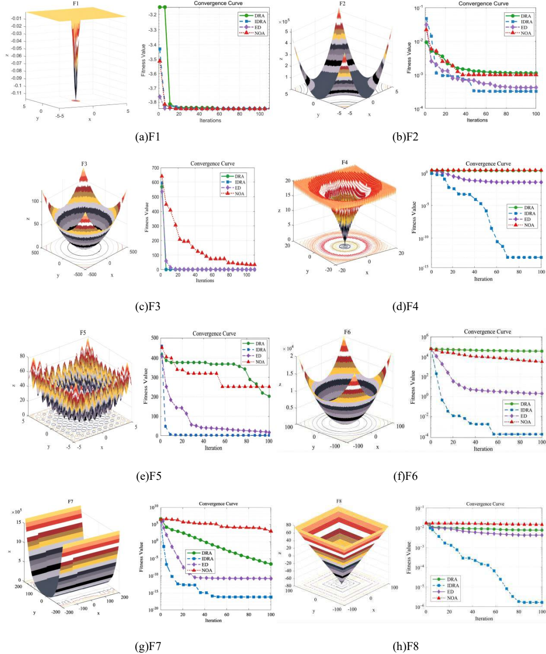
Fig.5 Simulation comparison results of the effectiveness of IDRA algorithm improvement
