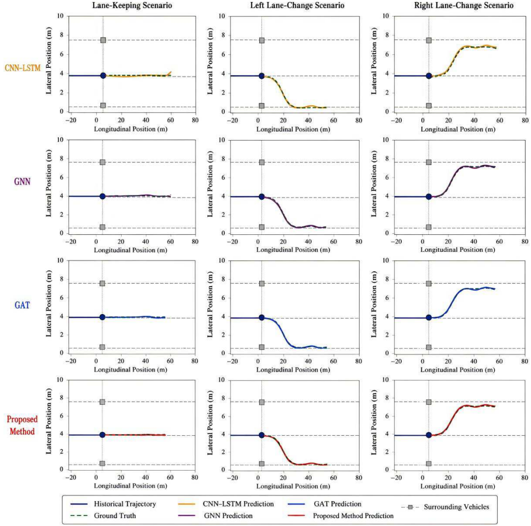
Fig.9 Experimental comparison results of different distributed driving methods for predicting vehicle trajectories and controlling risks in electric vehicles
