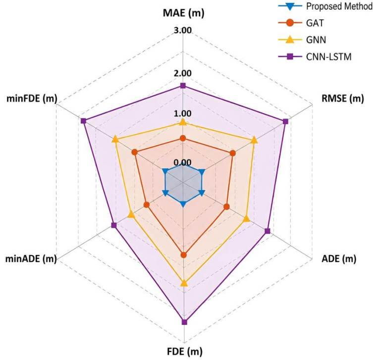
Fig. 10 Multi-index comparison radar chart of different methods
