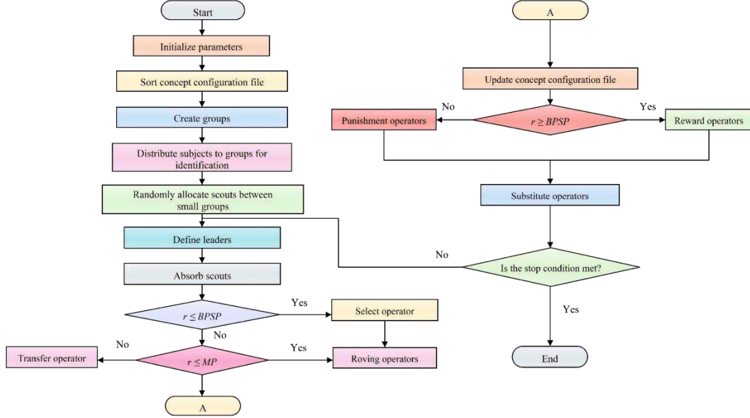
Fig. 1 The calculation flowchart of the DRA algorithm
