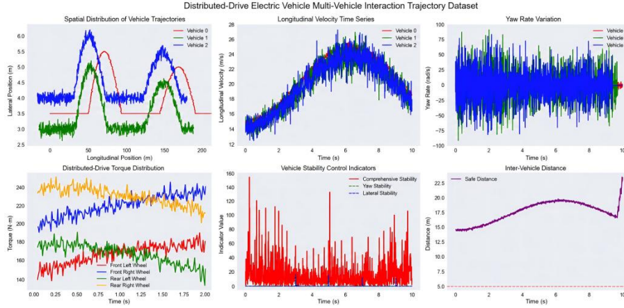
Fig.7 Analysis of dynamic responses and control characteristics of distributed-drive electric vehicle multi-vehicle interacting trajectory data set
