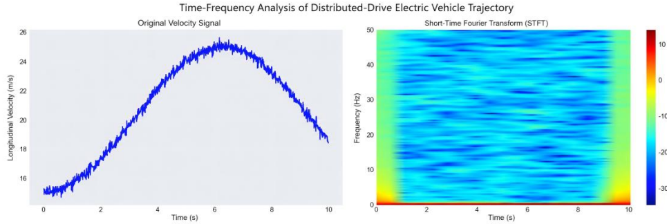
Fig.8 The analysis results of the time-frequency characteristics based on the STFT method
