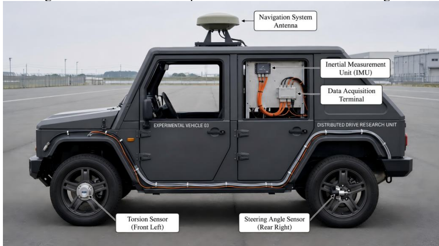
Fig.6 distributed-drive test vehicle
