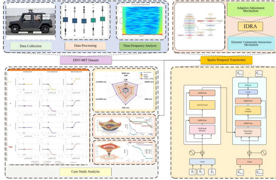
Fig.4 The computational flowchart of the distributed driving trajectory prediction and risk control method for electric vehicles based on the spatiotemporal Transformer and the improved DRA algorithm
