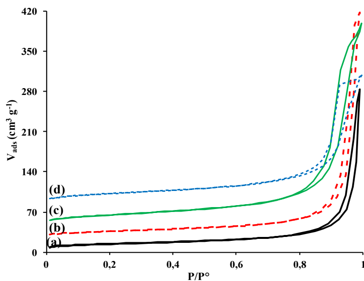
Fig. 3: N 2 -adsorption-desorption isotherms for Au/(HAp) 5 (Cit) x catalysis: (a) x=0; (b) x=1, (c) x=2; (d) x=4
