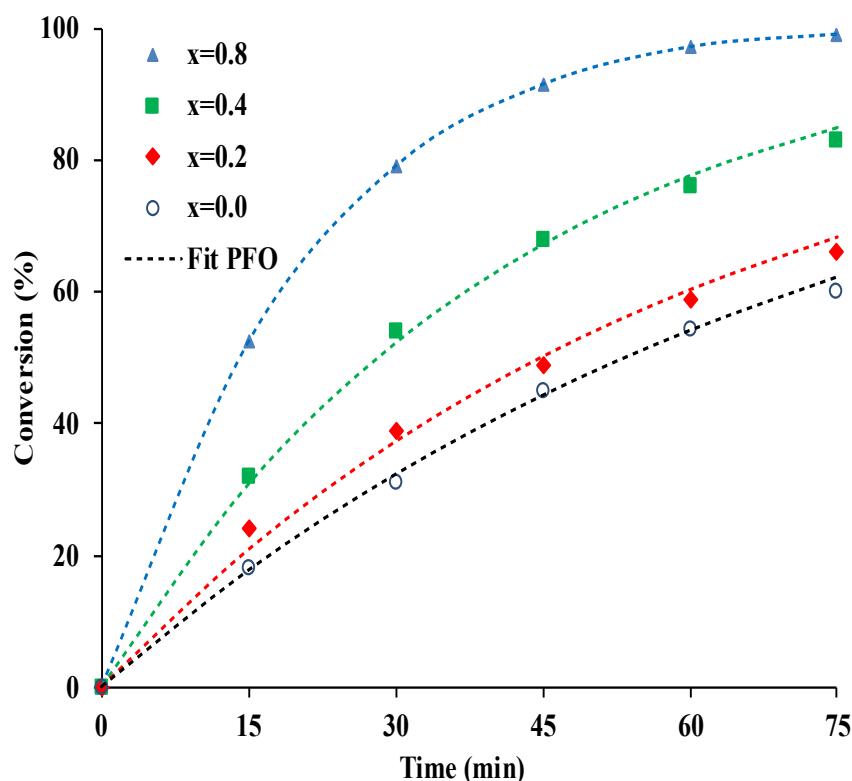
Fig. 7: Oxidation of benzyl alcohol by various gold catalysts
