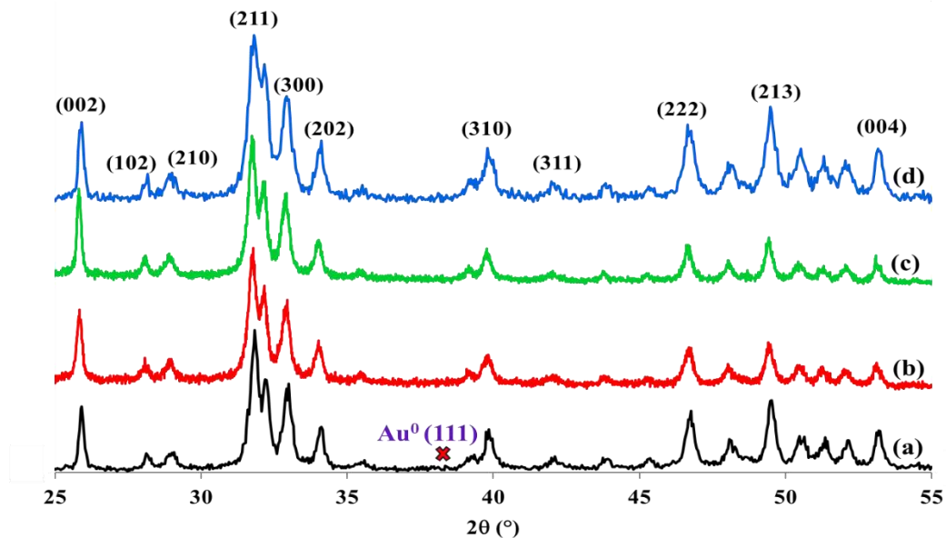
Fig. 1: XRD diffractograms for different catalyst: (a) Au/HAp; (b) Au/(HAp) 5 (Cit) 1 ; (c) Au/(HAp) 5 (Cit) 2 ; (d) Au/(HAp) 5 (Cit) 4
