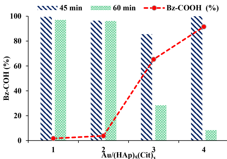
Fig. 8: Effect of time reaction in the Bz-COH selectivity
