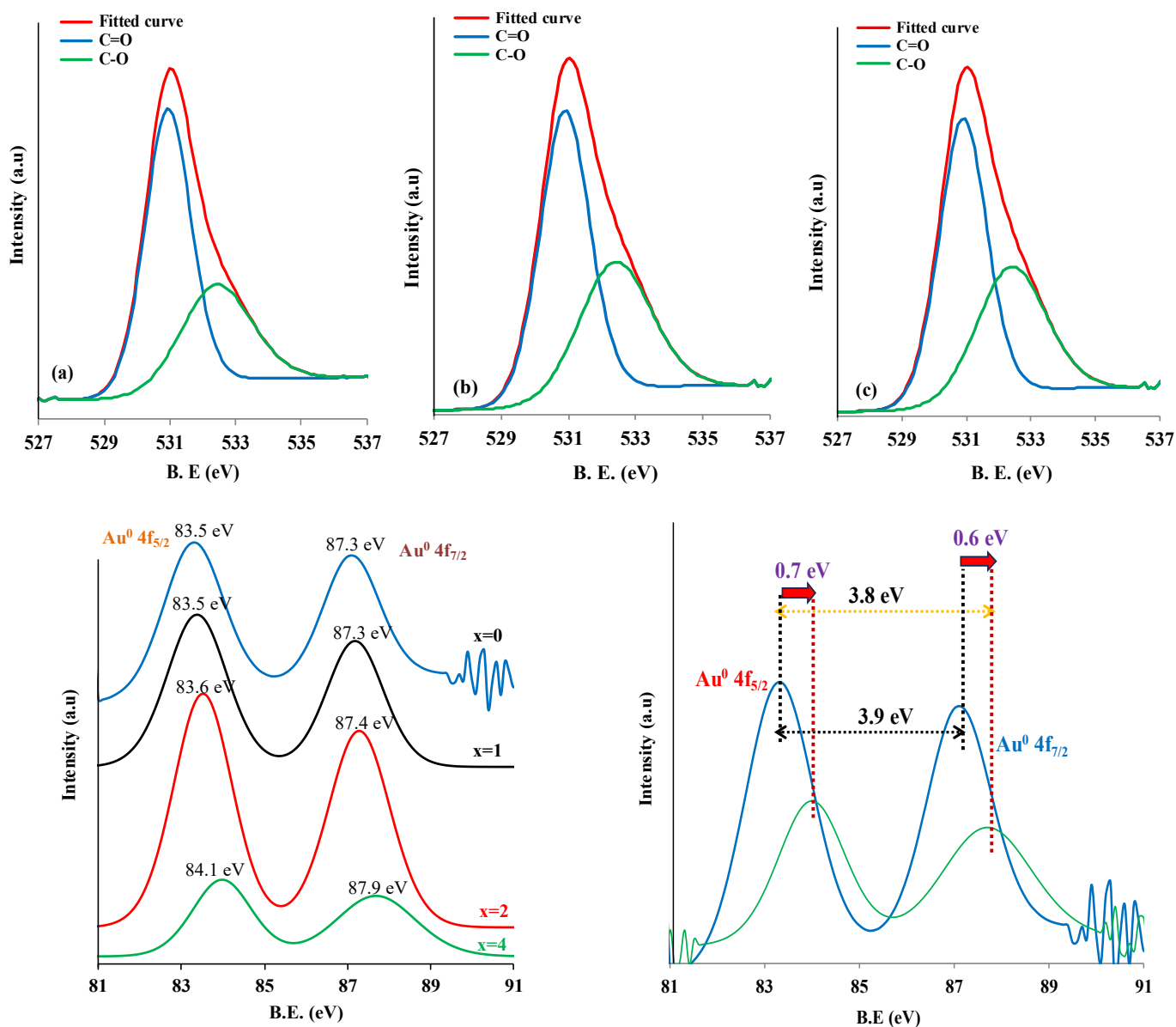
Fig. 4: XPS spectra of different \text{Au}/(\text{HAp})_5(\text{Cit})_x catalysts: A: (a): x=0 ; (b) x=2 ; (c): x=4 and B: (a): XPS spectra and (b) comparative XPS between \text{Au}/\text{HAp} and \text{Au}/(\text{HAp})_5(\text{Cit})_4
