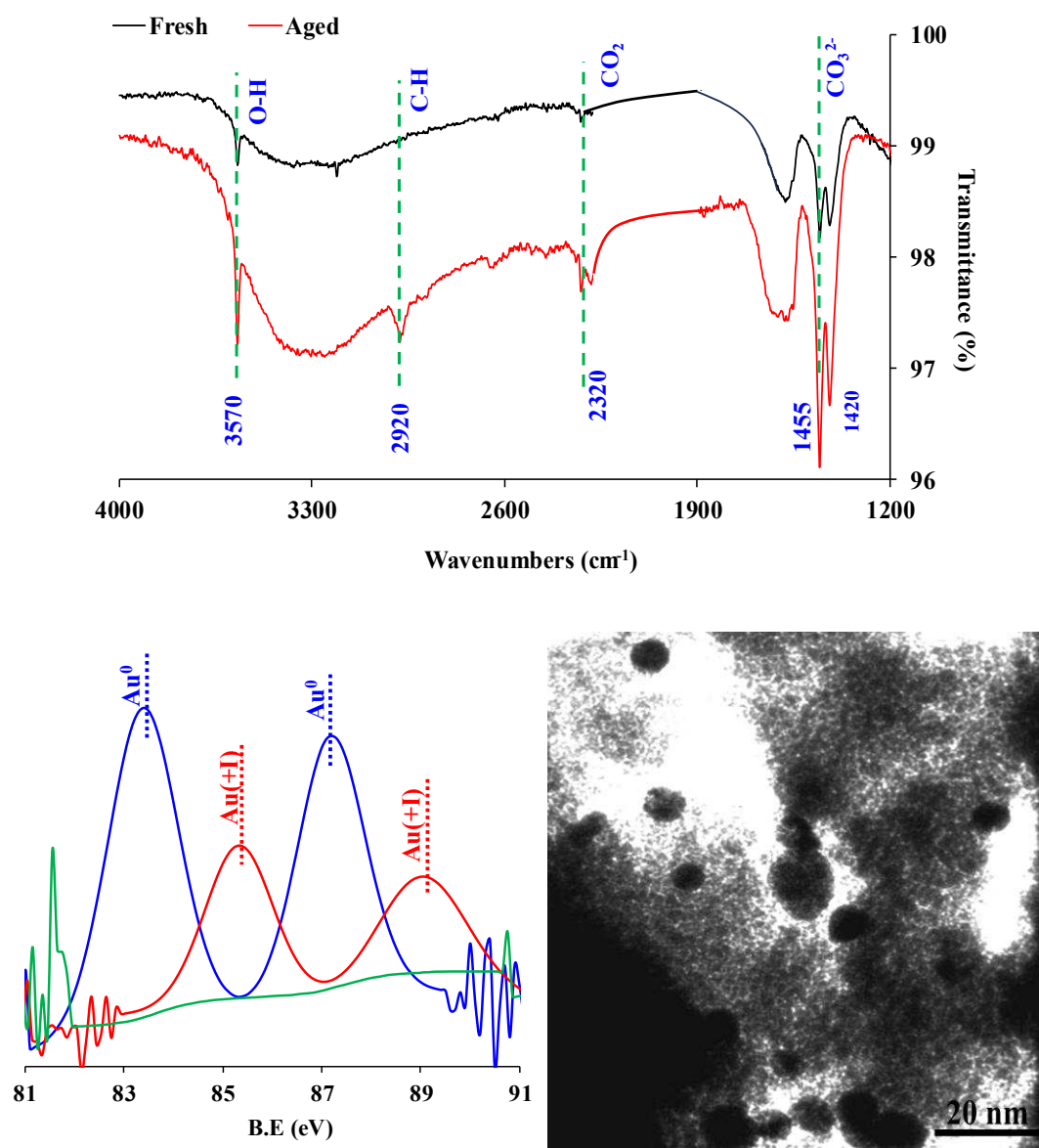
Fig. 11: (A) IR-ATR (B) XPS spectra (C) HR-TEM micrographs for Au/(HAp) 5 (Cit) 4 after 12 months
