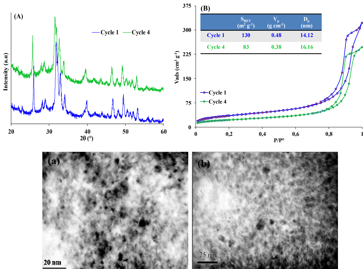
Fig. 10: Effect of Au/(HAp) 5 (Cit) 4 catalyst recycling on structural, textural and morphological properties: (A) XRD, (B) N 2 adsorption-desorption, (a) TEM after cycle 1 and (b) TEM after cycle 4.
