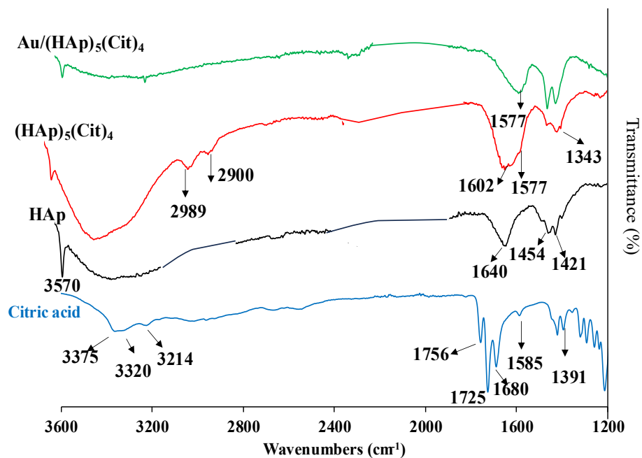
Fig. 2: IR-ATR spectra of Citric acid, HAp, (HAp) 5 (Cit) 4 and Au/(HAp) 5 (Cit) 4
