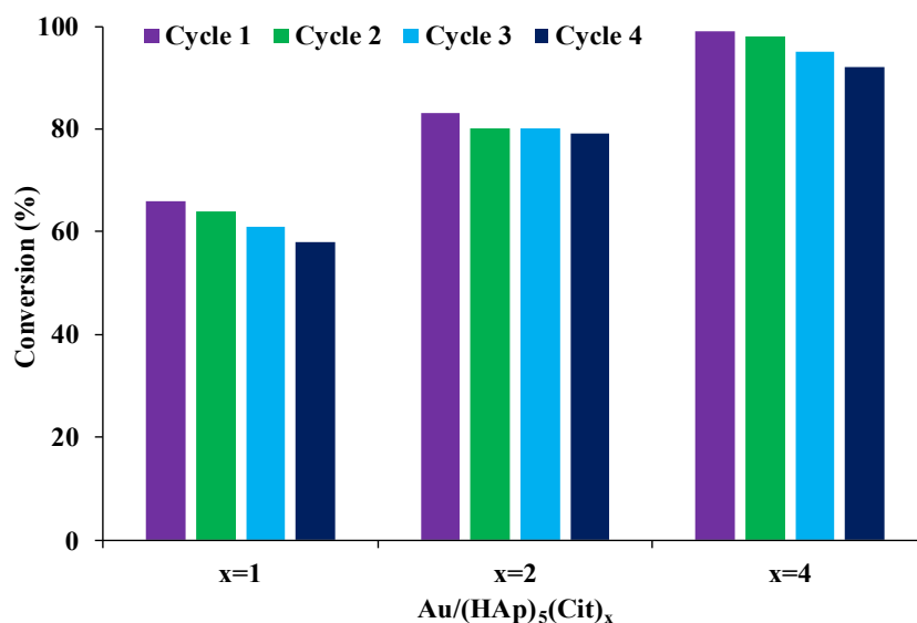
Fig. 9: Conversion stability of the catalysts over recycling cycles
