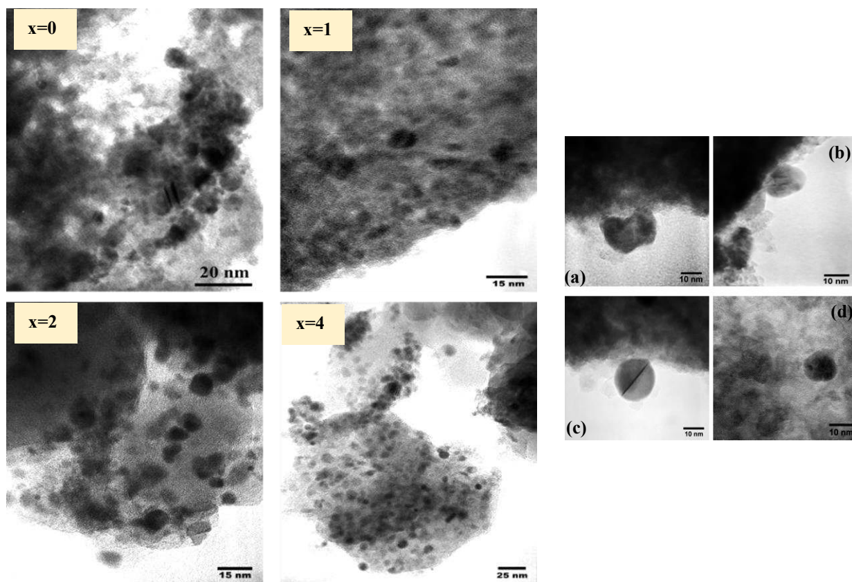
Fig. 5: TEM micrographs of Au/(HAp) 5 (Cit) x : (a) x=0; (b) x=1; (c) x=2 and (d)x=4
