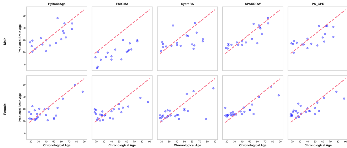
Figure 4: Sex-stratified performance of all models.
