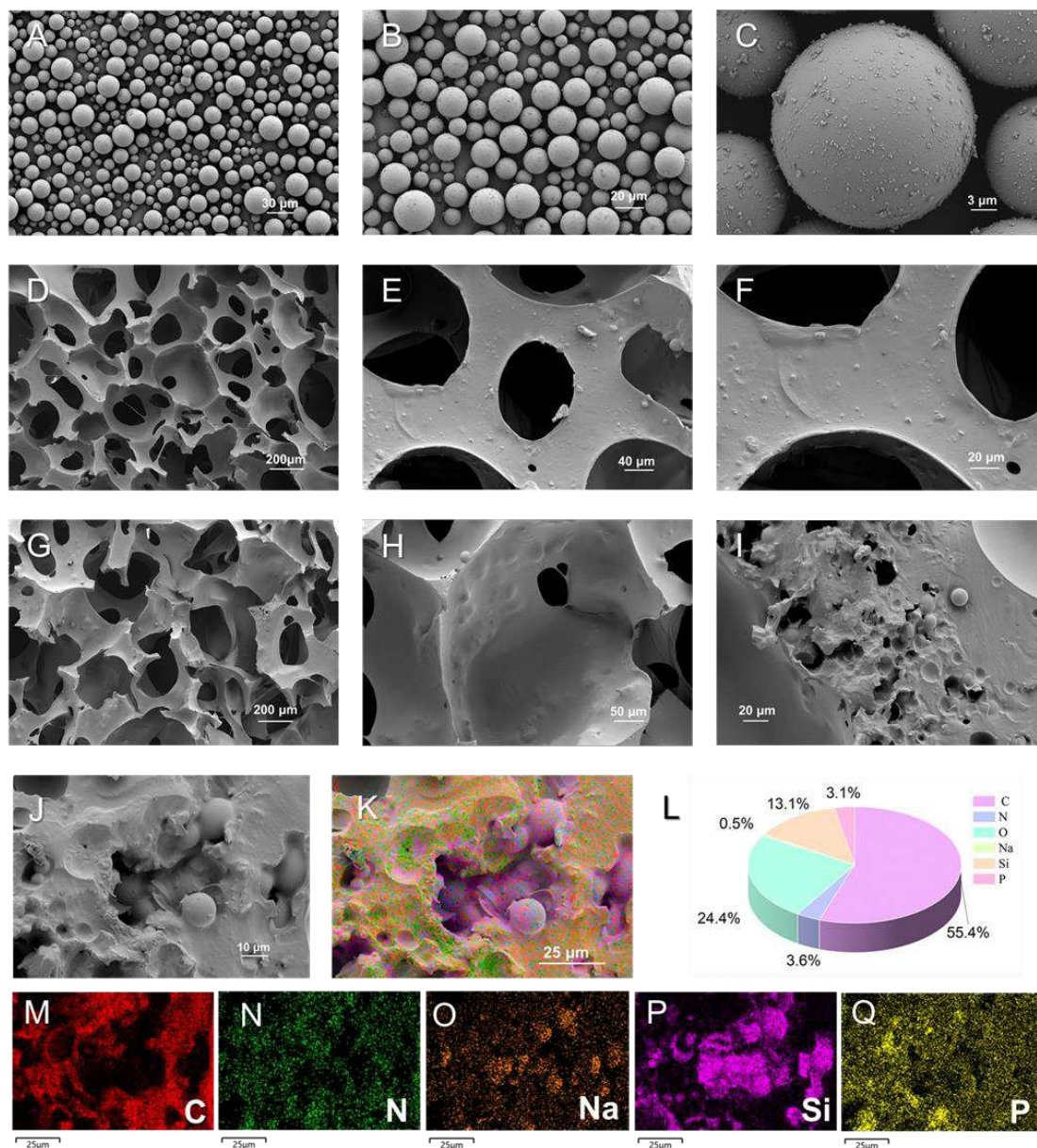
Figure. 2 (A-C) SEM images of HGM. (D-F) SEM images of pure PU foam. (G-I) SEM images of PU-FR foam. (L-Q) Elemental maps of the PU-FR.
