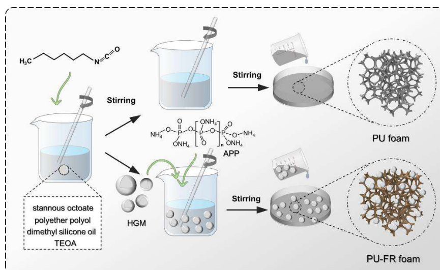
Figure. 1 Schematic illustration of the preparation process and structure of PU foam and PU-FR foam.
