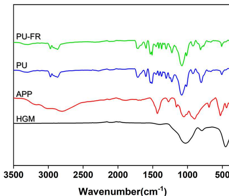
Figure. 3 Fourier transform infrared spectrum of HGM, APP, pure PU and PU-FR.
