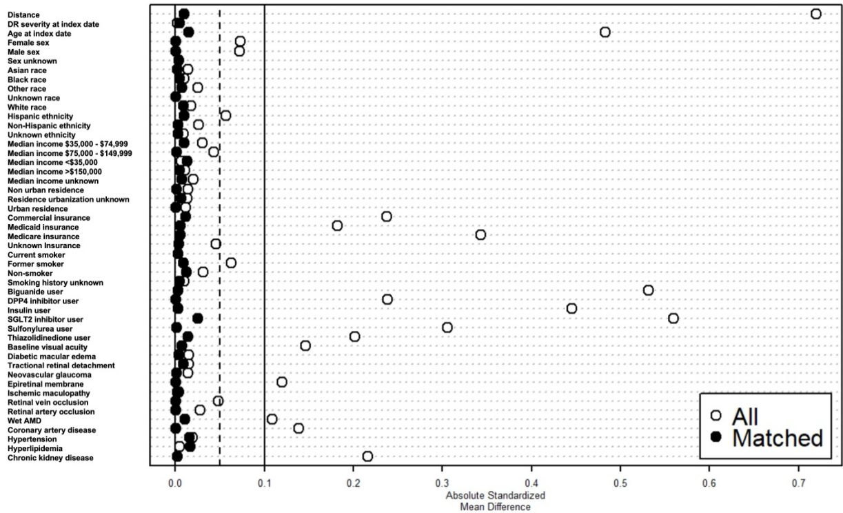
Supplementary Figure 1. Love plot showing absolute standardised mean differences for matched covariates before and after 1:1 propensity score matching.
