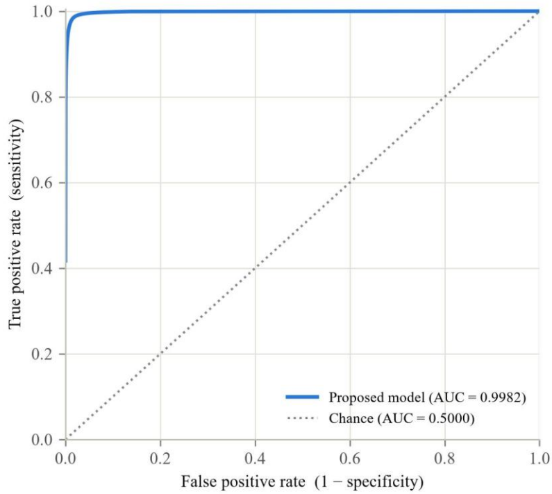
Fig. 9. Receiver operating characteristic curve for the Forged class, computed over 207,360,000 scored pixels from a fixed random subset of 1,200 test images.
