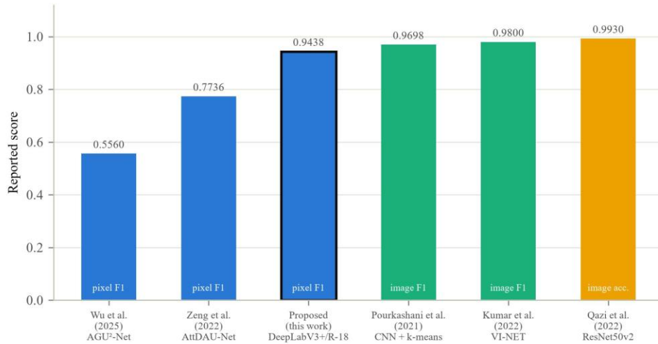
Fig. 15. The proposed model against five closely related published methods. Scores are as reported by each source and are not measured on a common test set.
