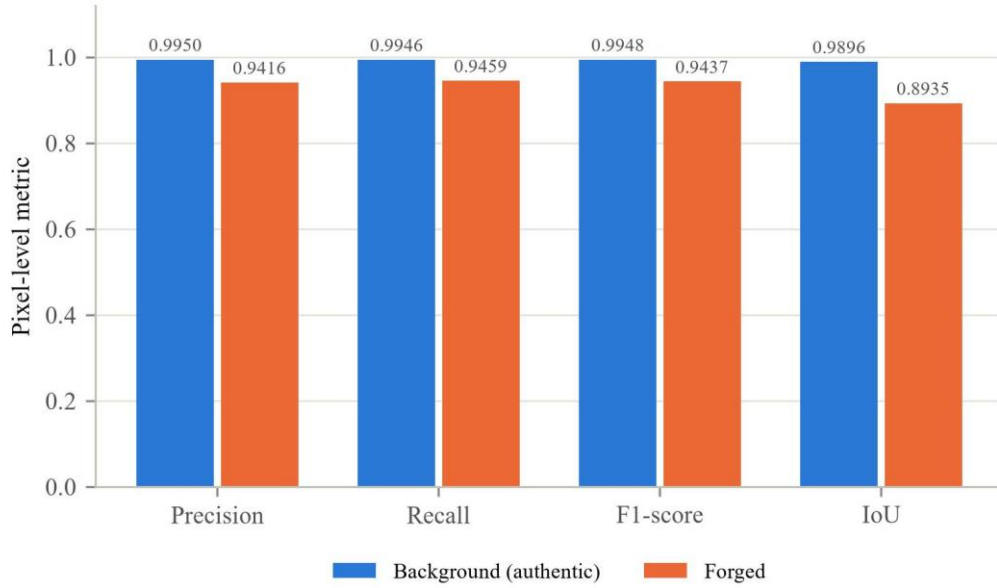
Fig. 8. Per-class pixel precision, recall, F1 and IoU of the proposed model on the held-out test split.
