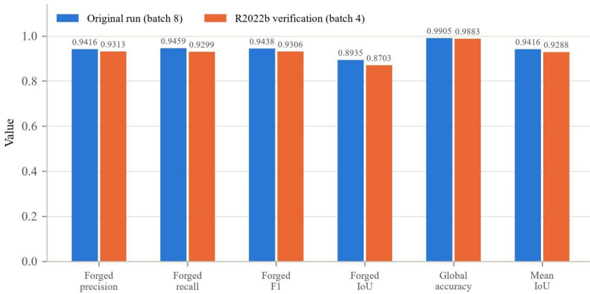
Fig. 16. Original run versus the independent R2022b re-verification, on the same held-out test split.
