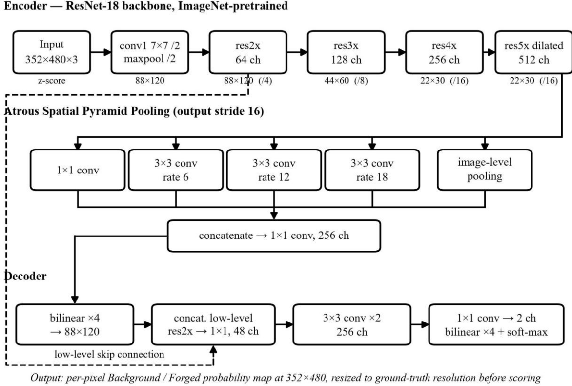
Fig. 3. Architecture of the proposed DeepLabV3+/ResNet-18 network. The encoder holds an output stride of 16 by dilating its final residual stage; the dashed connector is the low-level skip that restores boundary detail in the decoder.
