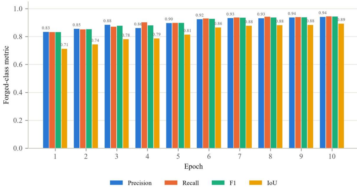
Fig. 6. Forged-class validation precision, recall, F1 and IoU after each of the ten training epochs.
