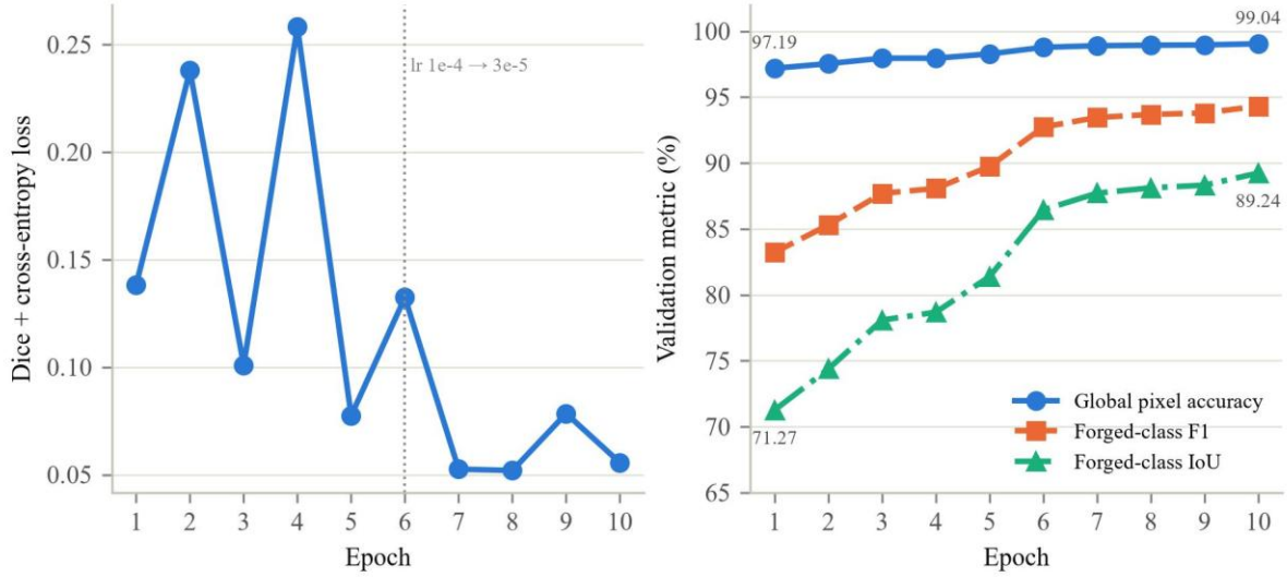
Fig. 5. Training loss and validation metrics per epoch for the proposed model. The dotted vertical line marks the learning-rate drop at epoch 6.
