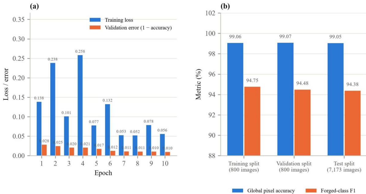
Fig. 7. (a) Training loss and validation error per epoch. (b) Global pixel accuracy and Forged-class F1 of the selected network, measured under an identical procedure on its training, validation and test splits.
