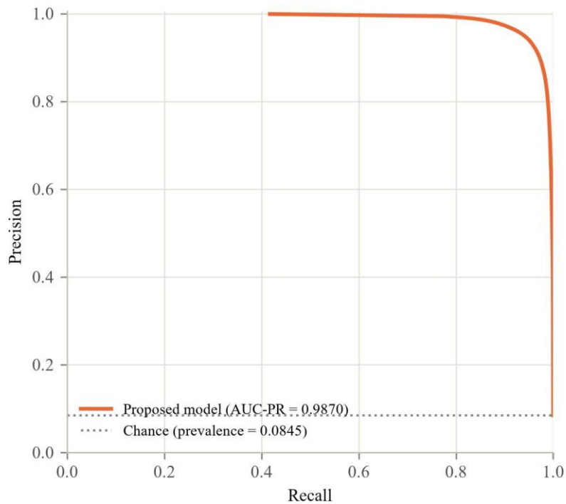
Fig. 10. Precision–recall curve for the Forged class over the same pixel population. The dotted line is the chance level, equal to the class prevalence.
