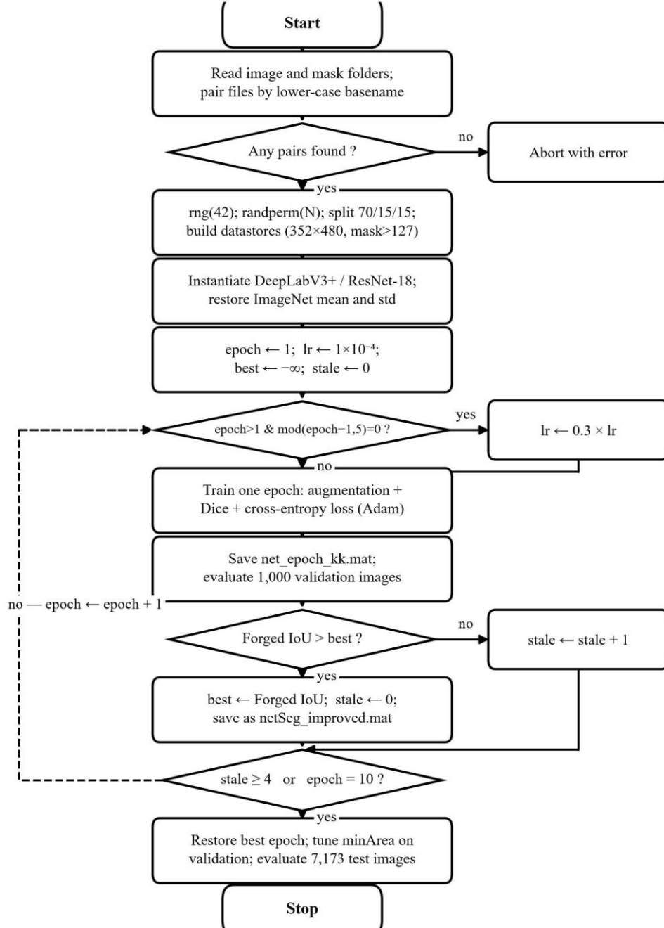
Fig. 2. Flowchart of the training and evaluation procedure. Diamonds are decision nodes; the dashed connector is the epoch loop-back; the branch nodes on the right rejoin the main spine.
