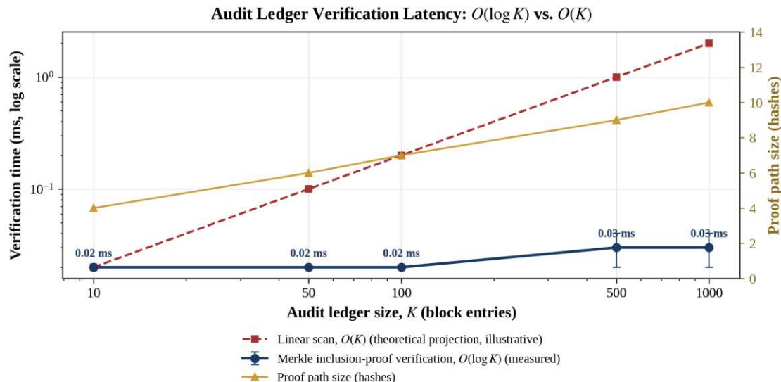
Fig. 9. Audit Ledger Merkle Proof Verification Latency O(\log K) vs Linear Scan O(K) . Demonstrates that Merkle-proof verification scales logarithmically with ledger size K , in contrast to a linear scan baseline, motivating the Merkle-tree design choice for audit-ledger inclusion checks at scale.
