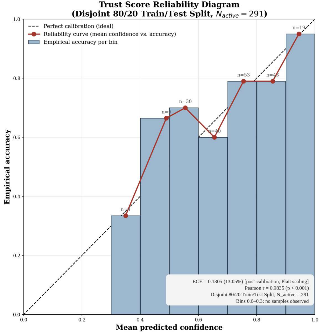
Fig. 7. Trust Score Reliability Diagram and Calibration Curve (Disjoint 80/20 Train/Test Split, N_{active} = 291 ). Plots predicted Trust Score against observed outcome frequency to verify that the Platt-calibrated score is well-calibrated on held-out data, supporting its use as a continuous input to the escalation threshold rather than an uncalibrated heuristic.
