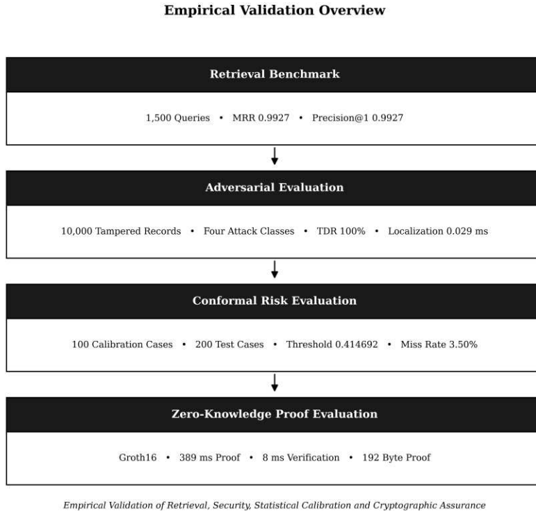
Fig. 8. Empirical Validation Overview summarizing the retrieval benchmark, adversarial evaluation, conformal risk evaluation, and zero-knowledge proof evaluation.
