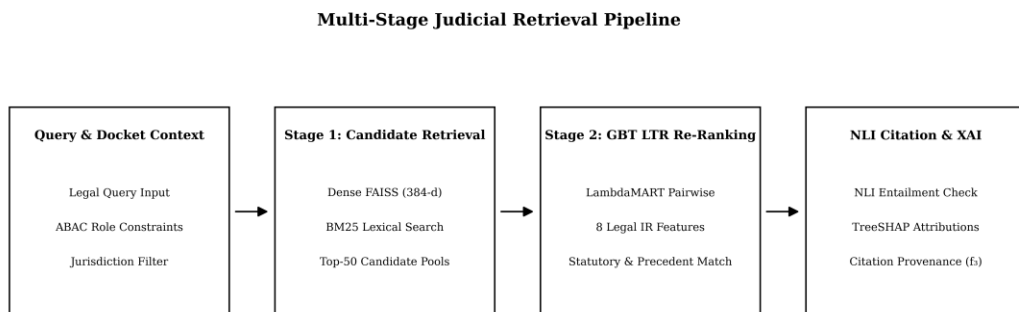
Fig. 6. Multi-Stage Judicial Retrieval Pipeline combining dense (FAISS IVF-Flat) and lexical (BM25) retrieval, candidate fusion, gradient-boosted re-ranking, TreeSHAP explainability, and NLI Citation Entailment verification.
