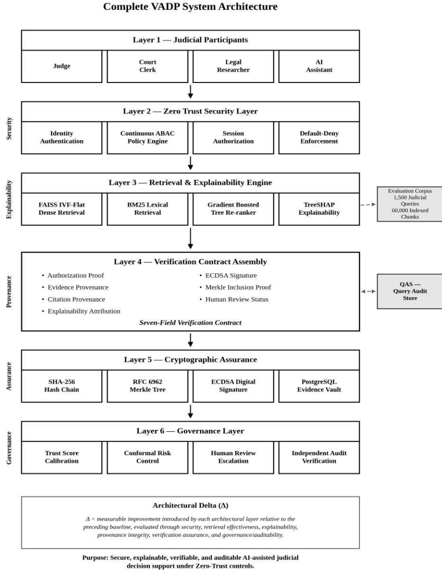
Fig. 1. Complete VADP Architecture integrating Zero-Trust authorization, multi-stage judicial retrieval, Verification Contract generation, cryptographic provenance, and governance mechanisms for independently auditable AI-assisted judicial decision support.
