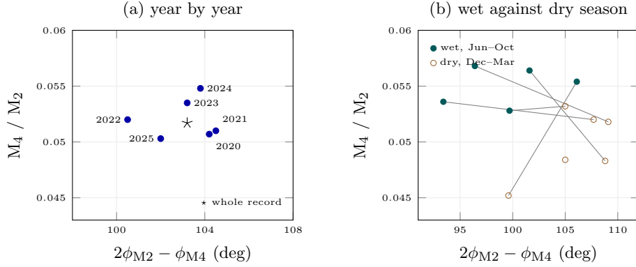
Fig. 6 Non-linear distortion in the coordinates of Friedrichs and Aubrey (1988). The horizontal axis is the relative phase of the first overtide, which is flood dominant between 0^\circ and 180^\circ , and the vertical axis is the M_4/M_2 amplitude ratio. (a) Separate harmonic fits to each complete year, with the whole-record value as a star. (b) The same fits split into wet and dry season and joined in pairs. The 2021 wet season is missing because of the 75-day outage in Fig. 2
