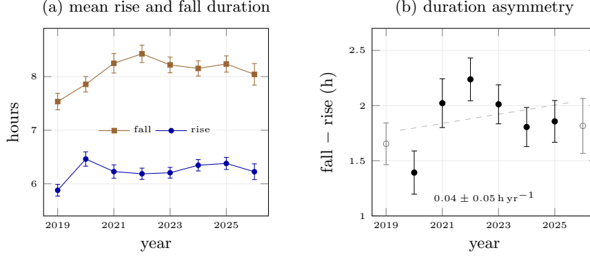
Fig. 9 Duration asymmetry through the record, from high and low waters identified directly in the hourly series. Error bars are one standard error of the mean. (a) The mean rise and fall durations for each year. (b) The difference between them, with the weighted straight line fitted to the six complete years. Open circles mark 2019 and 2026, which cover only part of a year and are excluded from the fit.
