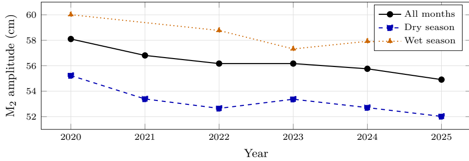
Fig. 8 Annual M_2 amplitude estimated from all months and from the dry and wet seasons separately. The three series decline at indistinguishable rates, which rules out uneven seasonal sampling as the cause
