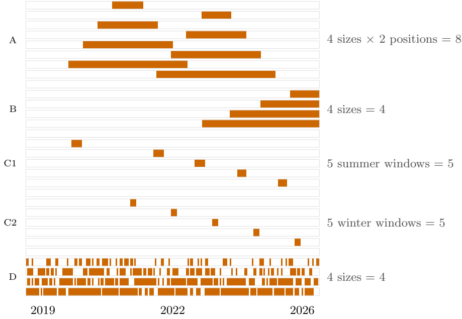
Fig. 3 The 26 withheld-data experiments. Each row is one experiment and spans the whole record from May 2019 to June 2026 and the shaded interval is the set of days withheld from the fit
