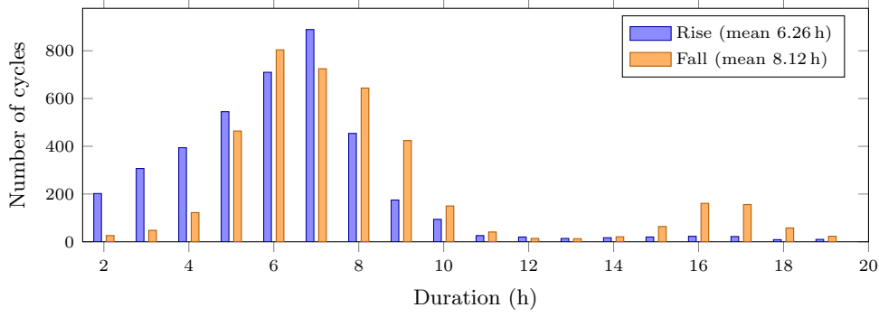
Fig. 5 Distribution of rise and fall durations over 3,931 and 3,958 tidal cycles. The two distributions overlap but the fall is systematically longer
