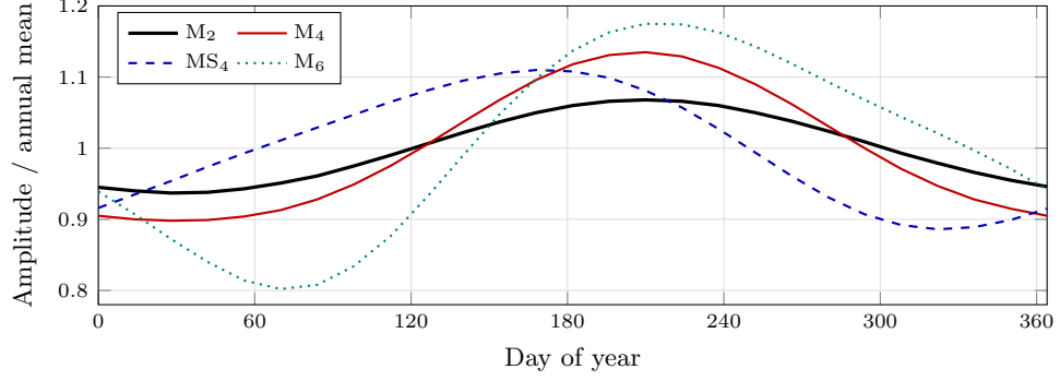
Fig. 7 Fitted annual envelopes of the amplitude of M_2 and of three shallow-water constituents, each normalised by its own annual mean. The shallow-water constituents vary two to three times more than M_2 and peak between June and August (days 150–240)
