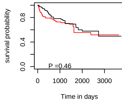
PFI hsa-mir-2355
