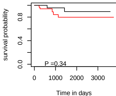
DFI hsa-mir-664a
