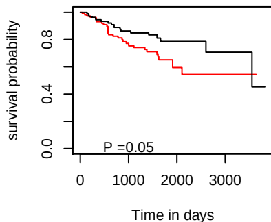
DSS hsa-mir-2277
