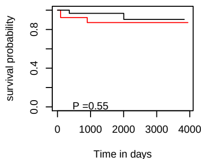
DFI hsa-mir-215
