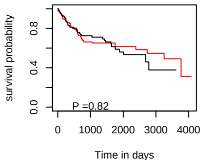
PFI hsa-mir-551b
