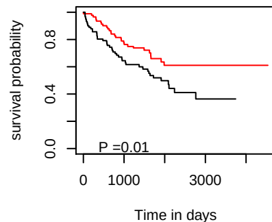
OS hsa-mir-194-1
