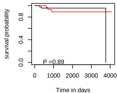
DFI hsa-mir-153-1
