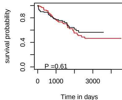
OS hsa-mir-664a
