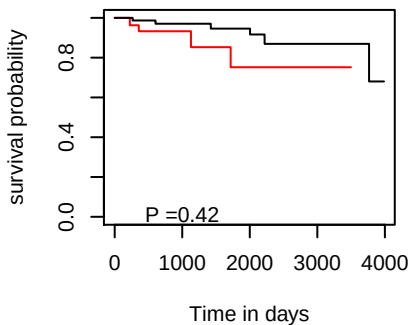
DFI hsa-mir-190b
