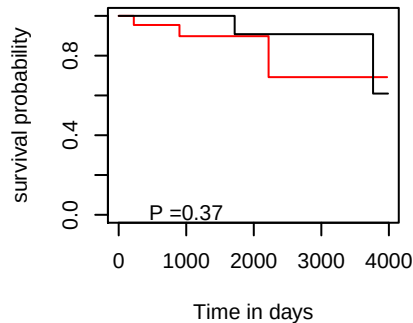
DFI hsa-mir-320b-2
