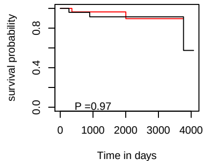
DFI hsa-mir-375
