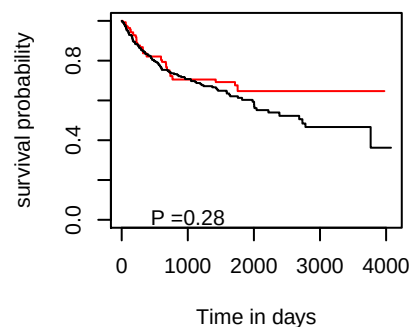
PFI hsa-mir-3131
