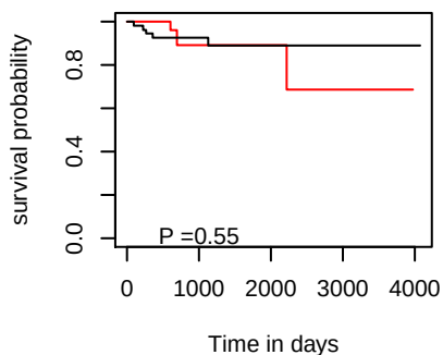
DFI hsa-mir-1537
