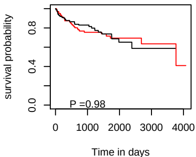
PFI hsa-mir-3130-1
