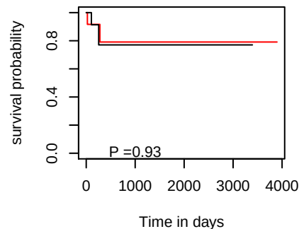
PFI hsa-mir-128-1
