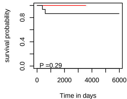
DSS hsa-mir-6808
