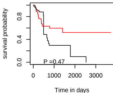
OS hsa-mir-151a
