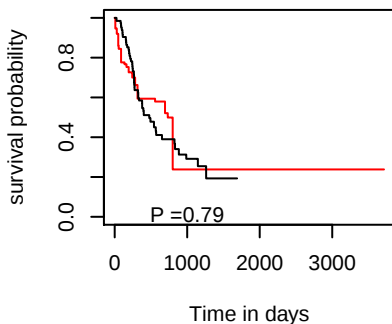
PFI hsa-mir-6502
