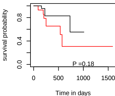
DFI hsa-mir-4786
