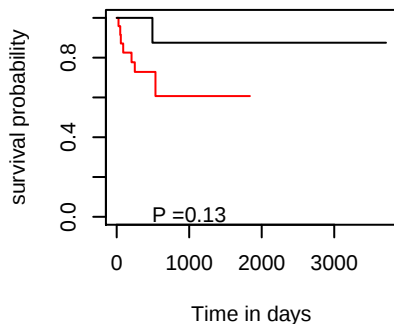
DFI hsa-mir-4662a
