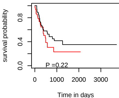
PFI hsa-mir-4491
