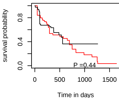
PFI hsa-mir-375
