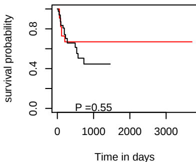
DFI hsa-mir-320c-2
