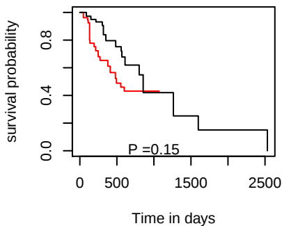
OS hsa-mir-483
