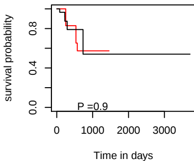
DFI hsa-mir-25
