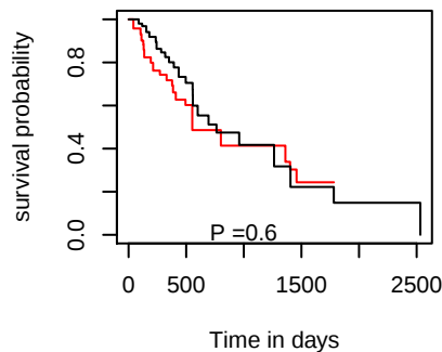
OS hsa-mir-1343
