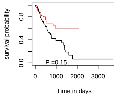
OS hsa-mir-5090
