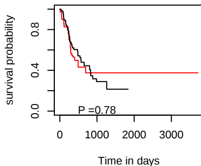
PFI hsa-mir-4645
