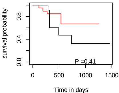
DFI hsa-mir-3648
