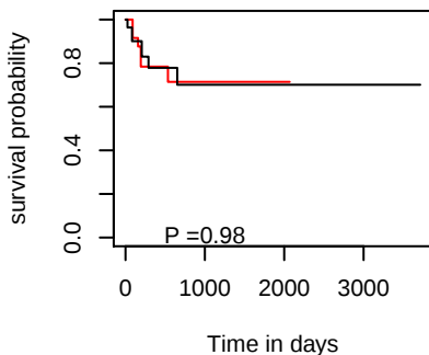
DFI hsa-mir-3940
