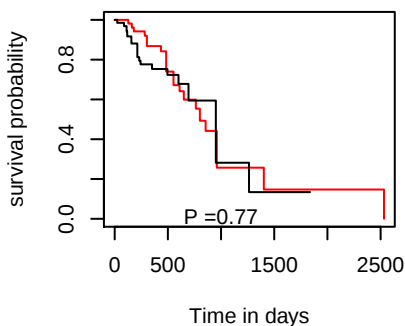
OS hsa-mir-5683
