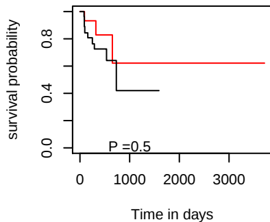
DFI hsa-mir-30d
