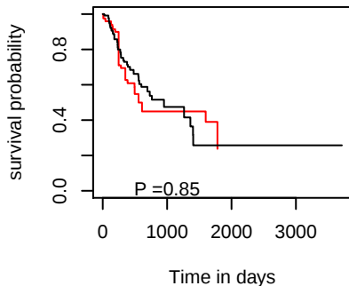
OS hsa-mir-489
