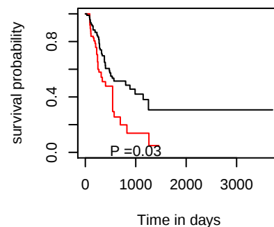
PFI hsa-mir-1284
