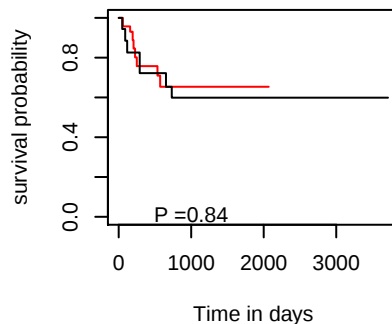
DFI hsa-mir-1305
