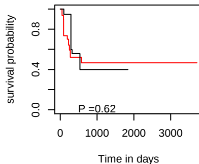
DFI hsa-mir-30c-1
