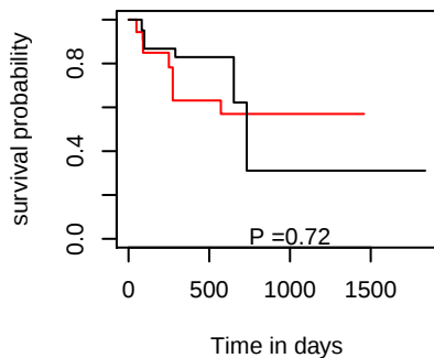
DFI hsa-mir-30e
