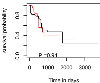
DSS hsa-mir-34a
