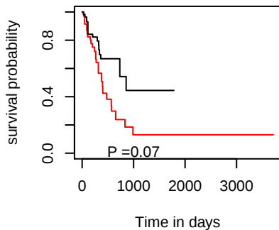
PFI hsa-mir-5010
