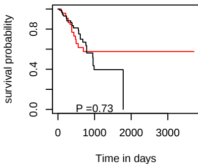
DSS hsa-mir-6852
