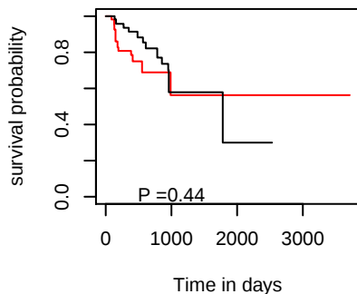
DSS hsa-mir-320c-2
