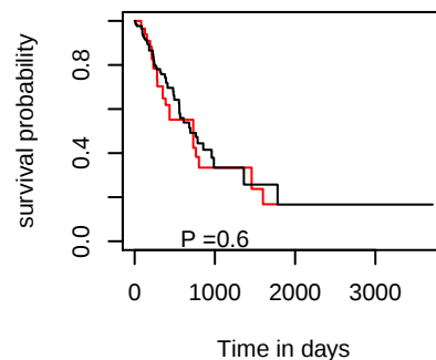
OS hsa-mir-4775
