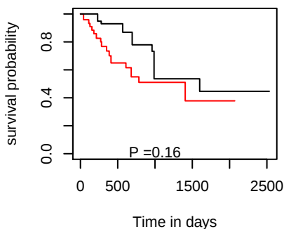
DSS hsa-mir-675
