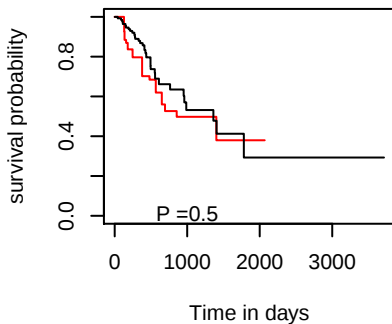
DSS hsa-mir-6513
