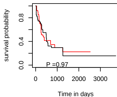
PFI hsa-mir-34a
