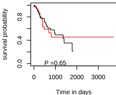
OS hsa-mir-4645
