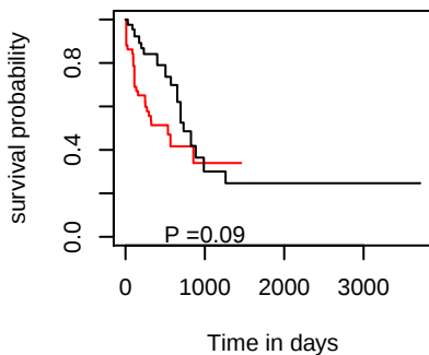
PFI hsa-mir-149
