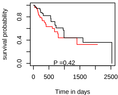
OS hsa-mir-675
