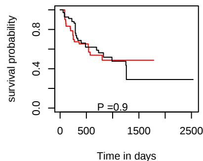
PFI hsa-mir-93
