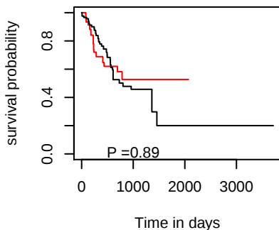
OS hsa-mir-6501
