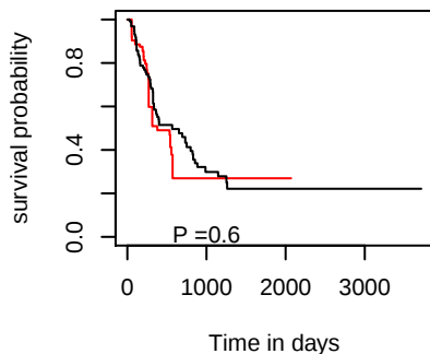
PFI hsa-mir-1305
