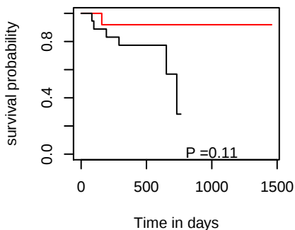
DFI hsa-mir-26b
