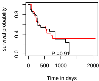
PFI hsa-mir-5001
