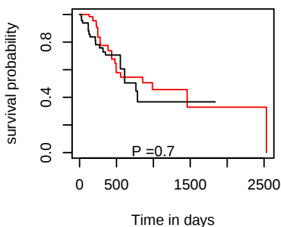
OS hsa-mir-4999
