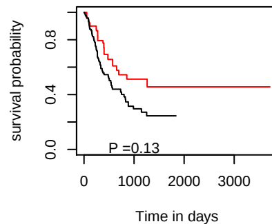
PFI hsa-mir-378f
