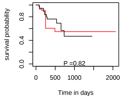
DFI hsa-mir-3176
