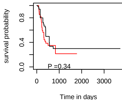
PFI hsa-mir-491
