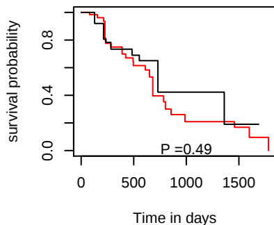
OS hsa-mir-139
