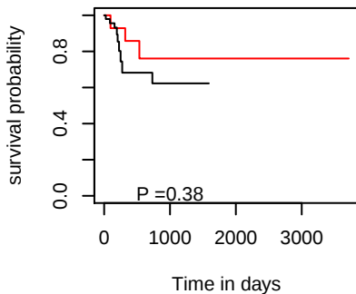
DFI hsa-mir-581
