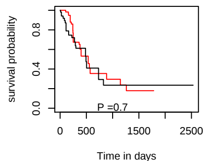
PFI hsa-mir-942
