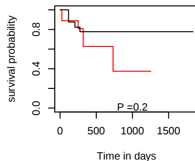
DFI hsa-mir-5683
