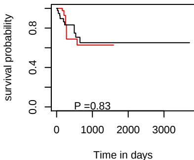
DFI hsa-mir-489
