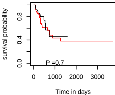
PFI hsa-mir-30d
