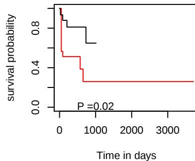
DFI hsa-mir-5010
