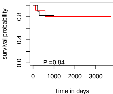
DFI hsa-mir-151a
