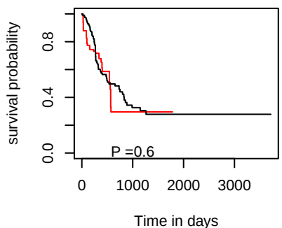
PFI hsa-mir-5687
