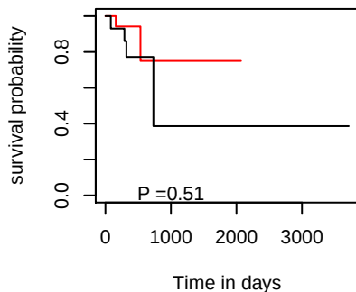
DFI hsa-mir-582
