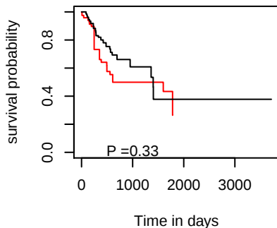
DSS hsa-mir-489
