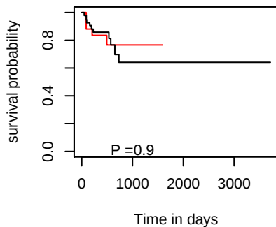
DFI hsa-mir-4777
