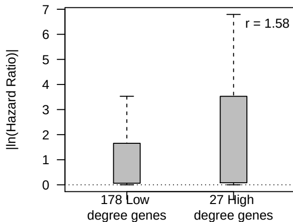
LUSC PFI
