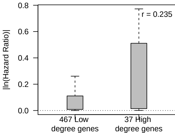
LUAD OS
