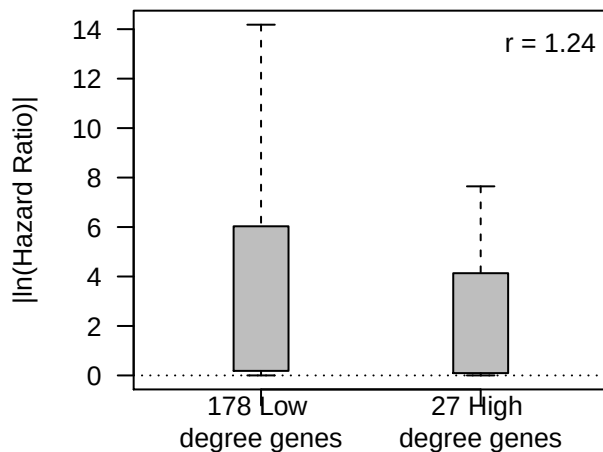
LUSC DFI
