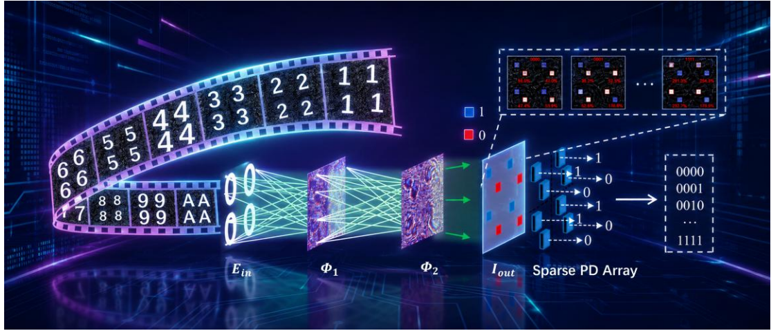
Fig. 1 Conceptual architecture of the “Light-Field-to-Bits” encoder. The system provides a direct "LFB" mapping from hexadecimal input patterns (0-F) to 4-bit binary codewords (0000-1111). The input digital information is initially encoded into the spatial amplitude of the light field ( E_{in} ). The wavefront then undergoes a cascaded diffractive modulation ( \Phi_1 and \Phi_2 ). The network deterministically routes the optical energy into specific regions of interest (ROIs) on the output detection plane ( I_{out} ). A sparse photodetector (PD) array is conceptualized to capture the focused optical distribution. The eight PDs are grouped into four differential pairs. Within each pair, the detector receiving the higher optical intensity directly dictates the output logic state of the corresponding bit.
