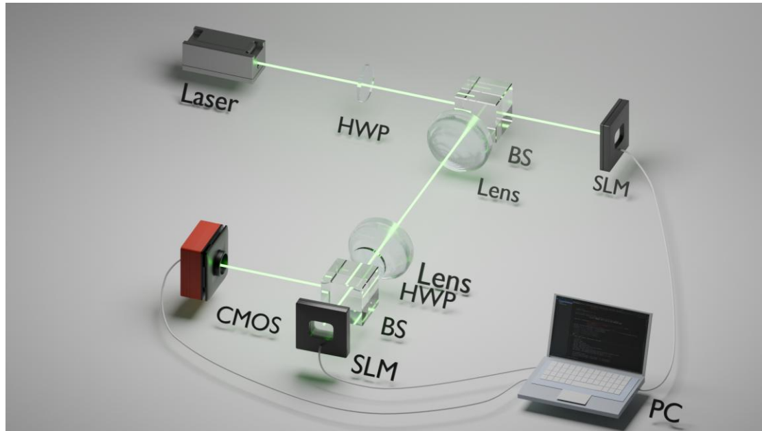
Fig. 3 Schematic of the experimental optical setup. The system employs a cascaded reflective architecture. A 532\text{ nm} wavelength laser serves as the coherent light source. The beam is expanded and polarization-tuned by a half-wave plate (HWP) before illuminating the amplitude-type SLM, which encodes the input information. An optical relay system comprising beam splitters (BS) and lenses directs the signal to the phase-type SLM, which executes the trainable phase modulation. The intermediate diffracted intensity is captured by a CMOS sensor and transferred to a PC for implementation of the secondary electronic diffractive layer. PC: Personal computer.
