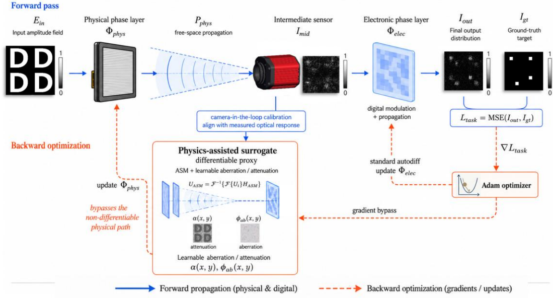
Fig. 2 In situ camera-in-the-loop optimization framework driven by a physics-assisted surrogate model. The system architecture operates through a collaborative optoelectronic loop comprising a forward propagation pass (solid blue arrows) and a backward optimization pathway (dashed orange arrows). In the forward pass, the input amplitude field ( E_{in} ) is modulated by the physical phase layer ( \Phi_{phys} ) and undergoes free-space diffractive propagation ( P_{phys} ). The intermediate intensity ( I_{mid} ) is captured by a CMOS sensor and subsequently processed by the electronic phase layer ( \Phi_{elec} ) to yield the final output distribution ( I_{out} ). During backward optimization, the task loss ( L_{task} ) is computed by evaluating the deviation between the final output distribution ( I_{out} ) and the ground-truth target ( I_{gt} ). The error gradients bypass the actual optical path and backpropagate through a differentiable physics-assisted surrogate.
