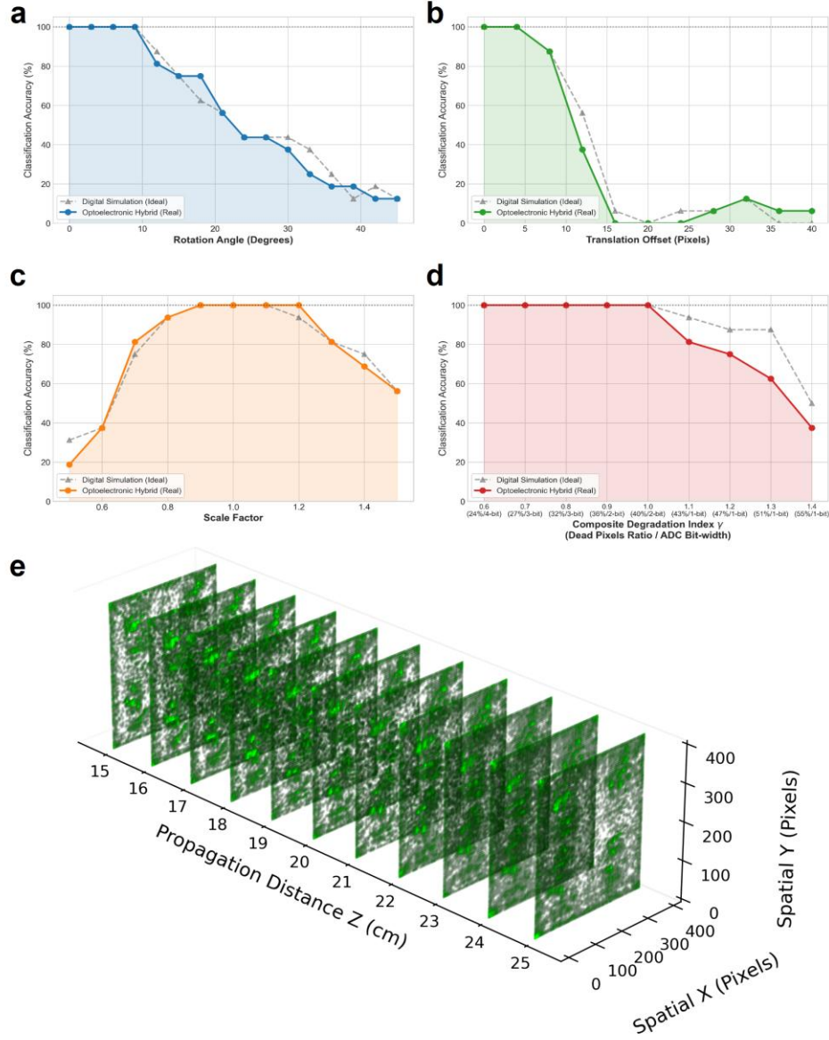
Fig. 5 Comprehensive robustness and physical tolerance evaluation of the "LFB" optoelectronic encoder. (a–c) Complete 4-bit codeword accuracy of the system under various spatial input perturbations, comparing the ideal digital simulation (dashed grey lines) with the experimental optoelectronic hybrid implementation (solid colored lines). (a) rotation, (b) translation offset, and (c) scale factors. (d) System robustness against composite optoelectronic hardware noise. The x-axis represents a composite degradation index \gamma , which pairs the CMOS dead-pixel ratio with the ADC quantization bit-width. (e) Volumetric evolution of the diffractive light field along the propagation axis.
