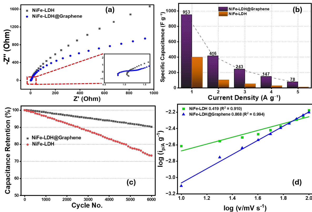
Figure 7. Electrochemical characterization of bare and graphene-coated NiFe-LDH electrodes: (a) EIS Nyquist plots showing charge-transfer and ion-diffusion behavior; (b) specific capacitance vs. current density relationship showing rate performance; (c) capacitance retention over 6,000 cycles of charging-discharging; and (d) determination of b value from the \log(i) - \log(v) plot, which indicates the importance of surface-controlled vs. diffusion-controlled charge storage mechanisms.
