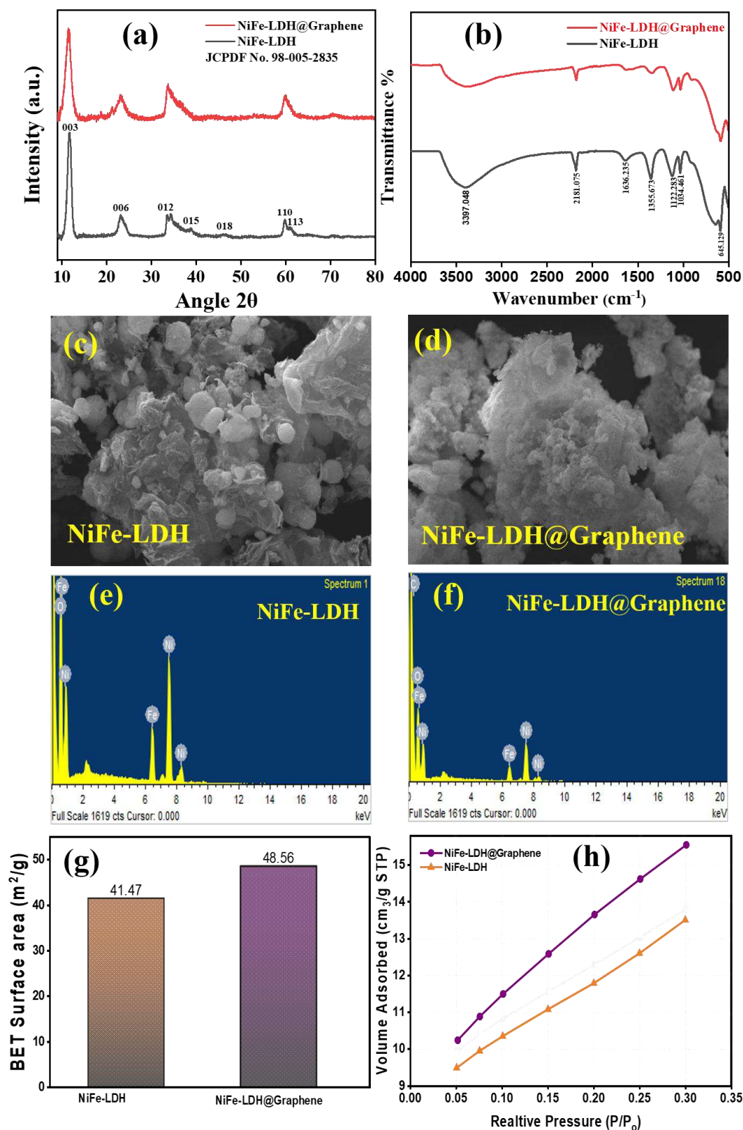
Figure 3. (a) X-ray diffraction patterns; (b) FTIR spectra; (c-d) FESEM images; (e-f) elemental mapping of Ni, Fe, O, and C elements in EDS; and (g-h) BET analysis of NiFe-LDH and NiFe-LDH@Graphene samples.
