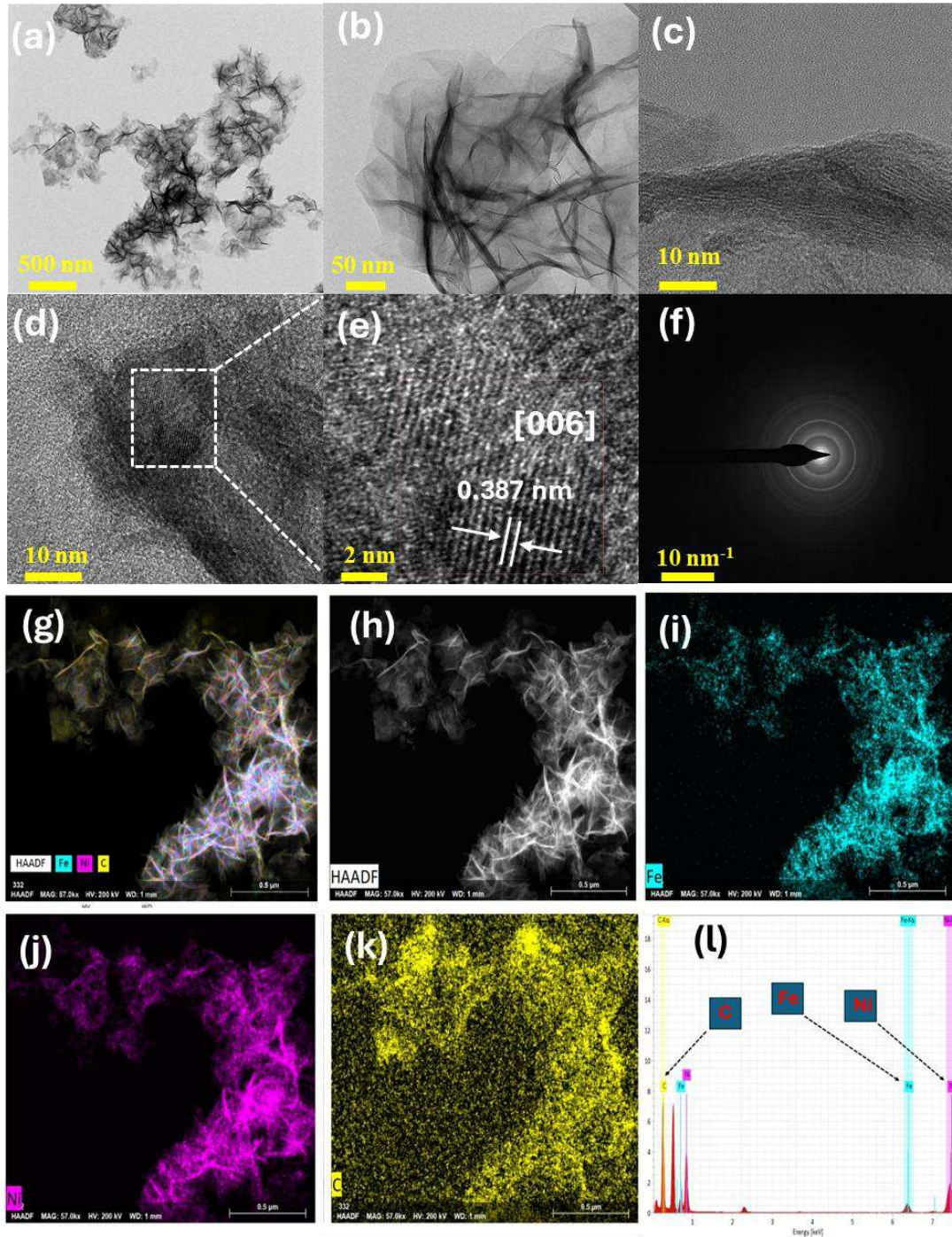
Figure 4. HRTEM analysis of the synthesized NiFe-LDH@Graphene material: (a-c) HRTEM images at various magnifications displaying the ultrathin, wrinkled, and sheet-like layered morphology; (d,e) enlarged HRTEM
