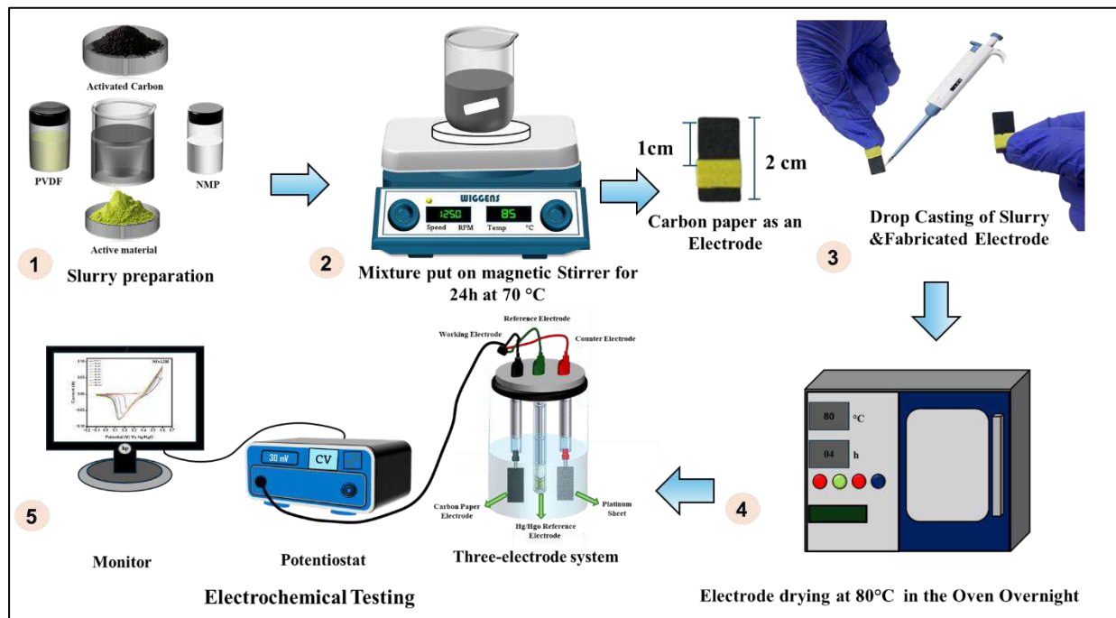
Figure 2. Schematic depicting the step-by-step process of slurry to electrode fabrication.
