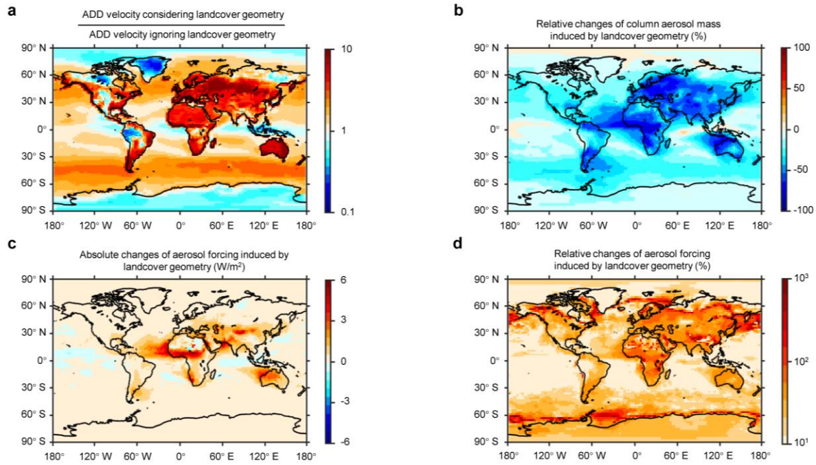
Fig. 4| Multiple influence of landcover geometry. a , Influence of landcover geometry on global ADD velocity. b , Relative changes of global column aerosol mass induced by landcover geometry (%). c , Absolute changes of global aerosol forcing induced by landcover geometry ( W/m^2 ). d , Relative changes of global aerosol forcing induced by landcover geometry (%).
