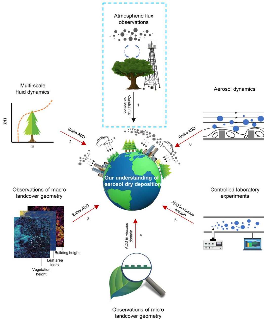
Fig. 3| Different paths to understand ADD in the new ADD framework. According to the new framework, progresses in understanding ADD comes from six paths: advances in atmospheric flux observations, multi-scale fluid dynamics, observations of macro landcover geometry, observations of micro landcover geometry, controlled laboratory deposition experiments, and aerosol dynamics. In contrast, progresses in understanding ADD can only come from the advance in atmospheric flux observations under current paradigm supported by the resistance model (the blue box).
