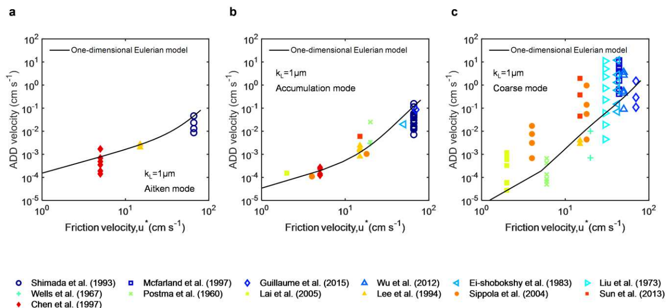
Extended Data Fig. 4| The dependence of ADD velocity on friction velocity. a, For Aitken mode. b, For accumulation mode. c, For coarse mode. Different symbols indicate observed ADD velocity over a smooth surface from published controlled laboratory studies over the past half century. These experiments were mainly conducted in ducts made of metal or glass, whose micro roughness typically ranges from 0.5 to 5 \mu\text{m} according to reported measurements for these materials (Methods). The black lines show predicted ADD velocity by the one dimensional Eulerian ADD model. The wall micro roughness ( k_L ) is set to 1 \mu\text{m} for all simulations. Aerosol diameter is set to 0.05, 0.5, and 5 \mu\text{m} for Aitken, accumulation, and coarse modes for corresponding simulations.
