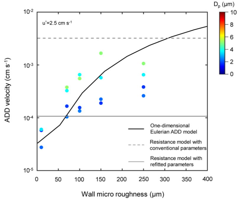
Extended Data Fig. 2| The dependence of ADD velocity on landcover micro roughness. The colorful dots are observed ADD velocity in a chamber deposition experiment. Chamber walls adhered with different sandpaper are used to model canopy-free landcover with different micro roughness. In the experiment, aerosols ranging from 1 to 5 \mu\text{m} are selected and friction velocity ( u^* ) is set to \sim 2.5 \text{ cm s}^{-1} . The black line shows predicted ADD velocity through the one dimensional Eulerian ADD model while grey line and dashed line show modeled ADD velocity through the resistance model with refitted and conventional parameters. Aerosol diameter ( D_p ) is set to 3 \mu\text{m} for all simulations.
