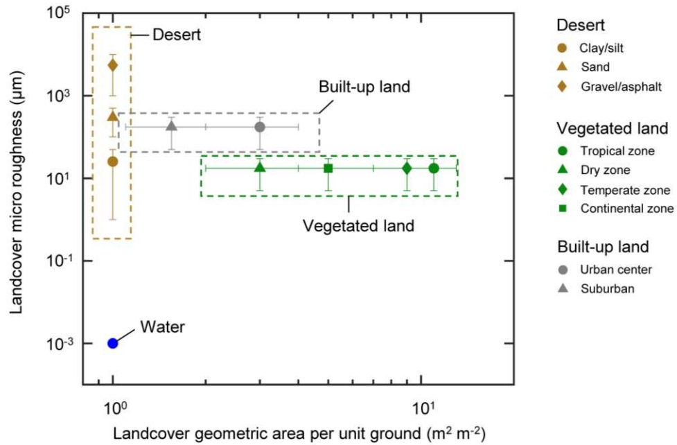
Extended Data Fig. 1| The geometric characterization for different landcover types. The blue, brown, grey, and green marks represent water, desert, built-up land and vegetated land respectively. Built-up land only considers buildings. In a geometric view, substantial differences exist both between and within these landcover types.
