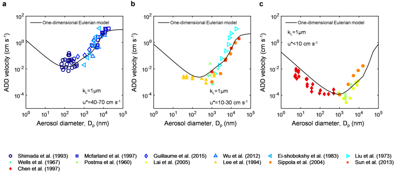
Extended Data Fig. 3| The dependence of ADD velocity on aerosol diameter. a , Under strong turbulence condition ( u^* = 40\text{--}70 \text{ cm s}^{-1} ). b , Under moderate turbulence condition ( u^* = 10\text{--}30 \text{ cm s}^{-1} ). c , Under weak turbulence condition ( u^* < 10 \text{ cm s}^{-1} ). Different symbols indicate observed ADD velocity over a smooth surface from published controlled laboratory studies over the past half century. These experiments were mainly conducted in ducts made of metal or glass, whose micro roughness typically ranges from 0.5 to 5 \mu\text{m} according to reported measurements for these materials (Methods). The black lines show predicted ADD velocity by the one dimensional Eulerian ADD model. The wall micro roughness ( k_L ) is set to 1 \mu\text{m} for all simulations. u^* is set to 50, 20, and 5 \text{cm s}^{-1} for strong, moderate, and weak turbulence conditions for corresponding simulations.
