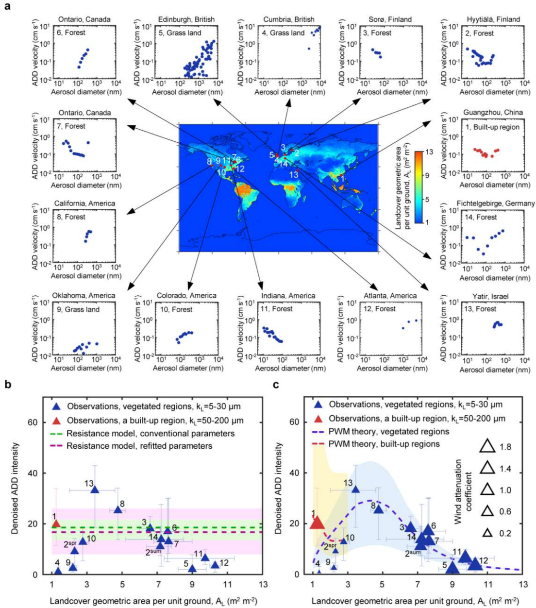
Fig. 1| The relationship between ADD and landcover geometry. a , Global observations of ADD velocities. Our measurements over a built-up region are presented in panel 1 as red circles, while published measurements over different vegetated regions are presented in rest panels as blue circles. b , The observed and resistance-model-predicted relationships between denoised ADD intensity and landcover geometry. A_L is calculated based on five remote sensing data sets and ground observations (Methods). The red triangle refers to the observed denoised ADD intensity of the built-up region and the blue triangles refer to the observed denoised ADD intensity of different vegetated regions. The vertical error bars of triangles reflect variation of observed ADD velocity in a . The horizontal error bars of triangles refer to A_L uncertainty caused by different data sets used
