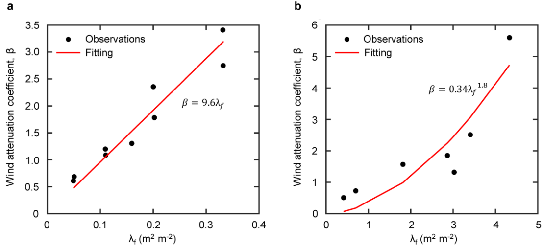
Extended Data Fig. 6| The relationship between wind attenuation coefficient and landcover geometric area per unit ground. a, For built-up land. b, For vegetated land. Observed wind attenuation coefficient \beta is calculated from measured wind profiles in wind tunnel experiments ( a ) and real forests ( b ). \lambda_f refers to landcover front area per unit ground, which equals 2 \cdot A_v / \pi and 2 \cdot A_b / \pi for vegetated land and built-up land respectively (Supplementary, section 2).
