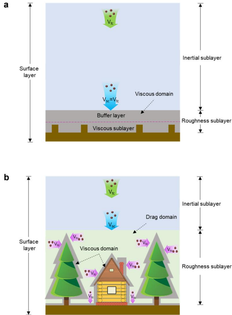
Extended Data Fig. 8| Illustration of V_{fc} , V_{sc} , and V_{tc} . a , Situation for canopy-free landcover.
