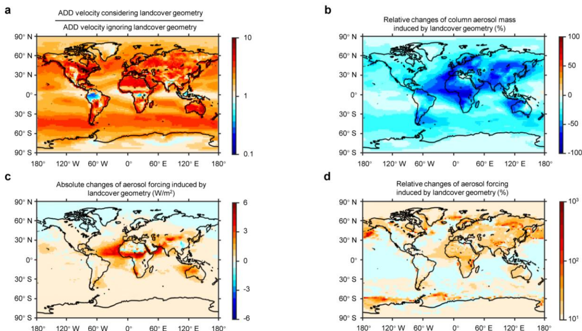
Extended Data Fig. 7| Multiple Influences of landcover geometry calculated based on the resistance model configured with refitted parameters. a , Influence of landcover geometry on global ADD velocity. b , Relative changes of global column aerosol mass induced by landcover geometry (%). c , Absolute changes of global aerosol forcing induced by landcover geometry ( \text{W/m}^2 ). d , Relative changes of global aerosol forcing induced by landcover geometry (%). These results are obtained by comparing the scenario considering landcover geometry predicted by PWM theory with the scenario ignoring landcover geometry predicted by the resistance model configured with refitted parameters. According to this calculation method, terrestrial aerosol cooling effect is reduced by 38%. Only the optimal estimation of multiple impacts of landcover geometry are presented here. The optimal estimation means input landcover geometry parameters meet: (1) values of A_L are taken as averages of results calculated from different remote sensing data sets; (2) values of k_L for ground, vegetations or buildings are taken as the optimal values that generate modeled ADD velocity agreeing best with observations within the measured k_L range of corresponding materials.
