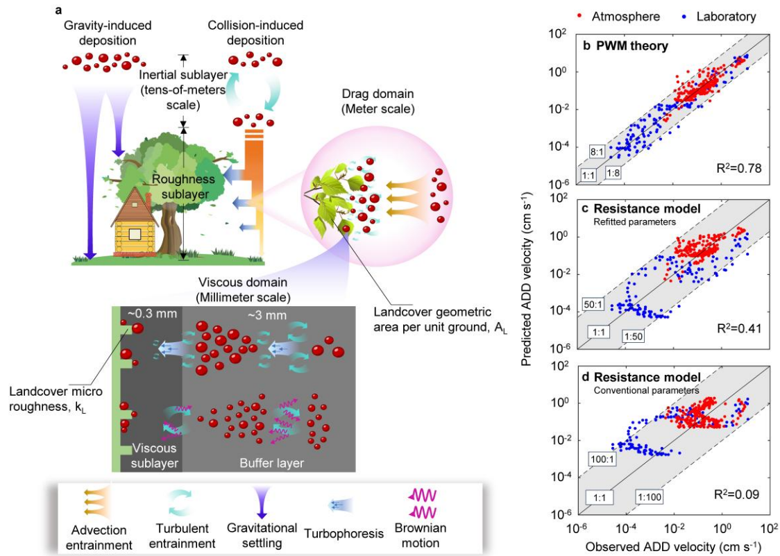
Fig. 2| Illustration and performance of the new ADD physical framework. a , Phase-wise migration of aerosols during dry deposition. The whole ADD includes aerosol migrations in inertial sublayer, drag domain (if canopies exist), and viscous domain. Aerosol migrations are driven by gravitational settling, air entrainment (turbulence & advection), Brownian motion, and turbophoresis. Macro landcover geometry (mainly referring to A_L ) influences aerosol migrations in drag domain and viscous domain by modulating atmospheric motion and the number of aerosol trapping sites within canopy, while micro landcover geometry (i.e., k_L ) affects the aerosol migration in viscous domain by changing positions of aerosol trapping sites. b , Comparison between ADD velocity from observations and the new ADD framework. c , Comparison between ADD velocity from observations and the resistance model with refitted parameters. d , Comparison between ADD velocity from observations and the resistance model with conventional parameters. Red and blue dots in b , c and d indicate observations from atmospheric flux measurements and controlled laboratory deposition experiments respectively. The grey shaded area covers 95% points.
