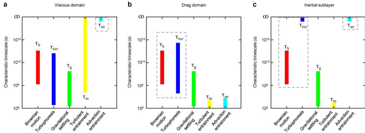
Extended Data Fig. 5| The scale analysis of aerosol motion. a , In viscous domain. b , In drag domain. c , In inertial sublayer. \tau_{ae} , \tau_{te} , \tau_b , \tau_g , and \tau_{tur} are defined as the time required for the corresponding mechanisms (advection entrainment, turbulent entrainment, Brownian motion, gravitational settling and turbophoresis) to drive aerosols to move one meter. The larger the time scale, the less important the corresponding mechanism. Grey boxes show ignored mechanisms in reconstructing ADD physical framework.
