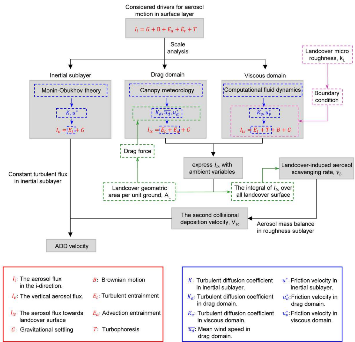
Extended Data Fig. 9| The outline of the derivation of ADD velocity. Red symbols highlight the role of aerosol dynamics. Blue symbols and boxes highlight the role of multi-scale fluid dynamics. Green and pink boxes highlight the role of landcover geometry. See mathematic details in Supplementary.
