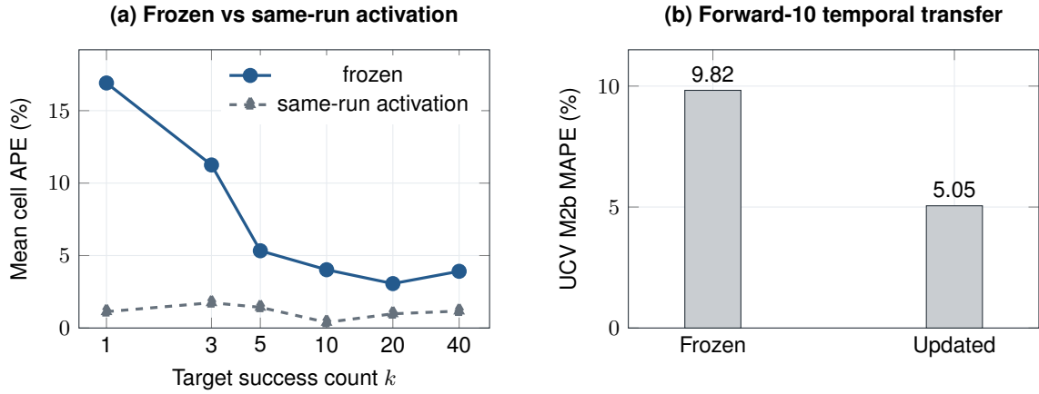
Fig. 4 UCV post-hoc activation and temporal diagnostics. (a) Frozen U-M2b mean cell APE by target success count versus the leakage-assisted, non-deployable same-run realized-activation diagnostic. (b) The separate Forward-10 later-block temporal-transfer diagnostic, shown as frozen and updated UCV M2b MAPE. Both panels are explanatory sensitivity analyses, not corrected prospective performance, a causal decomposition, or a deployable refresh policy.
