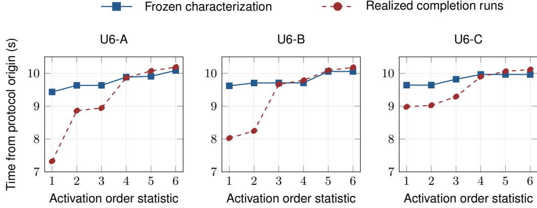
Fig. 3 Frozen versus realized UCV activation-order profiles. Each panel compares the mean within-vector activation order statistics from frozen characterization with those from accepted completion runs for one cyclic \{3, 2, 1\} placement. Times use the existing protocol origin. The largest discrepancy appears in the early order statistics. This is post-hoc state-distribution evidence, not prospective validation, causal attribution, or a deployable refresh rule.
