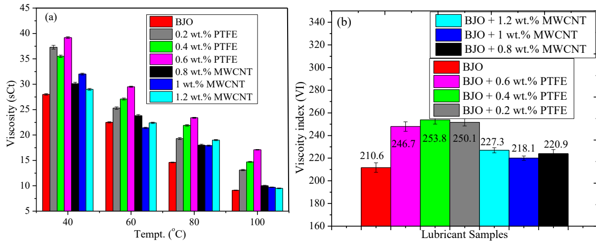
Fig. 5. Analysis of (a) viscosity against temperatures and (b) viscosity index as used in the study
