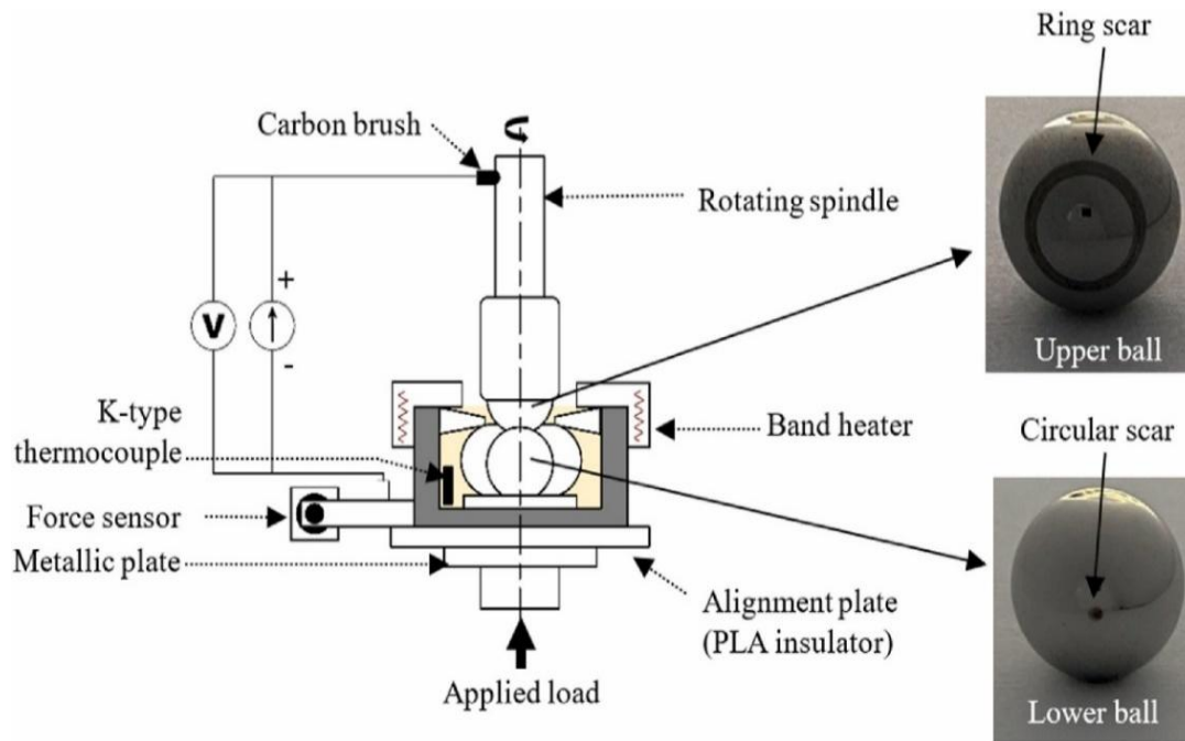
Fig. 1. Presentation of four-ball test set-up and snapshots of the upper and lower balls.
