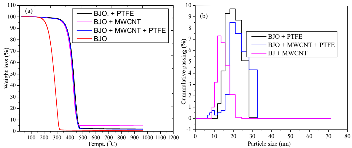
Fig. 4. (a) TGA and (b) dynamic light scattering of the samples used.
