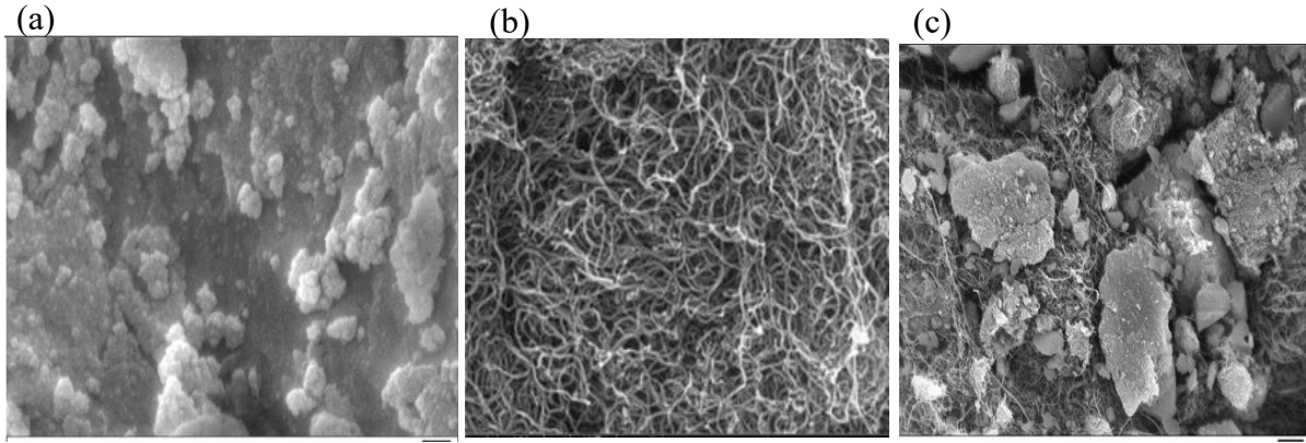
Fig. 2: FESEM images of nano additives of (a) PTFE, (b) MWCNT and (c) MWCNT/PTFE
