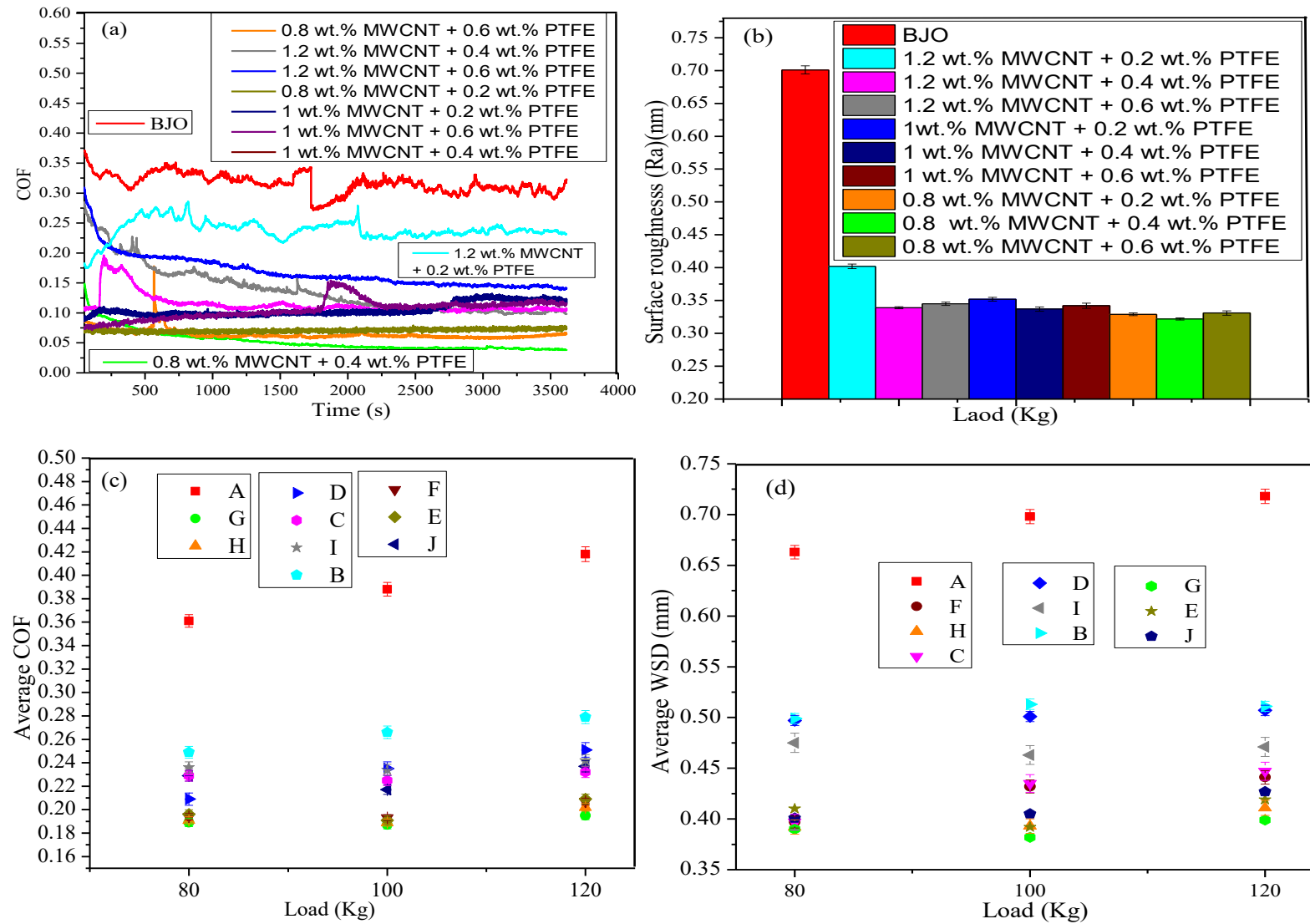
Fig. 7. (a) Coefficient of friction, (b) surface roughness (Ra), average COF and average WSD from the various blended concentrations additives under different loads; 80 Kg, 100 kg and 120 Kg, and temperature of 80°C
