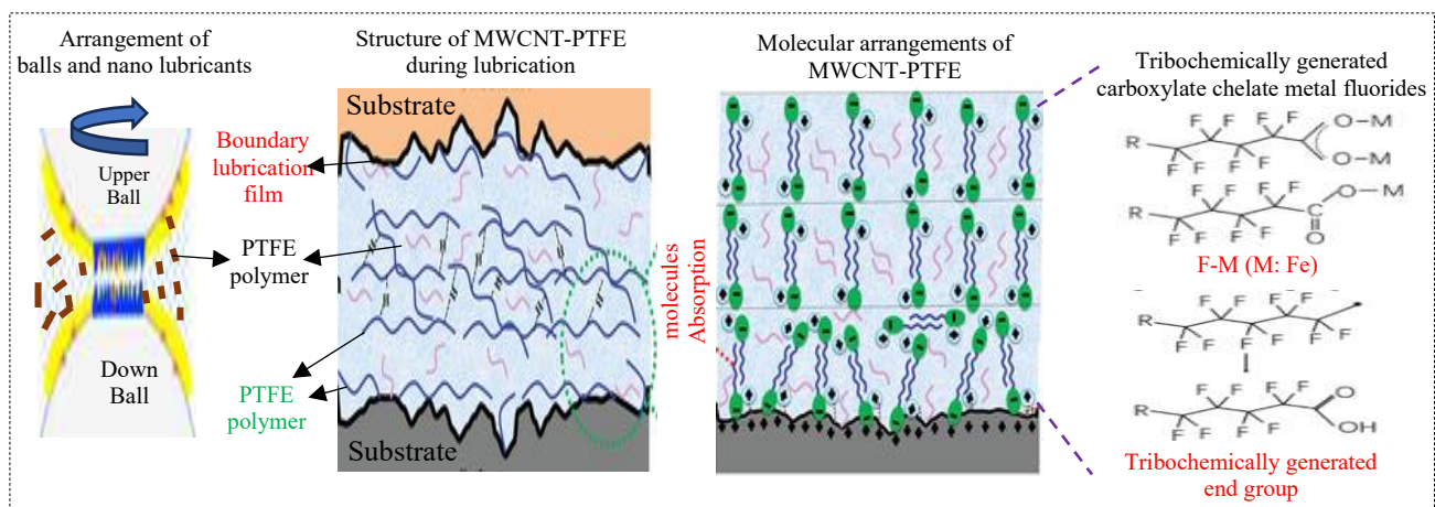
Fig. 10: Model mechanisms and tribo-film reactions towards tribo-pair wear shields for MWCNT/PTFE lubrication.
