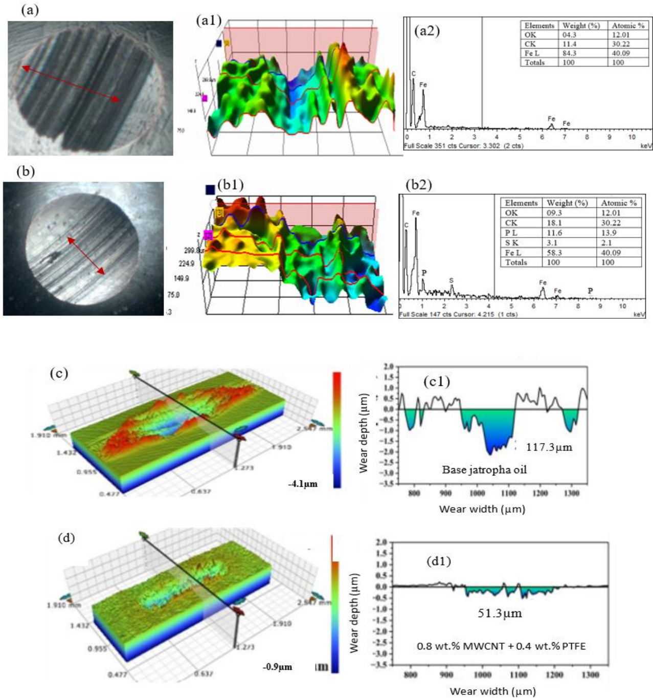
Fig. 9: (a and b) SEM, 3D image showing the Ra and the corresponding EDS; (c and d) 3D images showing wear scar and the corresponding wear depth under different working operations.
