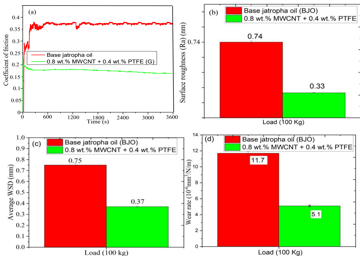
Fig. 8. (a) Coefficient of friction; (b) surface roughness (Ra); (c) average WSD and (d) wear rate from the optimized additives 0.8 wt.% MWCNT + 0.4 wt.% PTFE compared to BJO (Under 100 kg, 75 °C, 1500 rpm)
