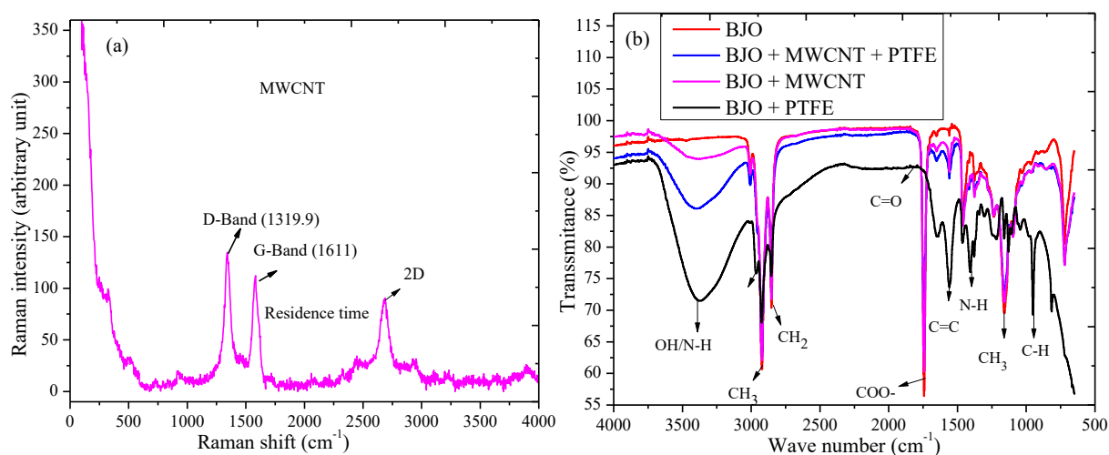
Fig. 3. (a) Raman spectroscopy of MWCNT and (b) FT-IR of the various samples.
