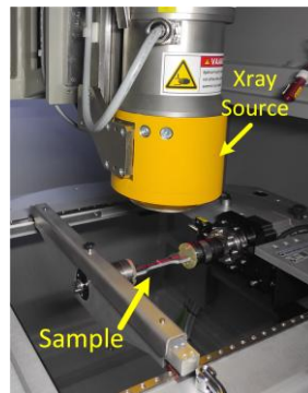
Fig. 5: Setup for XCT, showing the X-ray source and the mounted sample during scanning.
