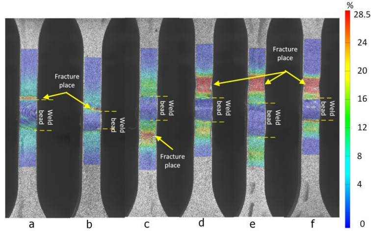
Fig. 20: DIC strain maps before fracture for the welded samples: a) W6N, b) W6R, c) W5N, d) W5R, e) W4N, and f) W4R.
