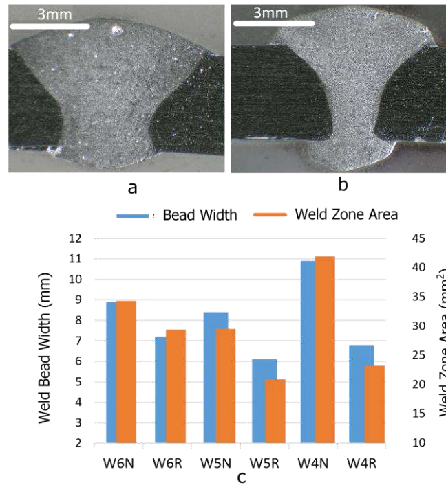
Fig. 7: Weld geometry and macrostructural characteristics of samples a) W5N and b) W5R, along with c) a comparison of weld bead width and weld zone area for all samples.
