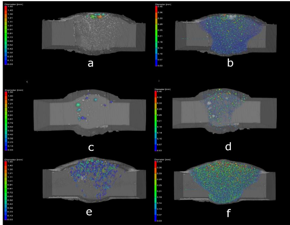
Fig. 19: XCT visualization of internal cavities in W6N, W6R, and W4N. Cavities larger than 0.4 mm in: a) W6N, c) W6R, and e) W4N. Porosities and cavities smaller than 0.4 mm in b) W6N, d) W6R, and f) W4N.
