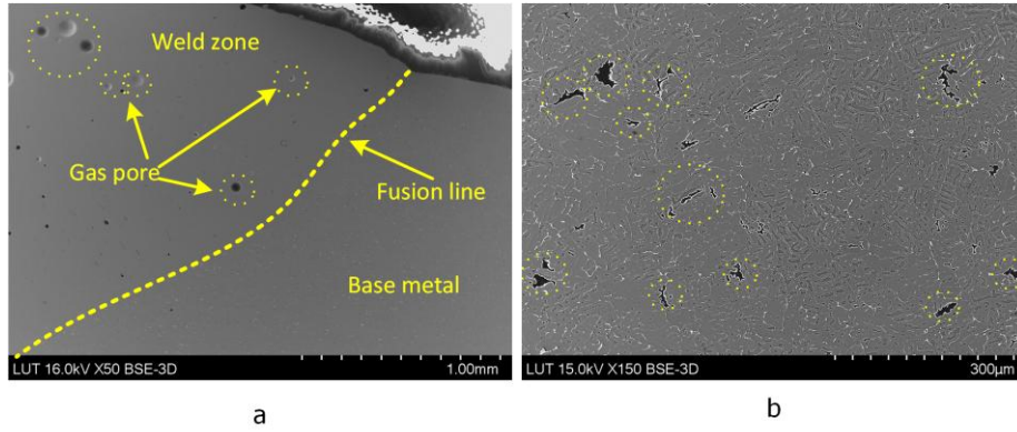
Fig. 10: SEM images of internal cavities observed in the weld region of sample W4N: a) spherical gas pores and b) irregular shrinkage cavities formed during solidification.
