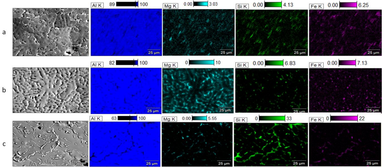
Fig. 15: SEM images and corresponding EDS elemental maps showing the distributions of Al, Mg, Si, and Fe in the weld metal of a) W6N, b) W5N, and c) W4N.
