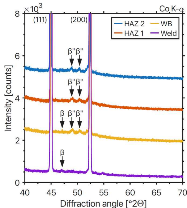
Fig. 22: XRD patterns of the weld metal, weld boundary, HAZ 1 , and HAZ 2 regions in W6N, recorded in the 2\theta range of 40–70°.
