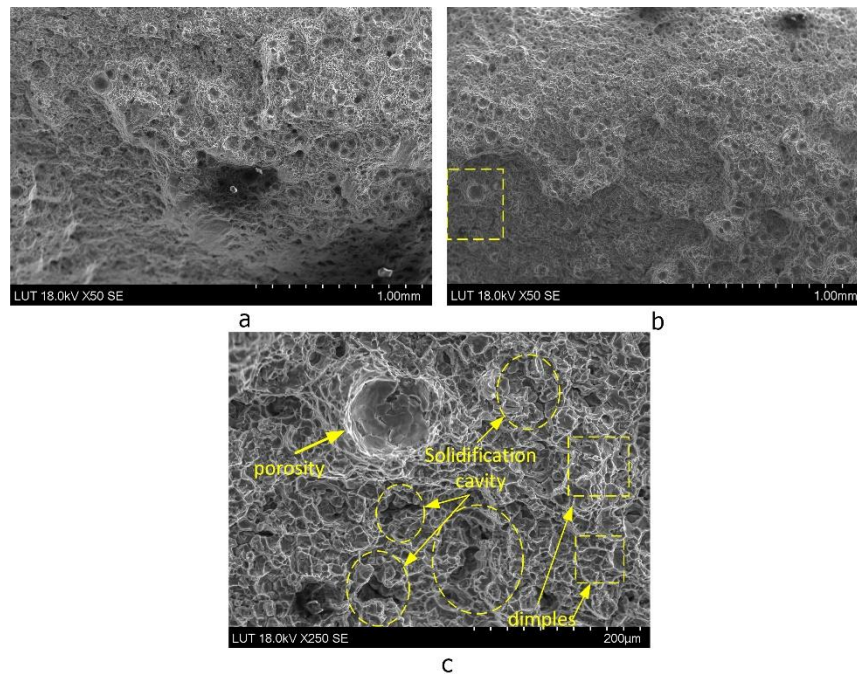
Fig. 23: SEM images of fracture surface observations of the samples a) W6N, b) W6R, and c) a higher-magnification image of the marked region in 23b.
