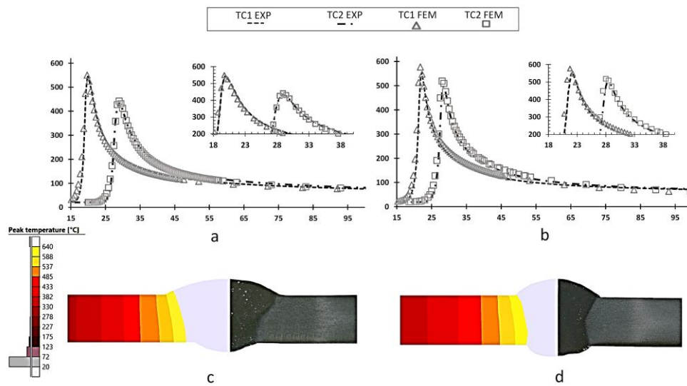
Fig. 6: Comparison of the experimental and FEM-predicted thermal cycle for samples a) W6N, b) W6R, and isothermal contour for samples c) W6N, and d) W6R.
