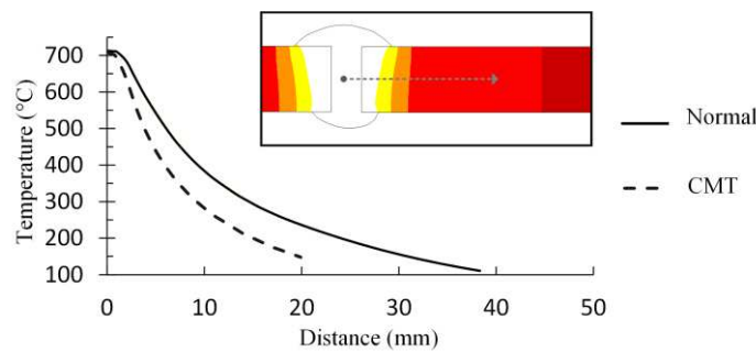
Fig. 8: FEM temperature profiles from the weld bead center to the base metal for samples W6N and W6R.
