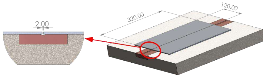
Fig. 1: Schematic illustration of the joint design, groove geometry, and specimen dimensions.
