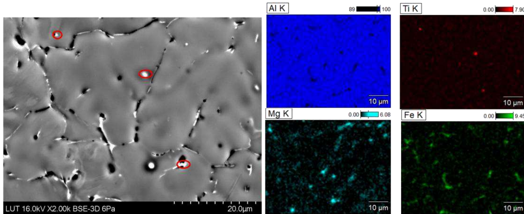
Fig. 13: SEM image and corresponding EDS elemental maps of Al, Ti, Mg, and Fe in the weld zone of sample W6N
