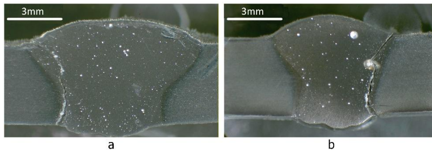
Fig. 21: Cross section of the fracture path in the samples: a) W6N and b) W6R.
