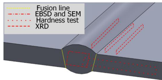
Fig. 3: Schematic cross-section showing the sampling locations for metallography, SEM, EBSD, hardness measurements, and XRD
