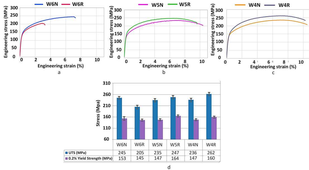
Fig. 18: Tensile properties of the welded samples: engineering stress–strain curves of samples a) W6N and W6R, b) W5N and W5R, c) W4N and W4R, d) average UTS and yield strength.
