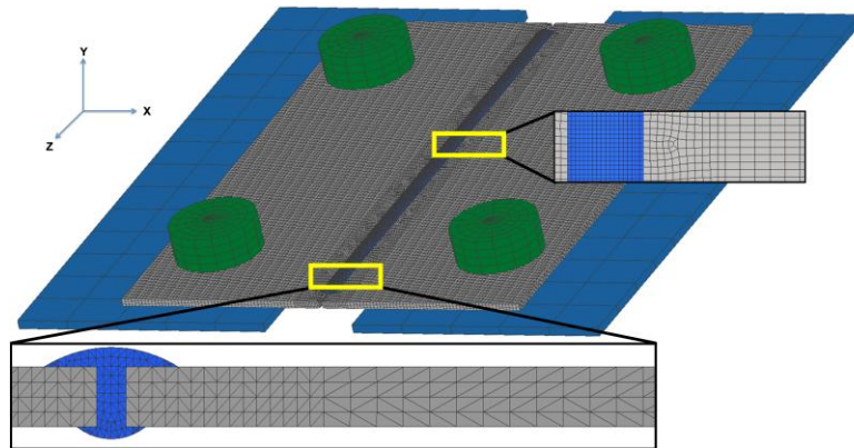
Fig. 2: Finite element model of the welded joint, including the clamping configuration and the locally refined mesh along the weld path.
