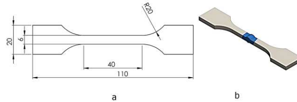
Fig. 4: Tensile test specimen, a) Geometry of the specimen, b) XCT analysis area.
