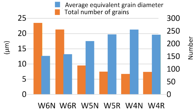
Fig. 12: Average equivalent grain diameter and number of detected grains in the weld metal regions of the different samples.
