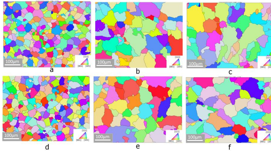
Fig. 11: EBSD maps of the weld metal for the samples: a) W6N, b) W5N, c) W4N, d) W6R, e) W5R, f) W4R.
