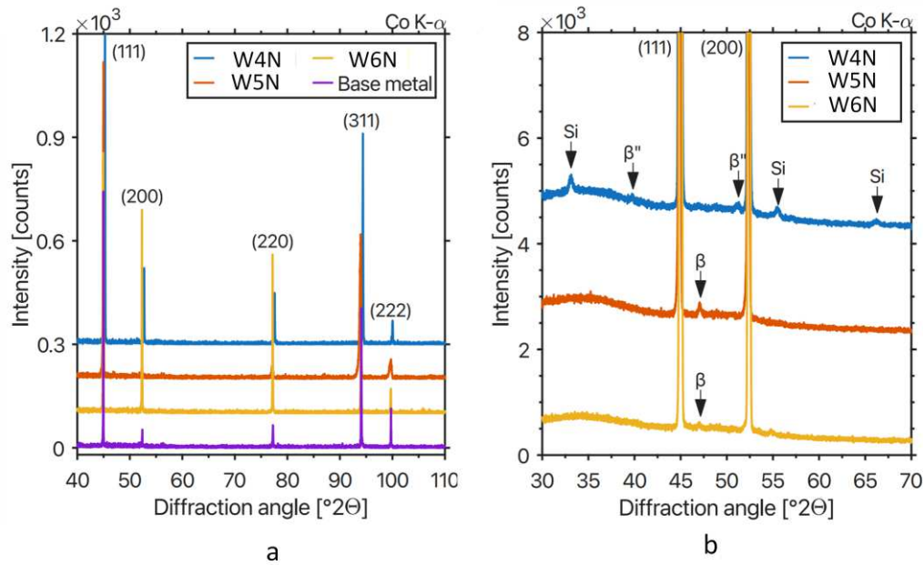
Fig. 16: XRD diffraction patterns of a) base metal, W6N, W5N, and W4N, and b) slow-scan diffraction patterns of W6N, W5N, and W4N within the 2\theta range of 30–70°.
