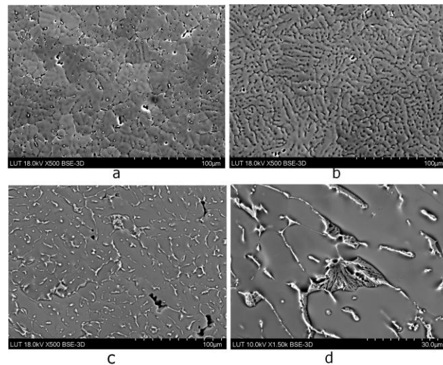
Fig. 14: SEM images of the weld metal microstructure in different samples: a) W6N, b) W5N, c) W4N, and d) higher-magnification image of the W4N weld metal.
