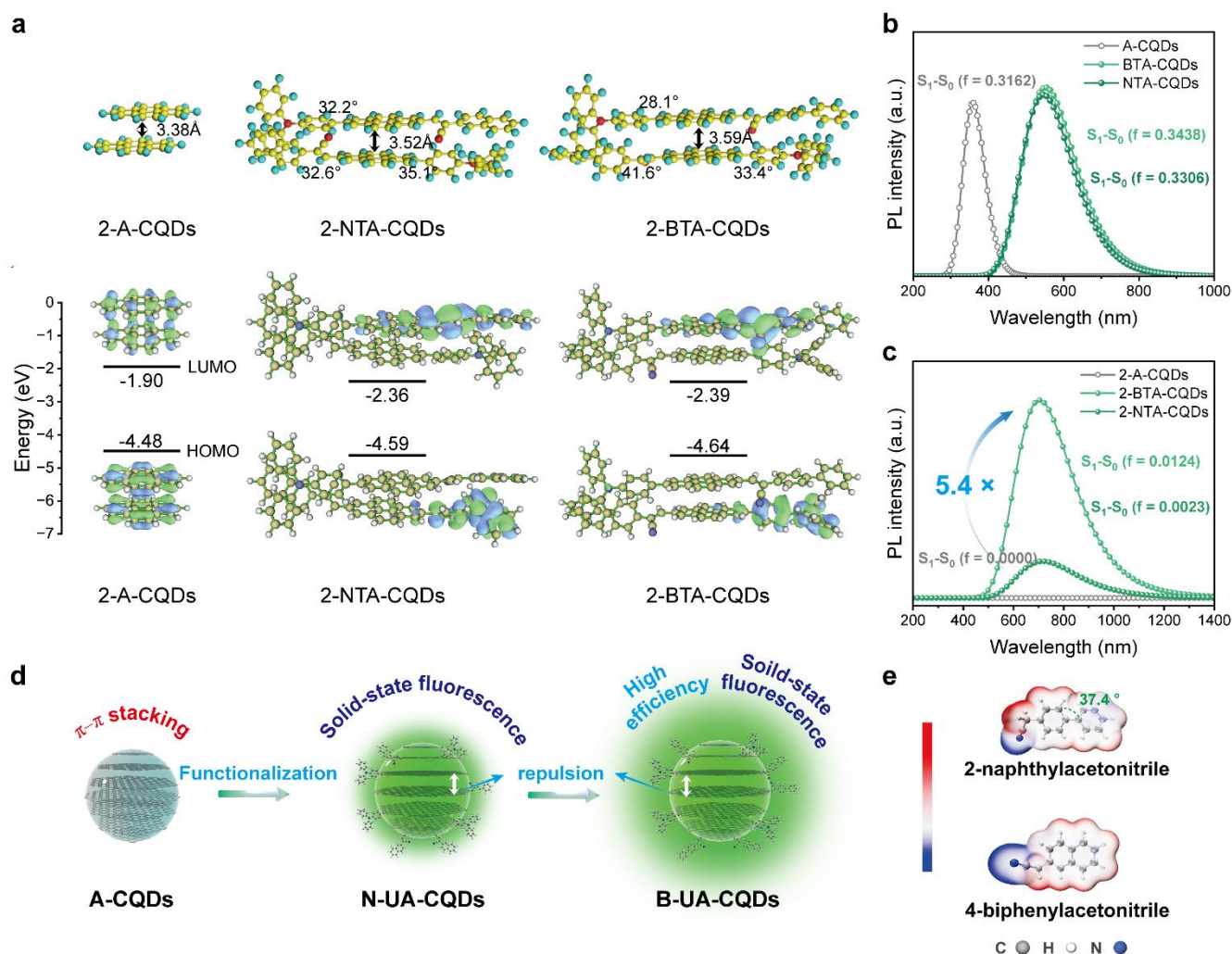
Fig. 3 DFT calculations. (a) Calculated optimized structure and HOMO/LUMO distribution of 2-A-CQDs, 2-NTA-CQDs, and 2-BTA-CQDs. PL spectra (the Gaussian broadening of the first excited state ( S_1-S_0 )) of (b) A-CQDs, NTA-CQDs, and BTA-CQDs, and (c) 2-A-CQDs, 2-NTA-CQDs, and 2-BTA-CQDs. (d) Schematic diagram of structural engineering strategy for UA-CQDs. (e) Electrostatic potential map of the precursors.
