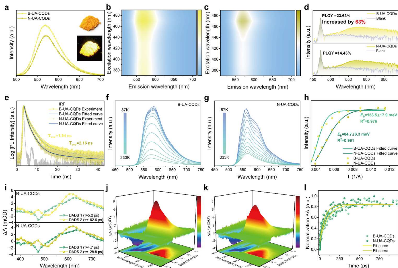
Fig. 4 Optical characteristics of UA-CQDs. (a) PL spectra in the solid state of UA-CQDs and images of the B-UA-CQDs under daylight (up) and UV light (down). Two-dimensional pseudocolor map of normalized excitation-dependent PL spectra of (b) B-UA-CQDs and (c) N-UA-CQDs. (d) The PLQY of UA-CQDs in the solid state under 470 nm excitation. (e) Time-resolved PL spectra of UA-CQDs in the solid state. Temperature-dependent PL spectra from 87 K to 333 K of (f) B-UA-CQDs and (g) N-UA-CQDs. (h) The exciton binding energy fitted by the Arrhenius equation. (i) TA spectra with global fitting results with two exponent decay functions. Three-dimensional colour-mapped surface plot illustrating the TA spectra of (j) B-UA-CQDs and (k) N-UA-CQDs. (l) Kinetic fitting curve at 510 nm.
