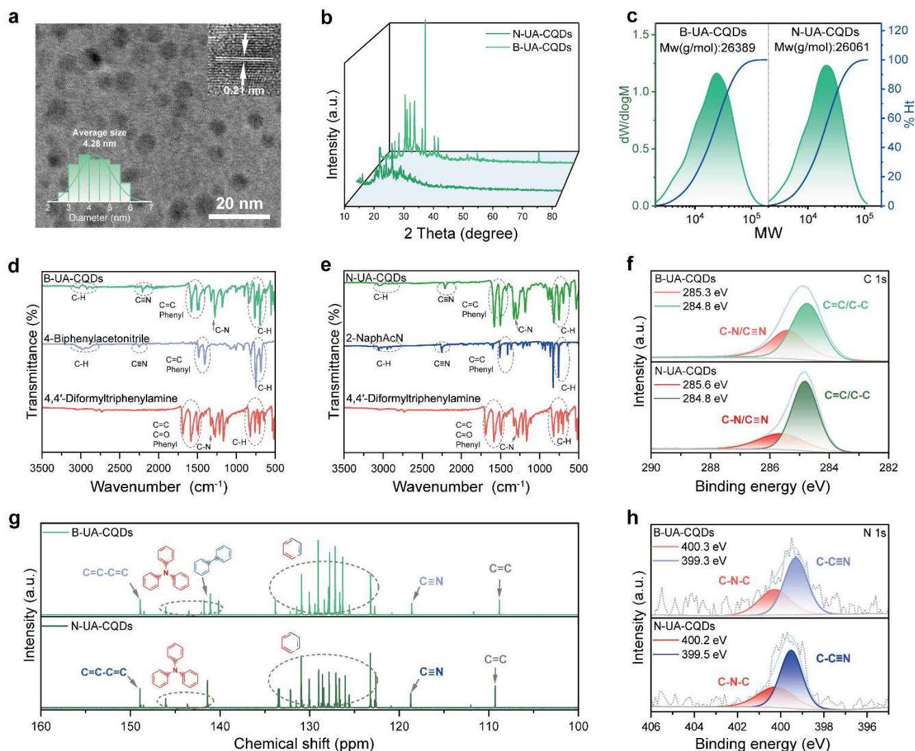
Fig. 2 Structural characterization of UA-CQDs. (a) TEM image of B-UA-CQDs. Inserts present the corresponding HRTEM image and diameter histogram. (b) XRD patterns of UA-CQDs. (c) Molecular weight distributions of UA-CQDs. FT-IR spectra of (d) B-UA-CQDs and (e) N-UA-CQDs along with their corresponding precursors. (f) High-resolution C 1s spectra of UA-CQDs. (h) High-resolution N 1s spectra of UA-CQDs. (g) ^{13}\text{C} NMR signals of UA-CQDs.
