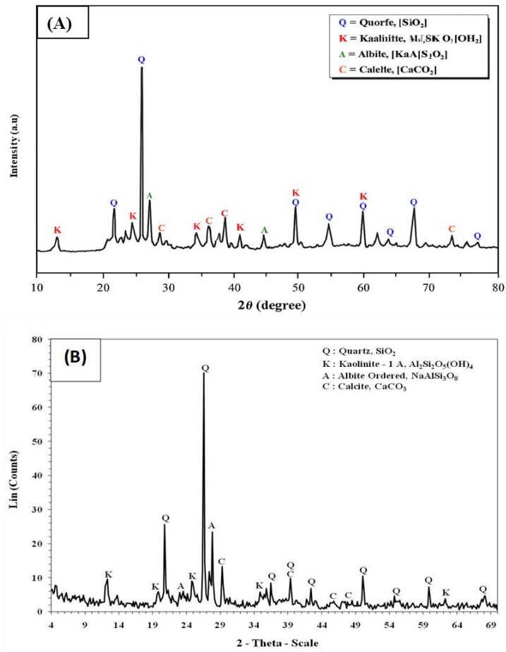
S. 1: XRD pattern for: (A) Ceramic sludge, (B) Ceramic dust
