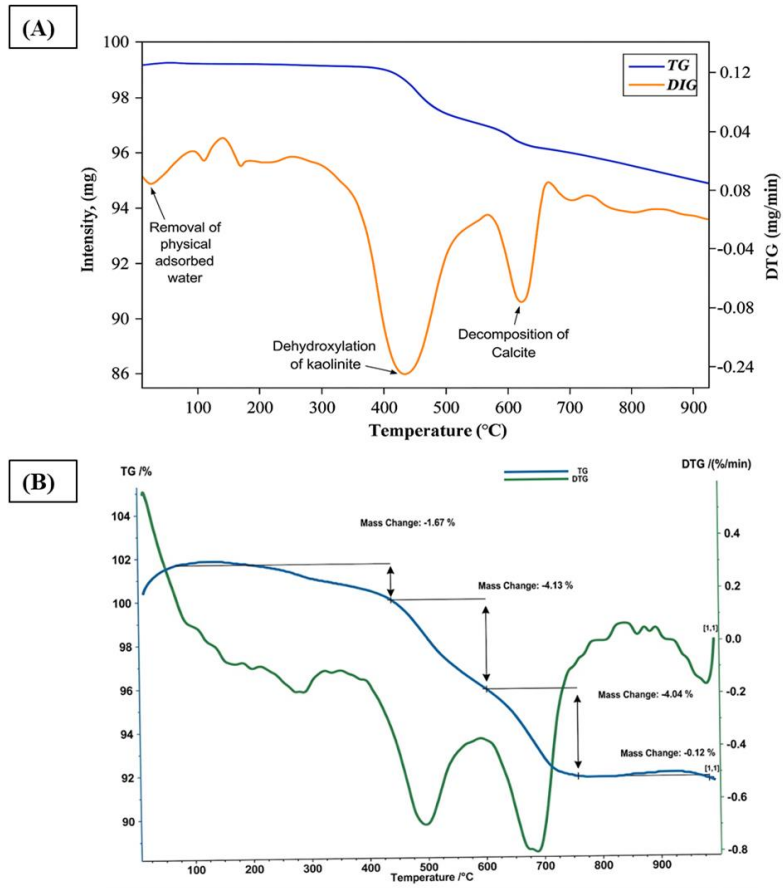
S. 2: DTA – TGA pattern for: (A) Ceramic sludge, (B) Ceramic dust
