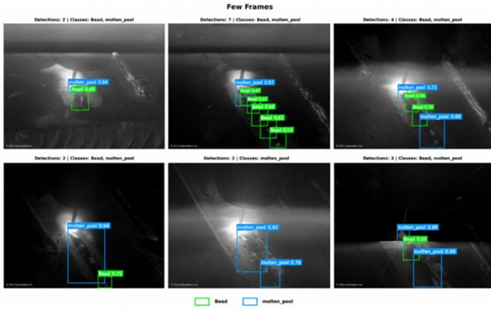
Fig. 5 Representative YOLOv8n detection results across diverse welding conditions, illumination levels, and bead geometries.
