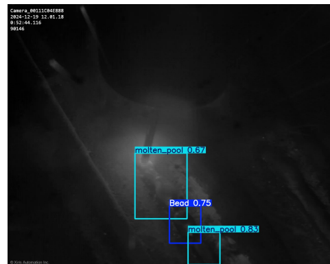
(f) Molten and Bead detection
