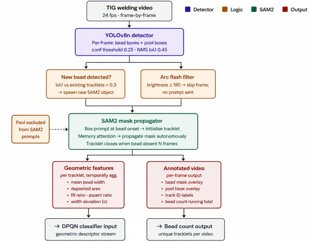
Fig. 7 YOLOv8n Guided SAM2 Video Segmentation Architecture
