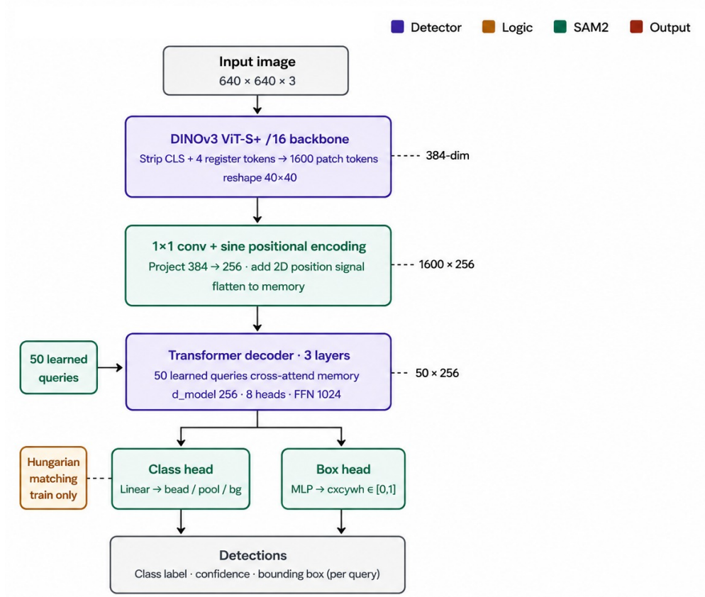
Fig. 4 DINO-DETR Architecture
