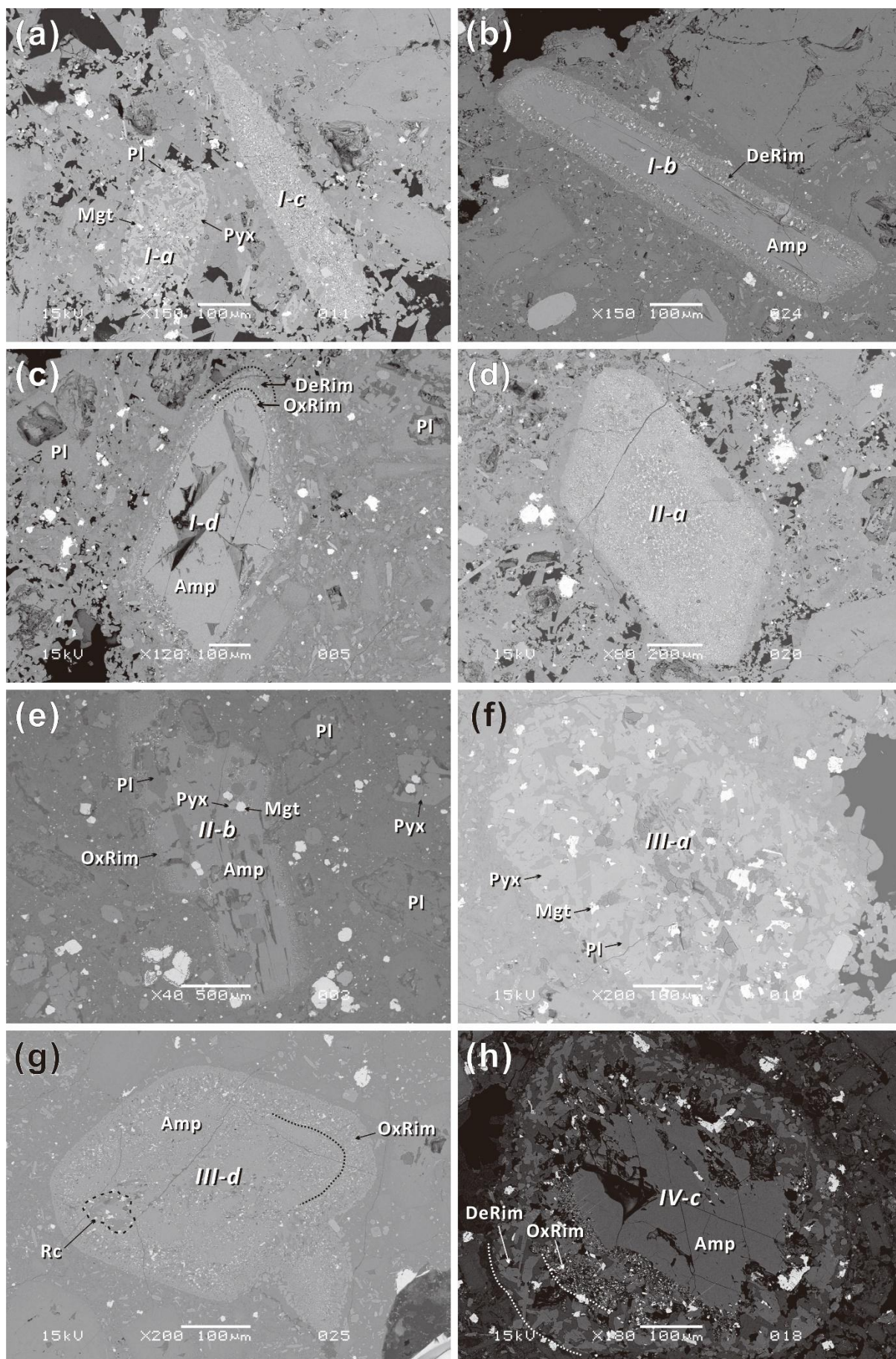
Fig. 6 Back-scattered electron images of DT-01 amphibole phenocrysts: (a) a decompressed
