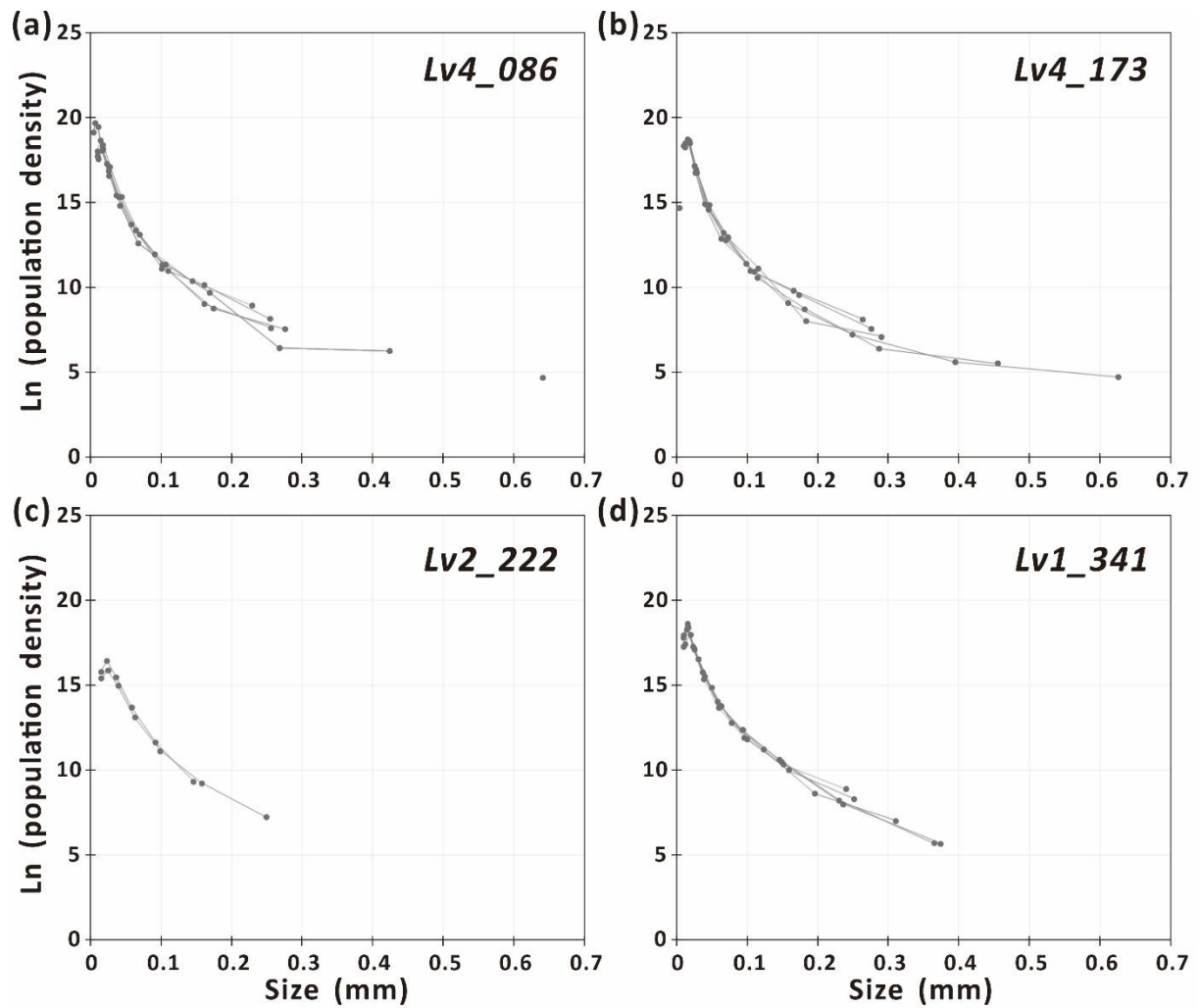
Fig. 9_Crystal size distributions (CSDs) illustrating feldspar microlite nucleation and growth in DT-01 samples. (a) The Lv4 sample, with the slowest magma ascent rate, exhibits an upward-concave curve indicating strong crystal growth. Its high y-axis intercept (nearly 20 \text{mm}^{-4} ) indicates nucleation dominance under rapid cooling. (b) Some Lv4 samples reach larger crystal sizes above 0.6 mm. (c) The Lv2 sample illustrates a lower y-axis intercept (about 16 \text{mm}^{-4} ) and smaller crystal size, resulting from melt undercooling in a short crystallization time. (d) The Lv1 sample, similar to Lv4, exhibits a slightly upward-concave line for crystal growth. Samples in Lv3 have no CSD data for the glassy groundmass lacking microlites.
