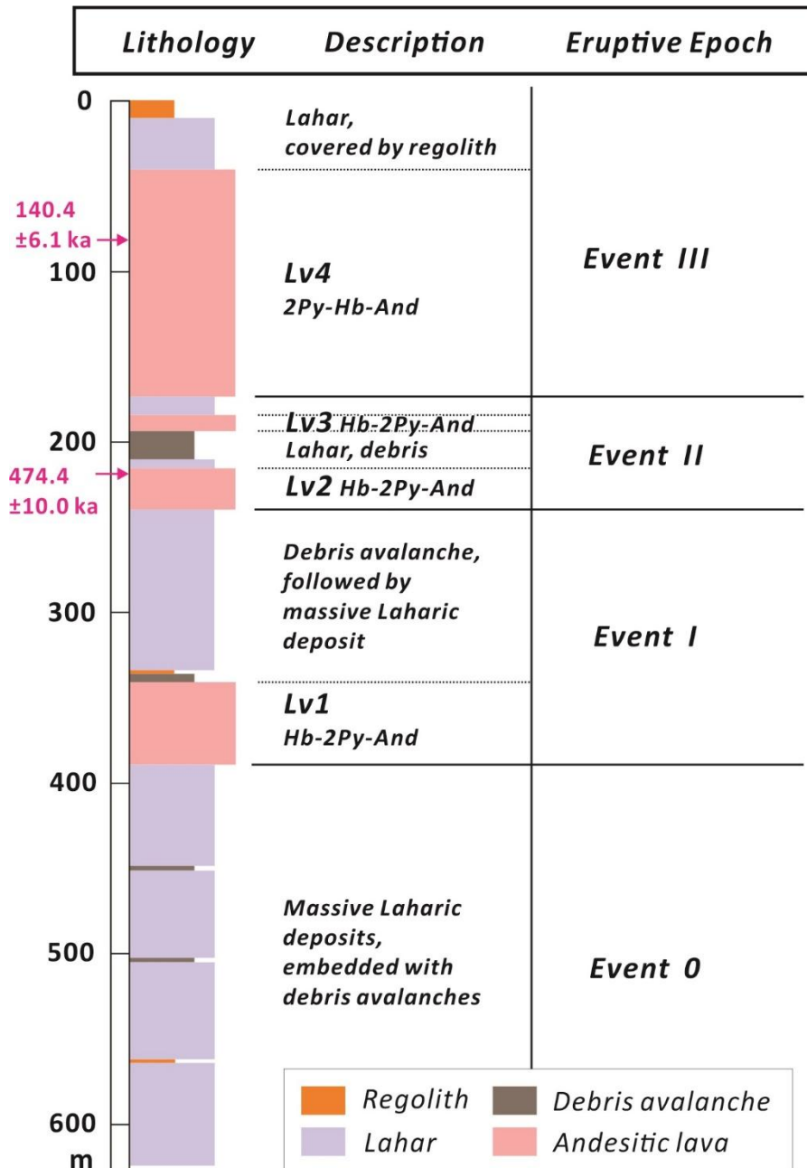
Fig. 3_Drilling core DT-01 lithologic column (see Fig. 2 for drilling core locality). It consists of massive laharic deposits, lava, and a few debris avalanches in alternation. At least four eruptive events are recorded in the section. Four andesitic lava units, namely Lv1 (hornblende two-pyroxene andesite), Lv2 (hornblende two-pyroxene andesite), Lv3 (hornblende two-pyroxene andesite), and Lv4 (two-pyroxene hornblende andesite) in ascending order, are associated with events I, II, and III. ^{40}\text{Ar}/^{39}\text{Ar} dating of lava groundmass at depths of 90 m (Lv4) and 214 m (Lv2) yields cooling (eruption) ages of 140 ka and 474 ka, respectively.
