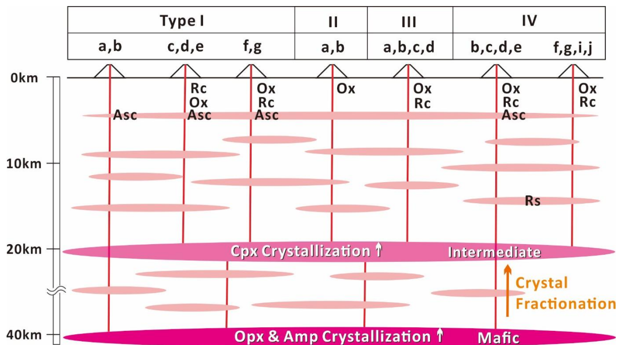
Fig. 11_ Illustration of amphibole evolution routes based on amphibole decomposition processes (Fig. 5) and mineral thermobarometry. Numerous magma batches dispersed throughout the crust act as buffers for amphibole crystallization. These fractionated intermediate magma batches, derived from primary mafic magmas, gradually cooled during ascent and produced abundant amphiboles. As the primary magma ascended, it underwent crystal fractionation (orthopyroxene, amphibole, and clinopyroxene), magma segregation (favoring amphibole crystallization), magma stagnation (at depths of 4-22 km), and magma mixing (recharged mafic magmas and fractionated magma batches), sequentially.
