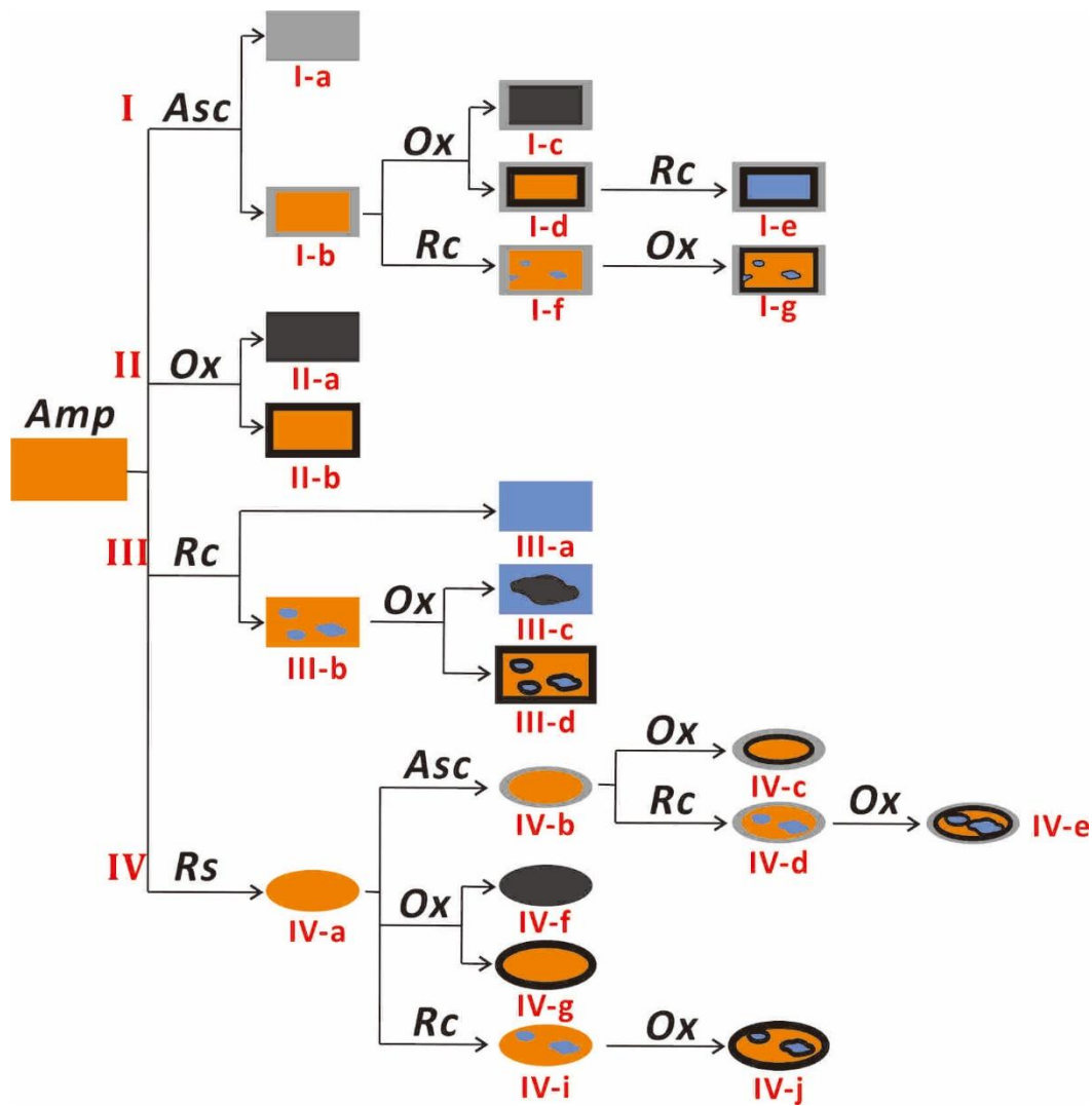
Fig. 5_Flowchart of amphiboles experiencing a sequential decomposition process: I. magma decompression (Asc), II. thermal oxidation (Ox), III. recrystallization (Rc), and IV. resorption (Rs). Complex amphibole occurrences are summarized in the 22 textural types, from I-a to IV-j, illustrating crystal evolving stages, e.g., an amphibole crystal of type I-g would undergo decompression (Asc), recrystallization (Rc), and thermal oxidation (Ox) sequentially.
