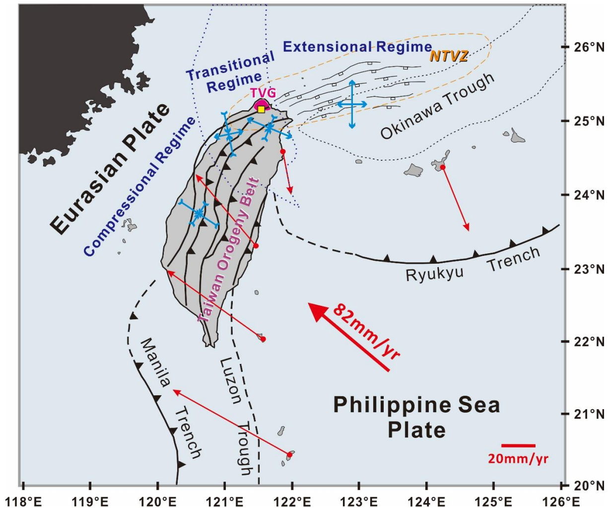
Fig. 1_Regional tectonic setting of Taiwan and its neighboring area (summarized from Kong et al. 2000; Hu et al. 2002; Hsu et al. 2009). Taiwan, formed by the collision of the Philippine Sea Plate and the Eurasian Plate, sits at the junction of two subduction systems, the Ryukyu Trench to the east and the Manila Trench to the south. The Tatun Volcano Group (TVG), located in the southwestern part of the northern Taiwan volcanic zone (NTVZ), poses a significant risk due to its proximity to Taipei City. The TVG lies in a transitional stress regime
