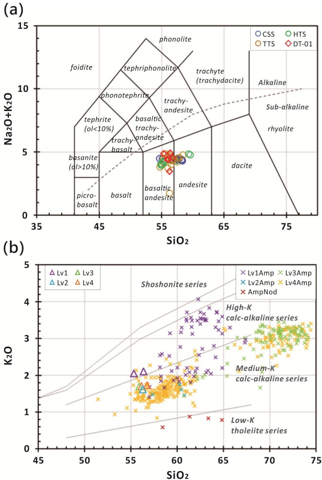
Fig. 10 (a) Total alkalis-silica (TAS) diagram of the TVG volcanic rocks – Chihsing volcanoes (CSS), Huangtsui volcanoes (HTS), Tatun volcanoes (TTS) (Song et al. 2004, 2006, 2007), and the DT-01 core (this study). (b) \text{K}_2\text{O} vs \text{SiO}_2 plots. Cross symbols – Lv1, Lv2, Lv3, Lv4, and AmpNod – represent melt compositions estimated from amphiboles in Lv1, Lv2, Lv3, Lv4, and amphibole-rich nodules, respectively, using amphibole chemometric
