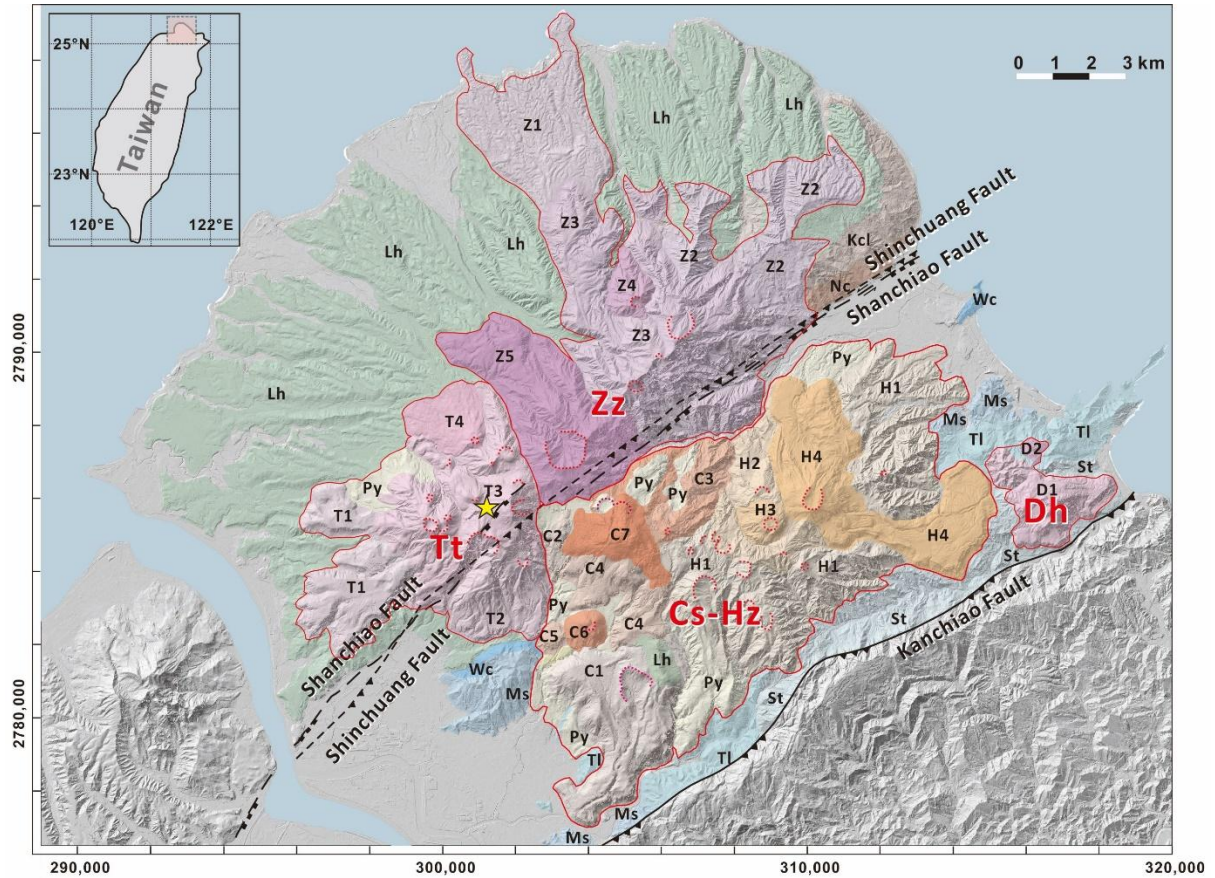
Fig. 2_ The Tatun Volcano Group (TVG) is divided into four synthem (unconformity- bounded units for volcanic strata: Chang 1975; Marti et al. 2018; Lucchi et al. 2019): Chutze (Zz), Tatun (Tt), Chihsing-Huangtsui (Cs-Hz), and Tinghuohsiu-Nantze (Dh). The Shanchiao Fault separates the TVG into northwestern (Chutze and Tatun synthem) and southeastern (Chihsing-Huangtsui and Tinghuohsiu-Nantze synthem) parts. Each synthem comprises several overlapping volcanoes composed of andesitic-to-basaltic-andesitic lava domes, lava flows, volcanic avalanches, and vast flooded lahars (Lh). The numbering of each lithosome (e.g., T1, T2, T3) indicates its eruptive order within the synthem. The sedimentary basement exposed along the southeastern fringe of the TVG comprises Oligocene-to-Miocene strata, including the Wutsishan (Wc), Mushan (Ms), Taliao (Tl), and Shihti (St) Formations. The studied core, DT-01 (yellow star), is located at Mt. Tatun within the Tatun synthem (Tt).
