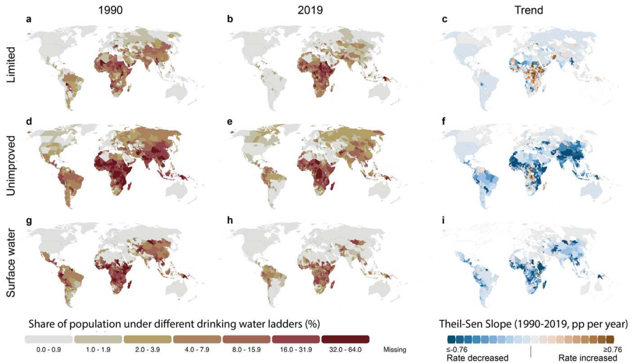
Figure 1. Share of population under different drinking water ladders. Limited access to drinking water (a-c), unimproved access (d-f), and surface water access (g-i). The status is shown for 1990 (a, d, g) and 2019 (b, e, h), the common span of the years of access to drinking water data (1990-2023) and water quality data (1980-2019). The trend (c, f, i) was calculated using Theil-Sen slope, using p > 0.05 as a threshold for significant trend.
