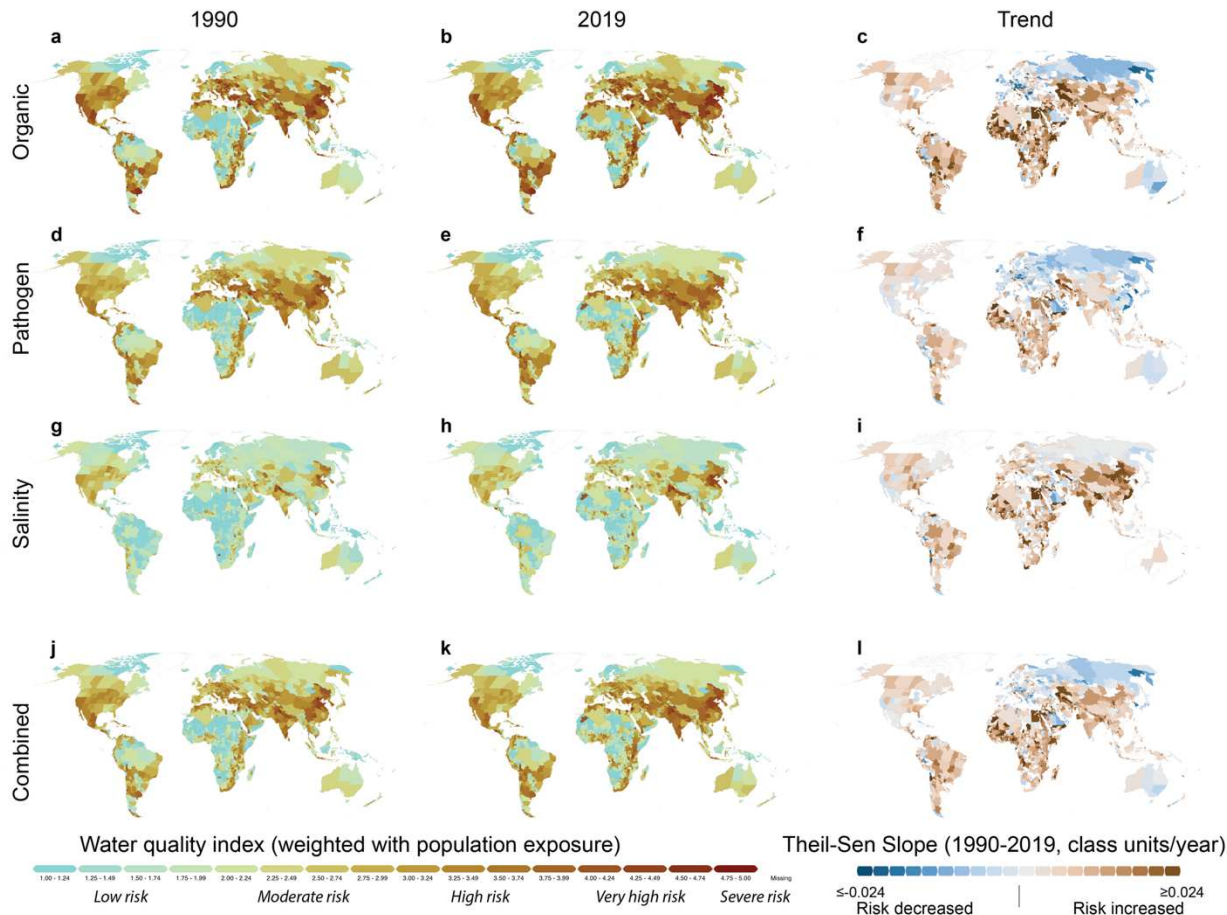
Figure 2. Water quality status and trends. Organic contamination risk (a-c), pathogen contamination risk (d-f), salinity risk (g-i), and combined risk indicator (j-l). The status is shown for 1990 (a, d, g) and 2019 (b, e, h), the common span of the years of access to drinking water data (1990-2023) and water quality data (1980-2019). The trend (c, f, i) was calculated using Theil-Sen slope, using p < 0.05 as a threshold for significant trend. See Table 1 for water quality thresholds, and Methods for how the combined risk indicator was calculated.
