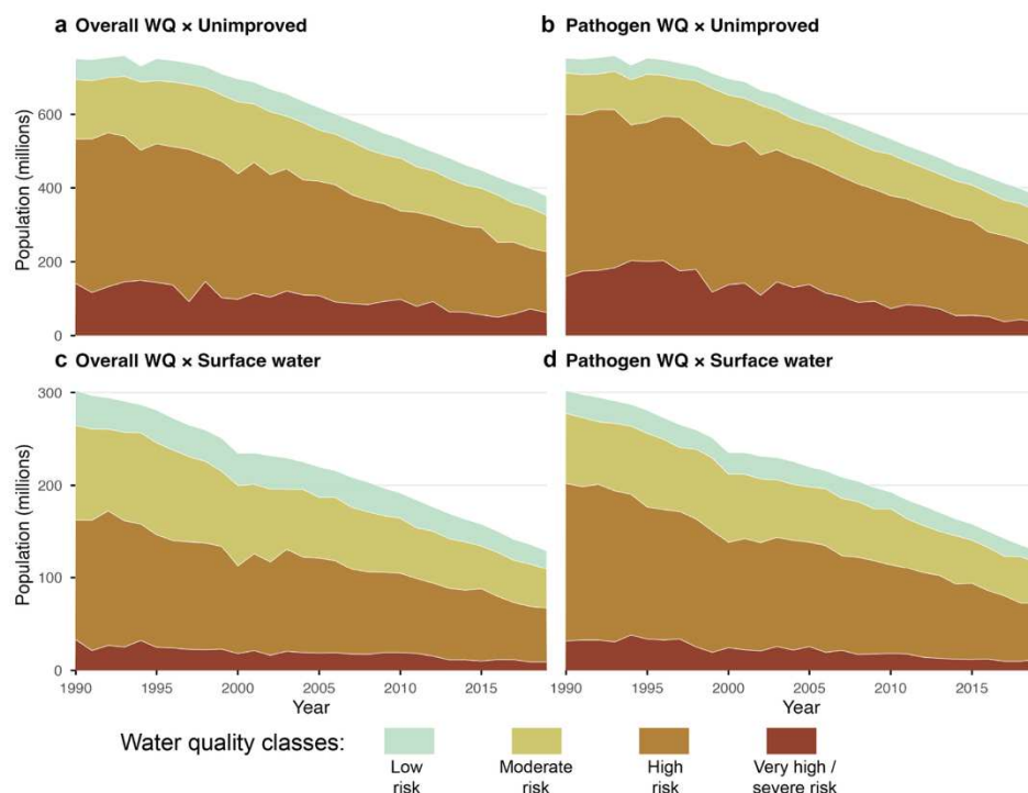
Figure 5. Population under each water quality class for unimproved and surface water access to drinking water. See water quality classes in Table 1.
