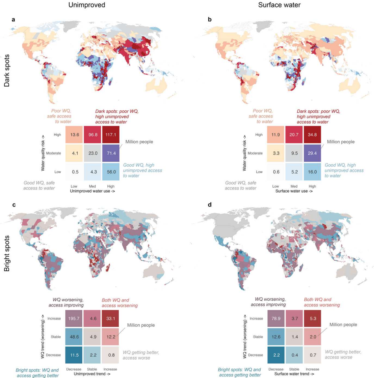
Figure 6. Bright spot and dark spot analysis using the current status and trends of combined water quality and unimproved and surface water service levels. Bivariate maps show an intersection between combined water quality and unimproved (a) and surface water (b) service levels, and trends of combined water quality and unimproved (c) and surface water (d) service levels. The bivariate legends show the population count in each category. See Supplementary Figures S8-S10 for the distribution of organic, pathogen, and salinity, respectively.
