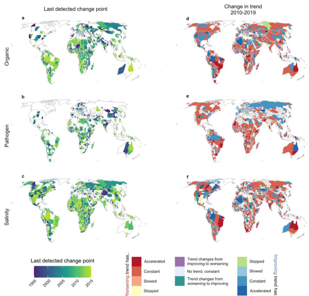
Figure 4. The year of the last detected changepoint and the classification of the recent changes in trend over the last ten years of the study period, 2010-2019, for organic contamination (a, d respectively), pathogen contamination (b, e) and salinity (c, f). Due to a minimum segment length of 5 years, the first and last possible change points are 1995 and 2015, respectively. See Supplementary Figure S7 for continental aggregations.
