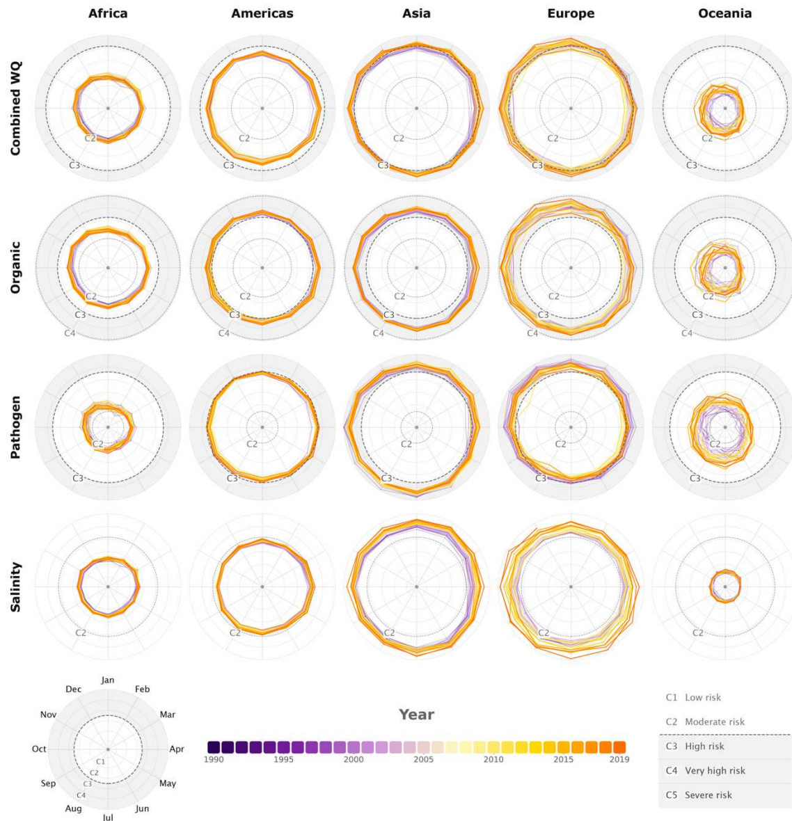
Figure 3. Water quality risk spirals showing the continental mean seasonality and evolution of risks over 1990-2019. The mean water quality indicators have been weighted using the population under surface water and unimproved service levels, and do not consider population under higher service levels.
