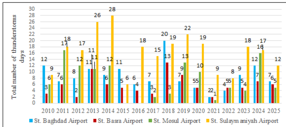
Figure 3. Annual distribution of thunderstorms for the period 2010-2025
