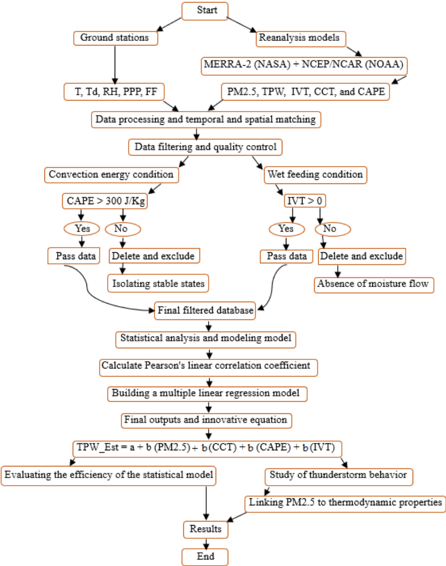
Figure 2. The methodological flowchart for 4 stations (2010-2025)
