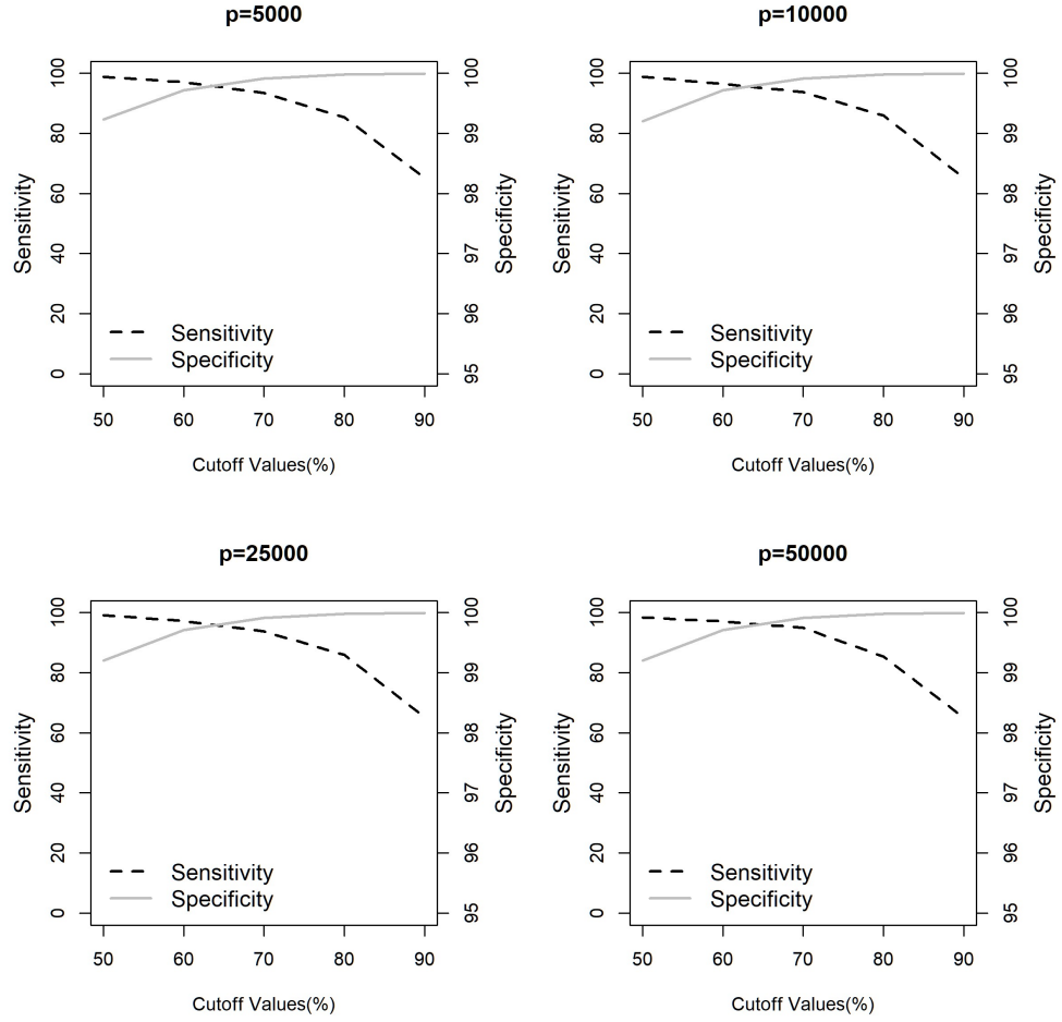
Fig. 3 Sensitivity (dashed line) and specificity (solid line) of Rare-Screening at different cutoff thresholds when n = 500 for different numbers of predictors.
