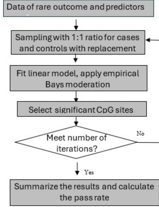
Fig. 1 Rare-Screening method flowchart.
