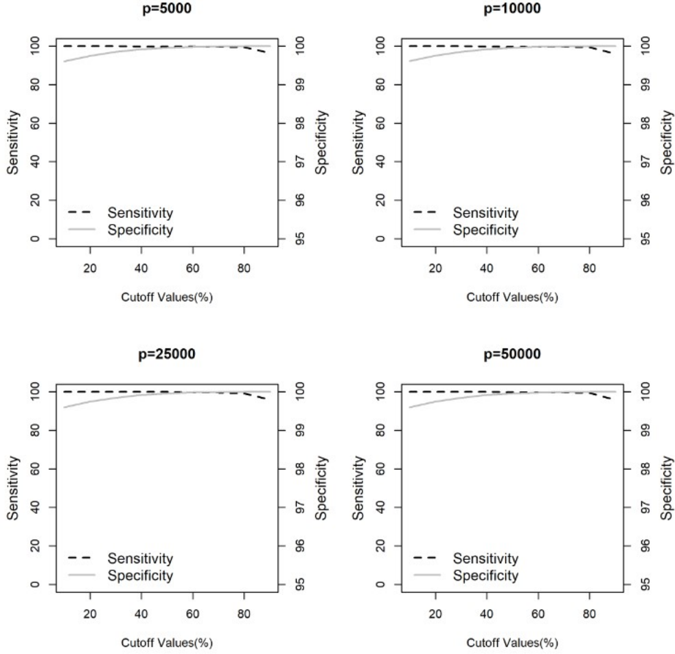
Fig. 6 Sensitivity (dashed line) and specificity (solid line) of Firth-ttScreening at different cutoff thresholds when n = 1000 .
