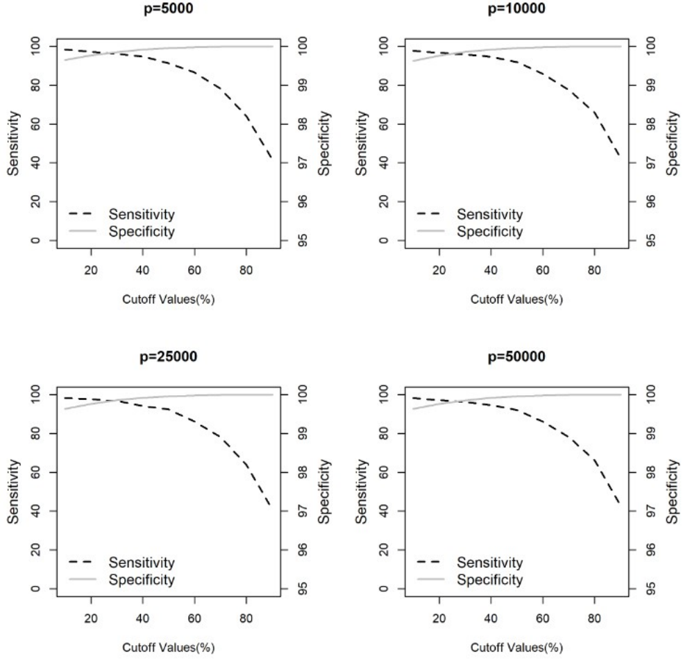
Fig. 5 Sensitivity (dashed line) and specificity (solid line) of Firth-ttScreening at different cutoff thresholds when n = 500 .
