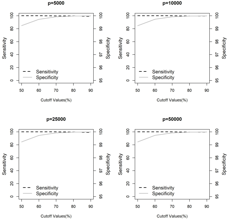
Fig. 4 Sensitivity (dashed line) and specificity (solid line) of Rare-Screening at different cutoff thresholds when n = 1000 for different numbers of predictors.
