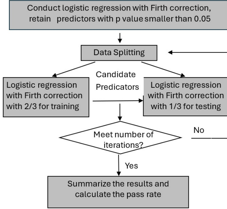
Fig. 2 Firth-ttScreening method flowchart.
