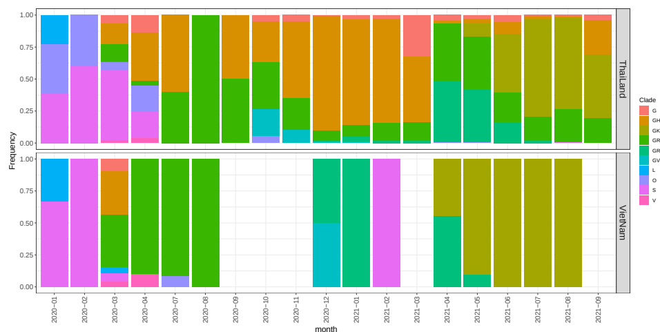
Supplementary Figure 1: Percentage of Clades by month in Vietnam and Thailand.
