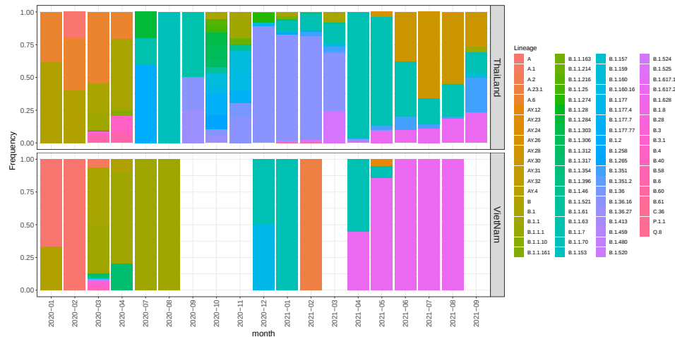
Supplementary Figure 2: Percentage by Lineage by month in Vietnam and Thailand.
