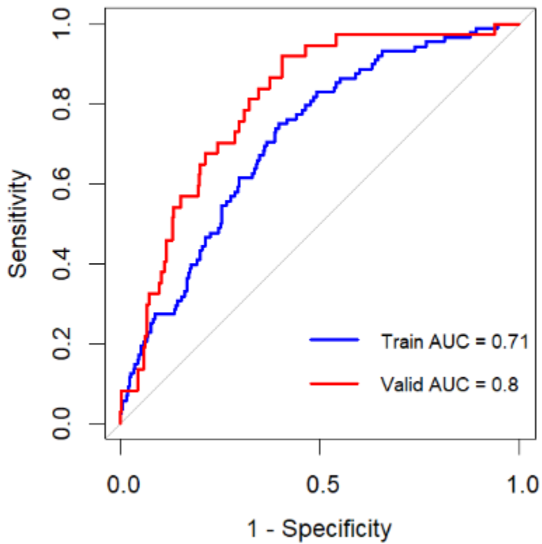
Figure 2 Receiver operating characteristic (ROC) curves for the prediction model in the training and validation sets.
