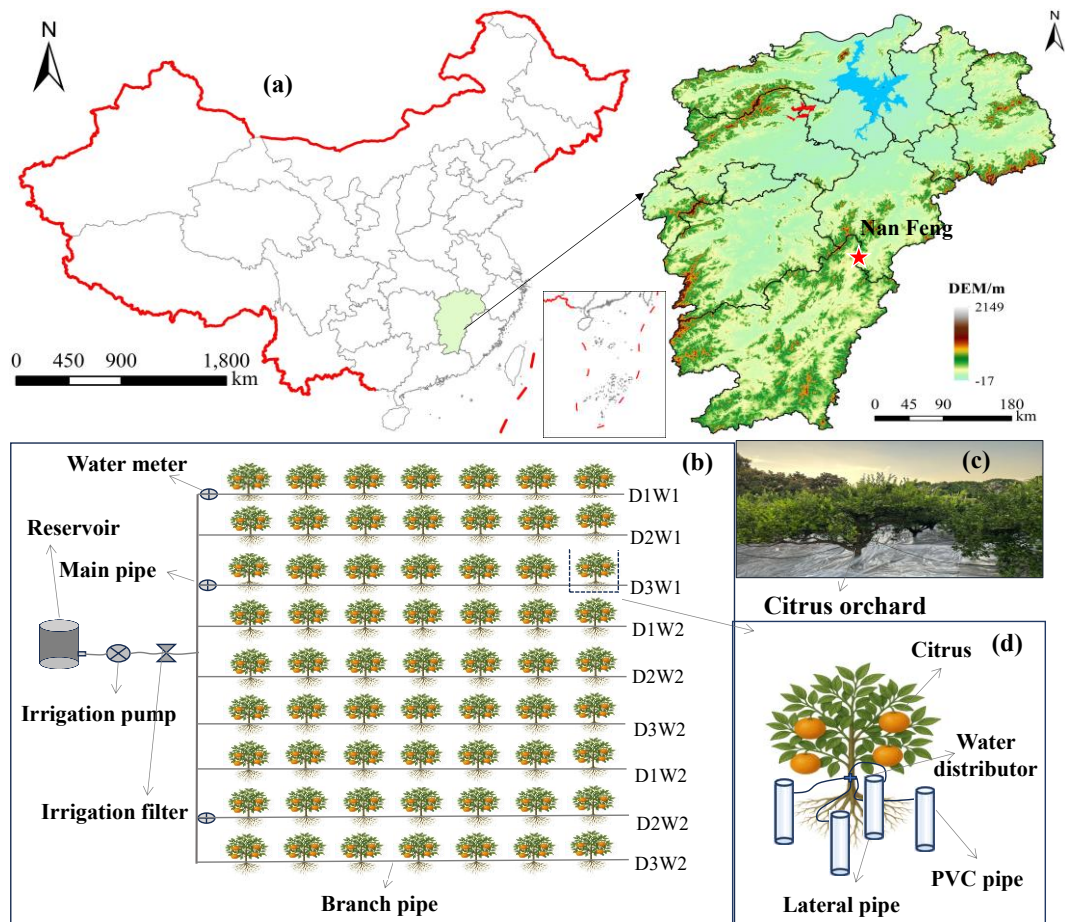
Fig. 1 Schematic diagram of the study area location and deep irrigation system (a, location of the study area; b, layout of irrigation systems for different treatments in the experimental plot; c, schematic diagram of the citrus orchard; d, structural diagram of the irrigation emitter)
