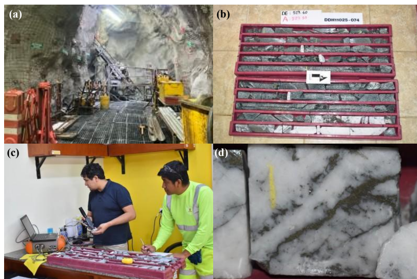
Fig. 4. Materials and characterization of the diamond-drill core. (a) Underground drill platform used for diamond drilling; (b) core boxes from DDH11025-074 corresponding to the 519.60–529.30 m interval; (c) acquisition of drill-core reflectance spectra using a TerraSpec 4 Hi-Res spectrometer; and (d) representative texture of a quartz–carbonate structure containing visible sulfides.
