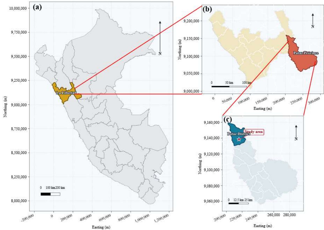
Fig. 1. Geographic location of the study area in northern Peru. (a) Location of the La Libertad Region within Peru; (b) location of Pataz Province within the La Libertad Region; and (c) location of the study area within the Pataz district. Coordinates are expressed in meters using the UTM coordinate system.
