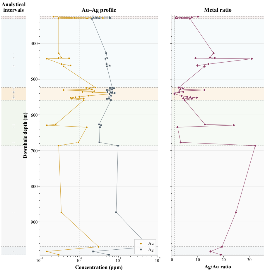
Fig. 8. Downhole distribution of Au–Ag and associated elements in DDH11026-081
