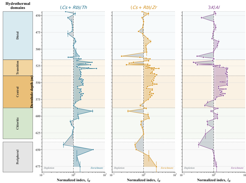
Fig. 9. Downhole variation and statistical differentiation of the lithogeochemical indices in DDH11025-074
