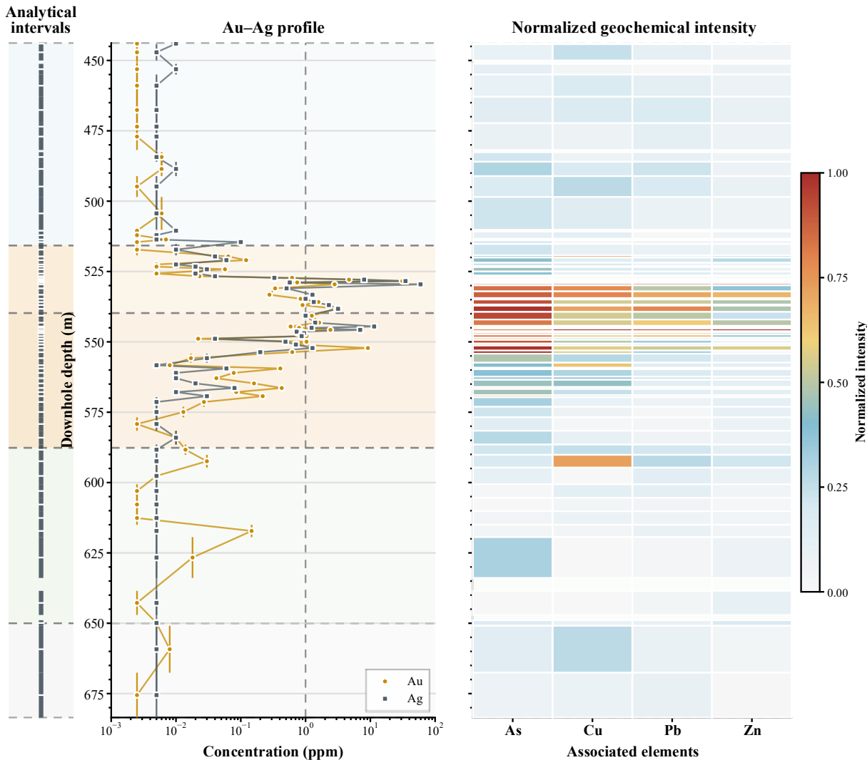
Fig. 7. Downhole distribution of Au–Ag and associated elements in DDH11025-074
