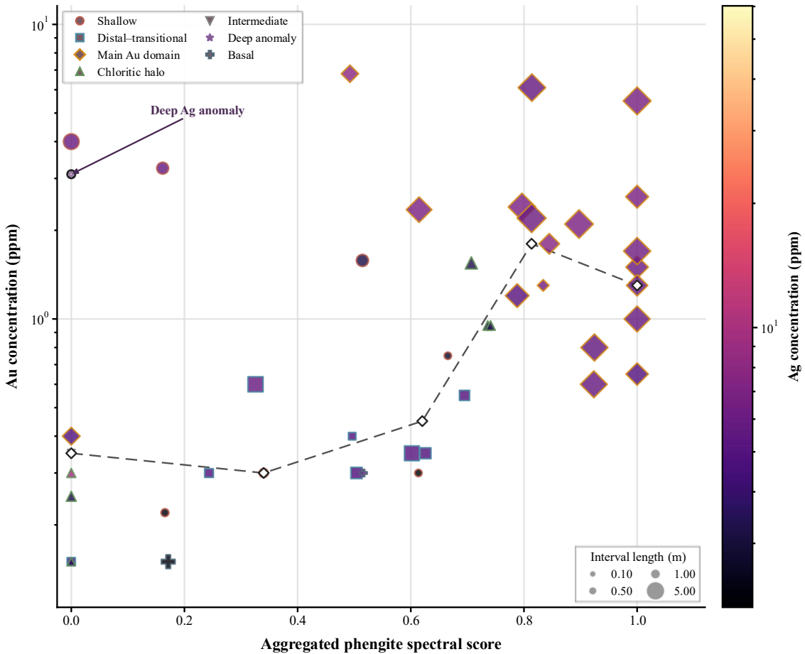
Fig. 12. Relationship between the aggregated phengite spectral score and the distribution of Au–Ag in DDH11026-081
