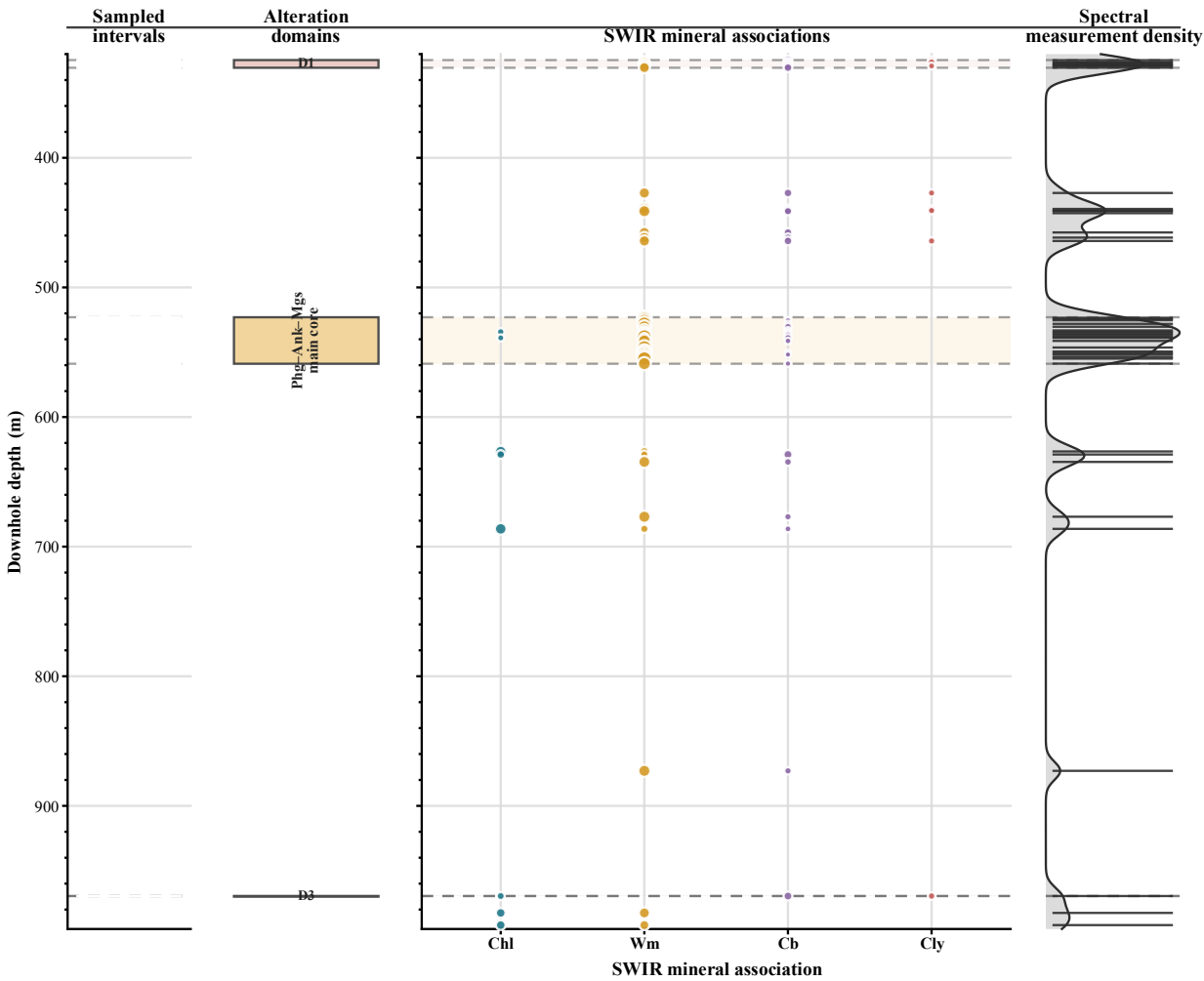
Fig. 6. Downhole distribution of hydrothermal domains and SWIR mineral assemblages in DDH11026-081
