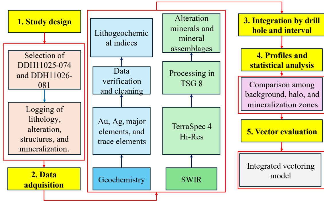
Fig. 3. Methodological workflow for integrating geological, geochemical, and spectral data
