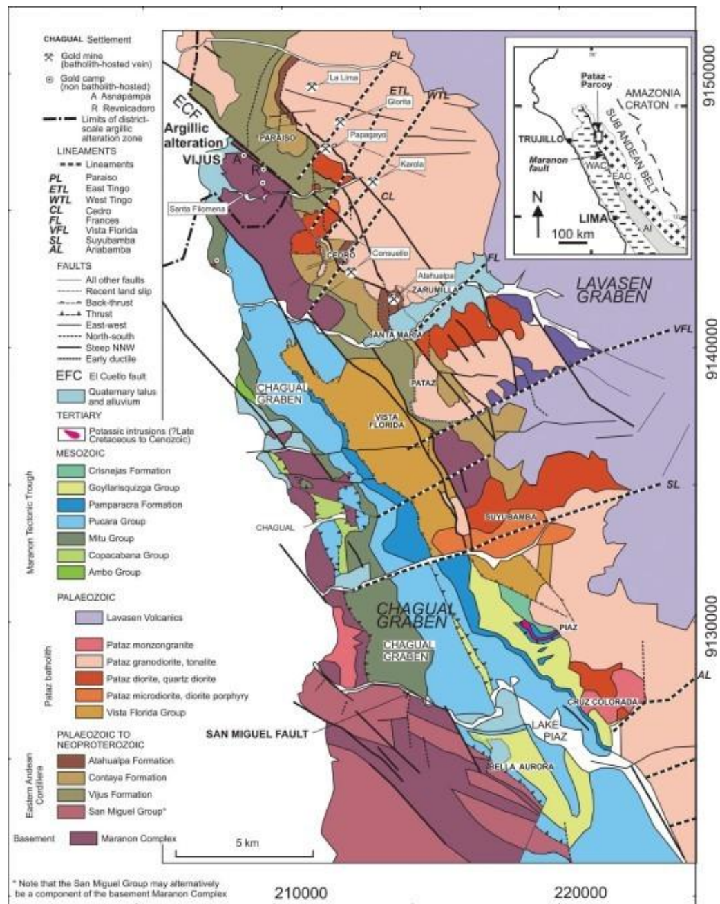
Fig. 2. Geological and structural setting of the Pataz gold district. Modified from Witt et al. (2016).
