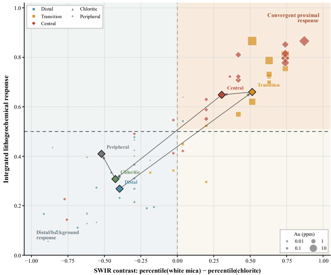
Fig. 11. Convergence of the integrated lithochemical response, SWIR mineralogical contrast, and Au concentration in DDH11025-074
