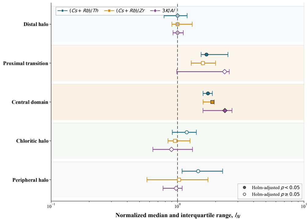
Fig. 10. Normalized medians and interquartile ranges by hydrothermal domain in DDH11025-074
