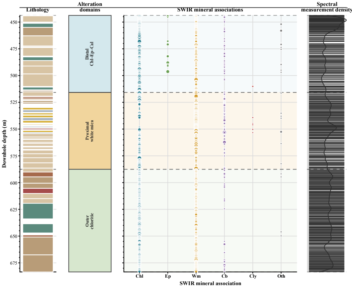
Fig. 5. Downhole distribution of hydrothermal domains and SWIR mineral assemblages in DDH11025-074
