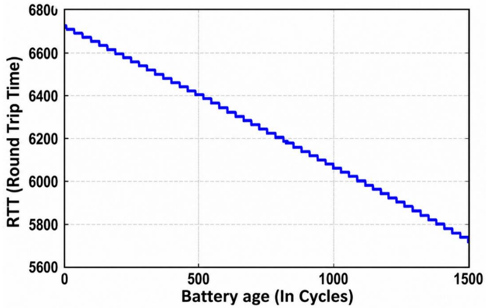
Fig 14. Round-trip time versus Battery's age
