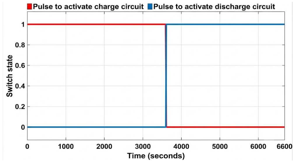
Fig 5. Triggering pulses for MOSFETs in charge and discharge circuits
