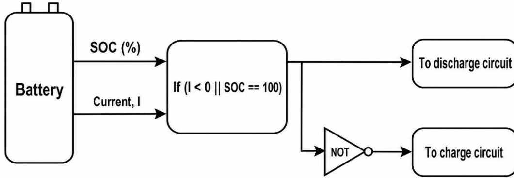
Fig 6. Equivalent model for circuit switching logic
