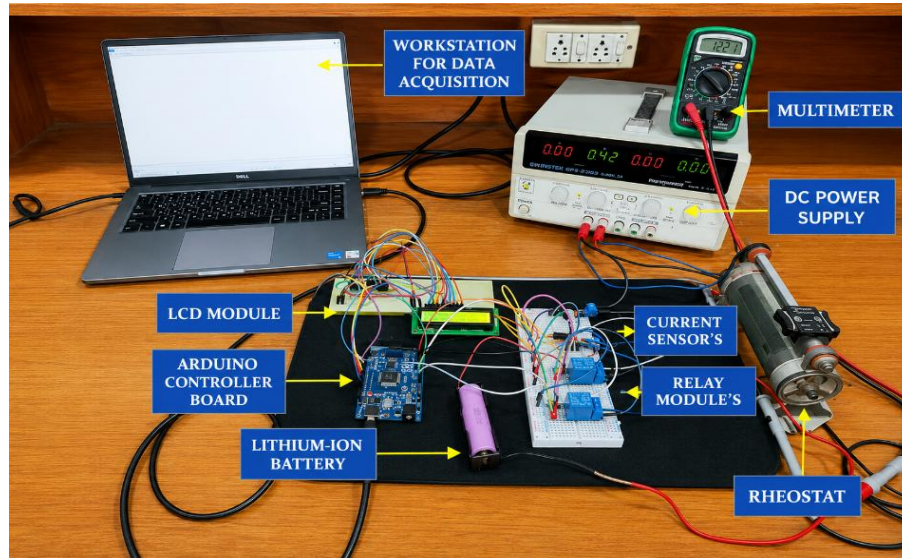
Fig 8. Experimental Setup
