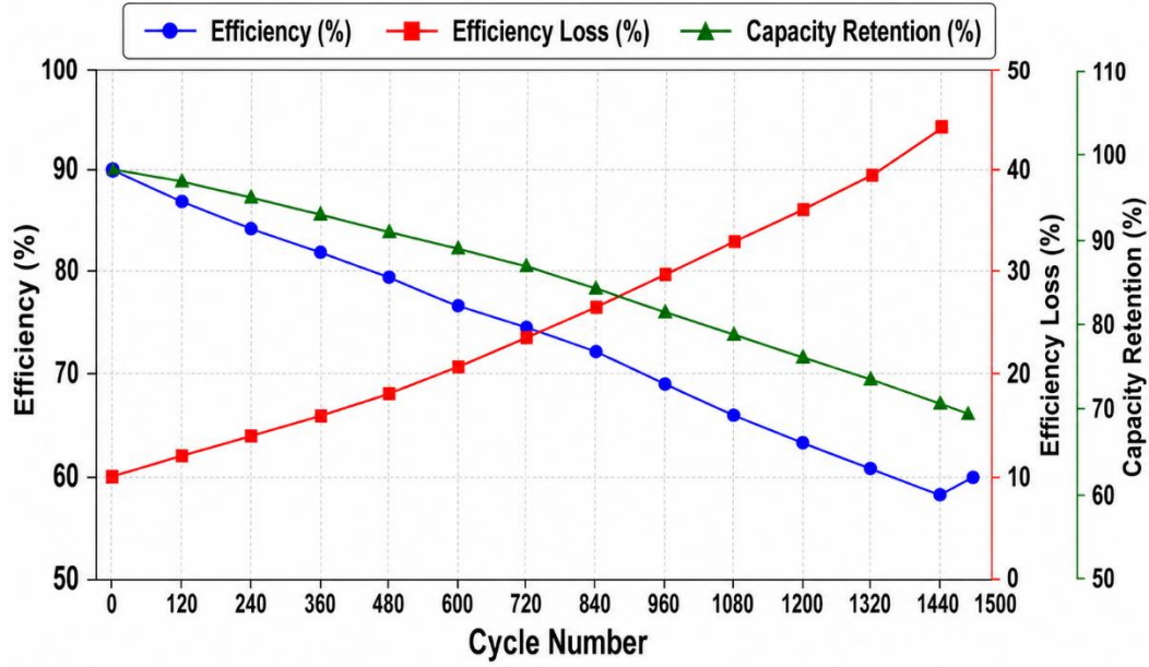
Figure 12. Variation of coulombic efficiency, efficiency loss, and capacity retention with battery cycle number
