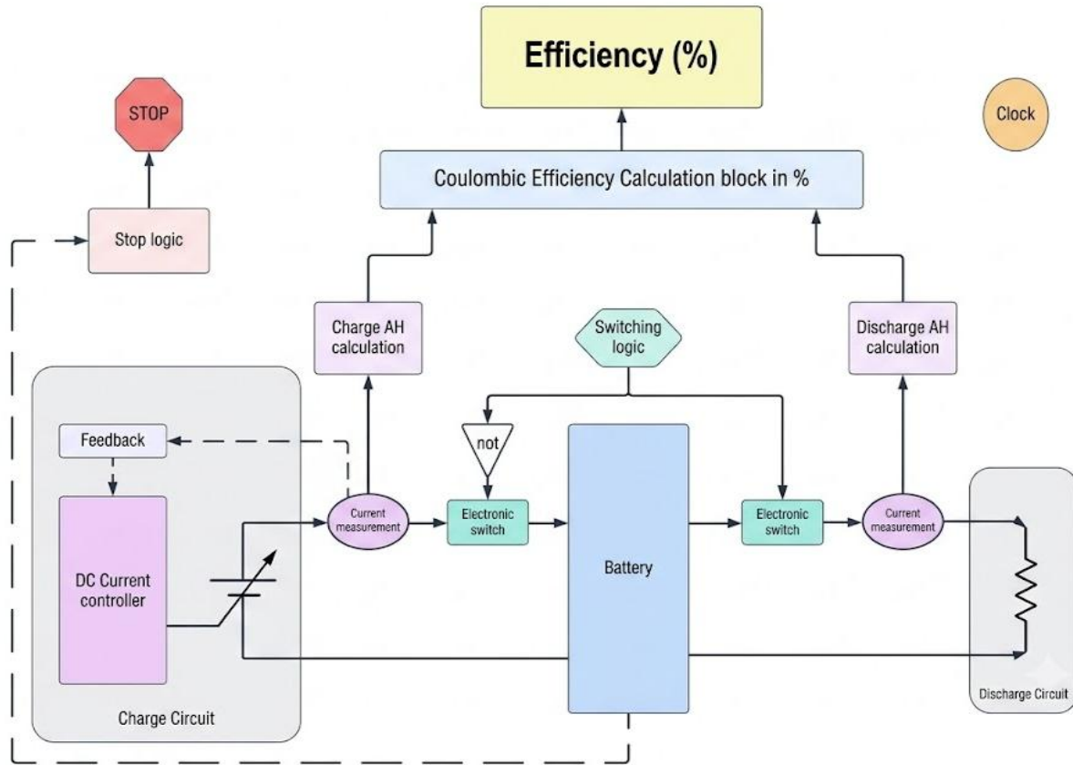
Fig 1. Schematic of the proposed model
