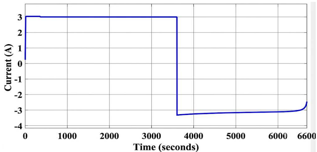
Fig 4. Current profile over a single charge-discharge cycle
