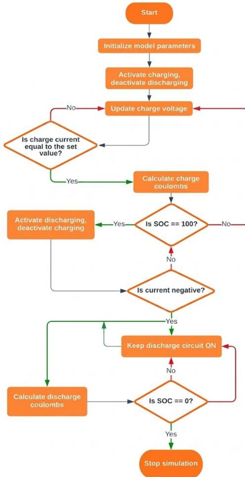
Fig 2. Flow chart for efficiency computing process
