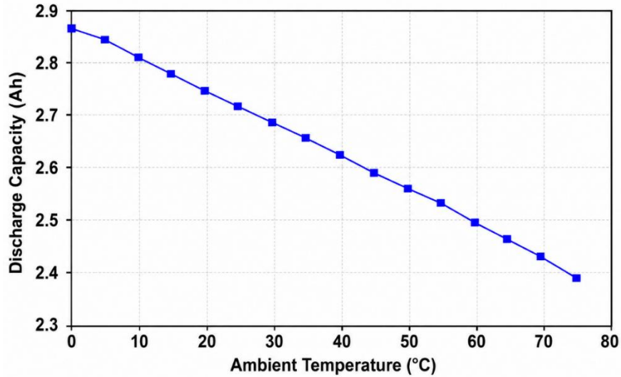
Fig 11. Ambient temperature vs. discharge capacity
