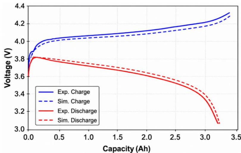
Figure 9 Experimental and simulated voltage profile
