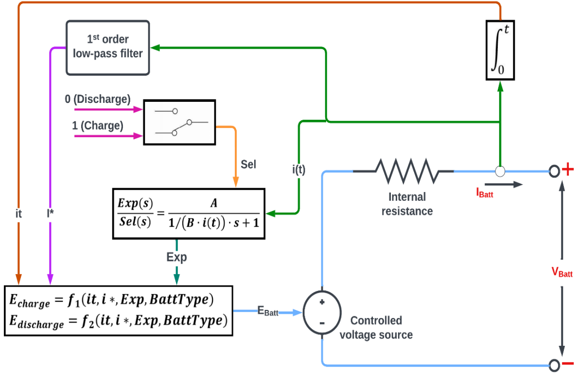
Fig 3. The battery model - Equivalent circuit
