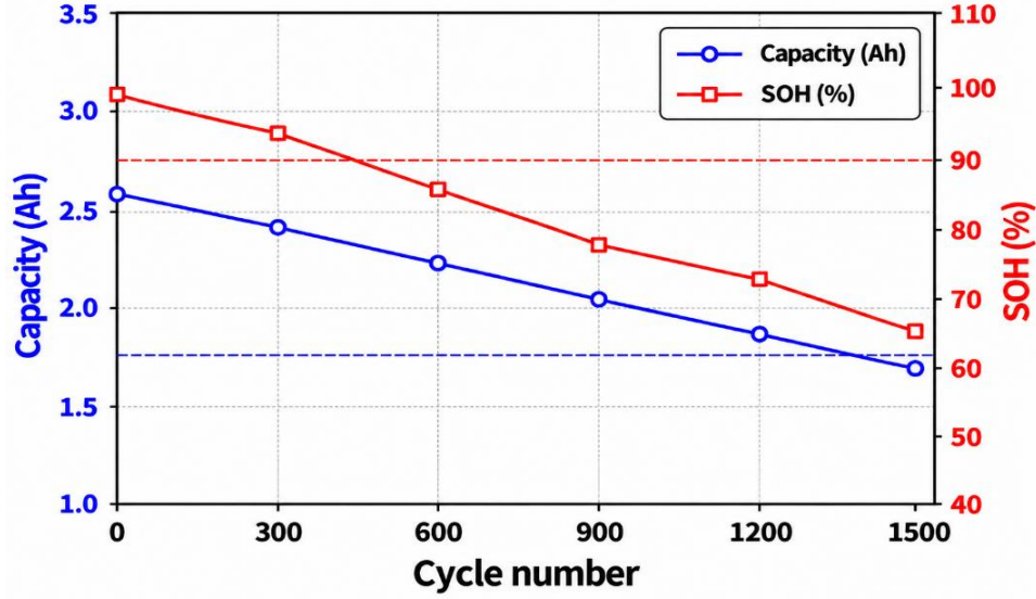
Figure 10 Evolution of discharge capacity and state of health of the lithium-ion cell
