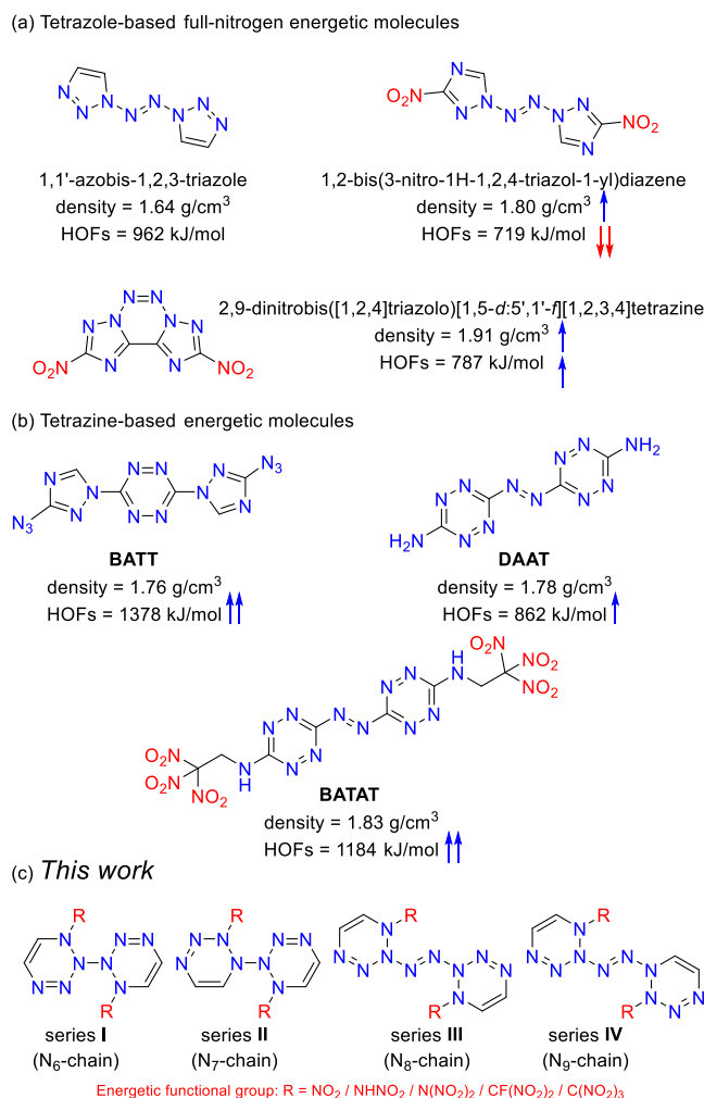
Fig. 1 (a) Tetrazole-based full-nitrogen energetic molecules, (b) Tetrazine-based energetic molecules, (c) The design of energetic materials structures with 1,2,3,4-tetrazine ring as the molecular framework.
