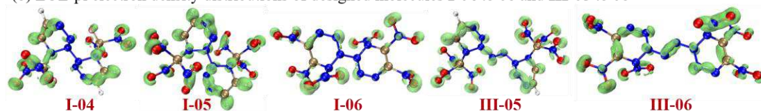
Fig. 5 Electrostatic potential (at M06-2X/6-311+G(d,p) level): (a) ESP map of designed molecule I-04 to 06 and III-05 to 06 , (b) LOL-pi electron density distributions of designed molecules I-04 to 06 and III-05 to 06 .
