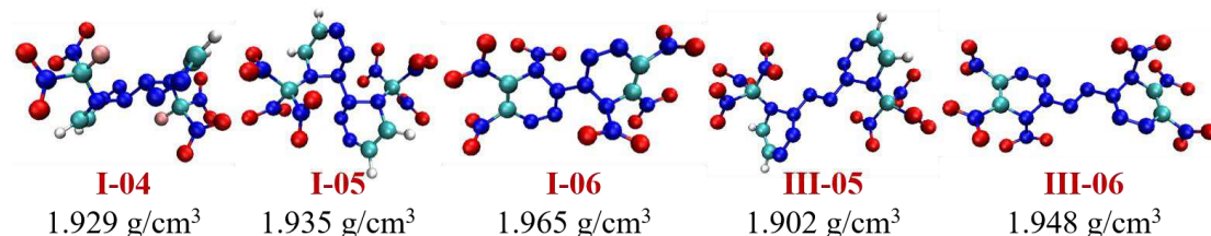
Fig. 2 Molecular optimization structure and density of designed molecule I-04 to 06 and III-05 to 06 at B3PW91/6-311+G(d,p) level
