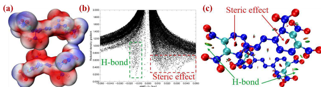
Fig. 6 Study on the weak interactions between molecule III-06 dimer. (a) The ESP map of the optimized III-06 dimer, (b) The NCI scatter graph of the III-06 dimer, (c) The NCI RDG filling map of the III-06 dimer. (at \omega B97X-D/def2tvzp level)
