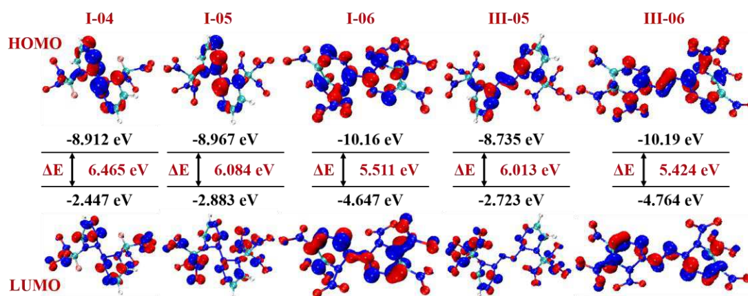
Fig. 3 HOMO and LUMO orbitals map and energy gaps of designed molecule I-04 to 06 and III-05 to 06 at M06-2X/6-311+G(d,p) level
