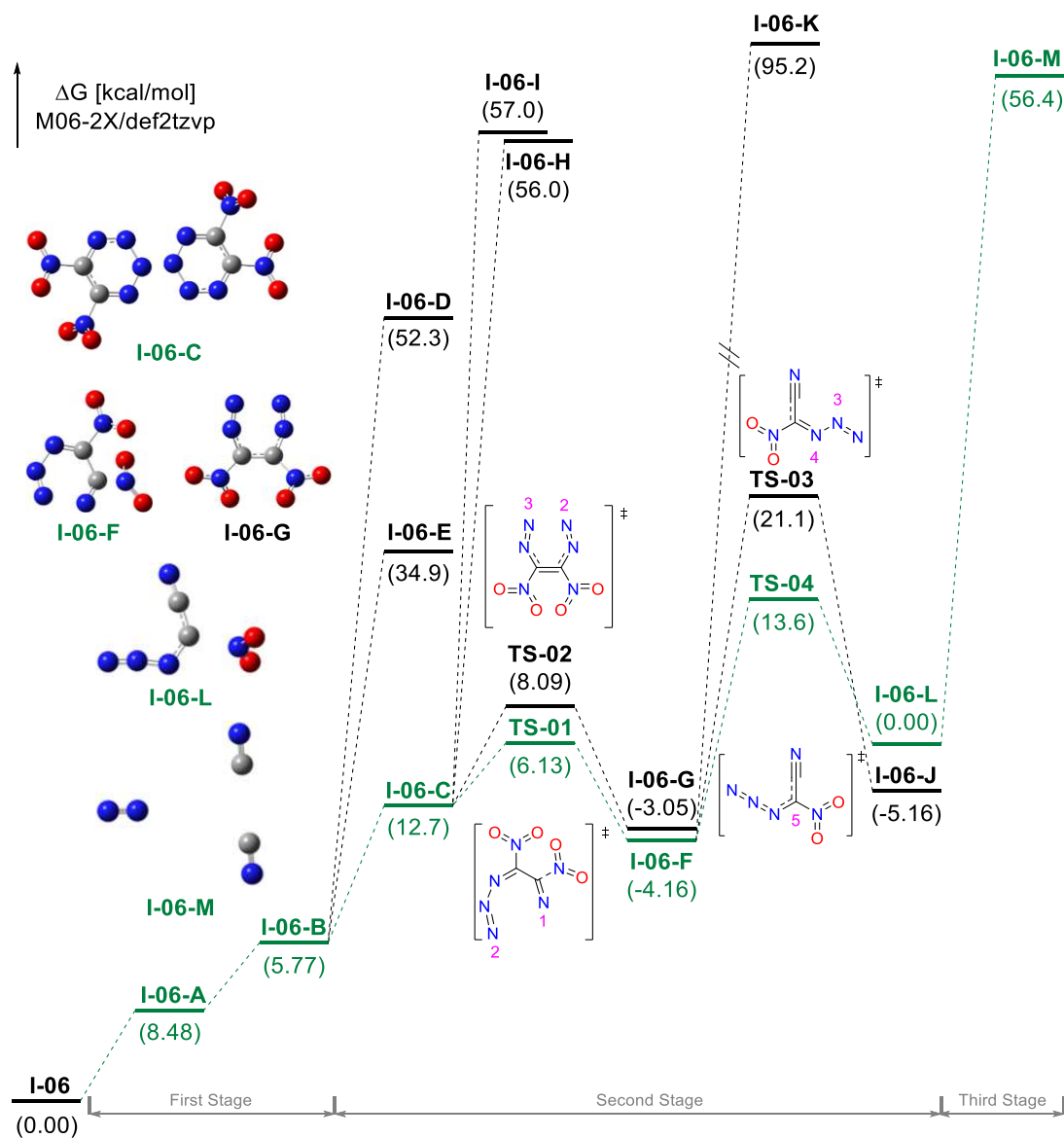
Fig. 7 Possible decomposition pathway of molecule I-06 (at M06-2X/def2tzvp level)
