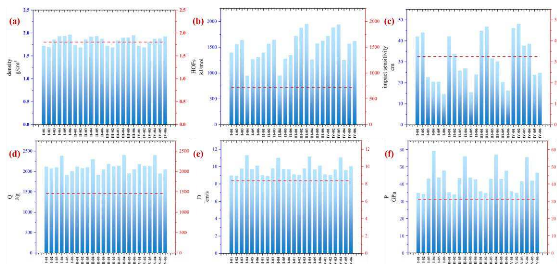
Fig. 4 Detonation properties of the designed molecules, compared with those of compound M02 (red dotted line) at M06-2X/6-311+G(d,p) level. (a) Predicted density value, (b) predicted HOFs value, (c) predicted impact sensitivity ( h_{50} ) value, (d) predicted explosion heat ( Q ) value, (e) predicted detonation velocity ( D ) value, (f) predicted explosion pressure ( P ) value.
