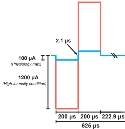
Fig. 4: Accurately scaled stimulation waveforms used for the 100 \mu\text{A} and 1200 \mu\text{A} stimulation paradigms. Waveform parameters consisted of biphasic charge-balanced cathodic leading pulses at 1600 \text{ pps} with a 200 \mu\text{s} phase duration and 2.1 \mu\text{s} inter-phase gap.
