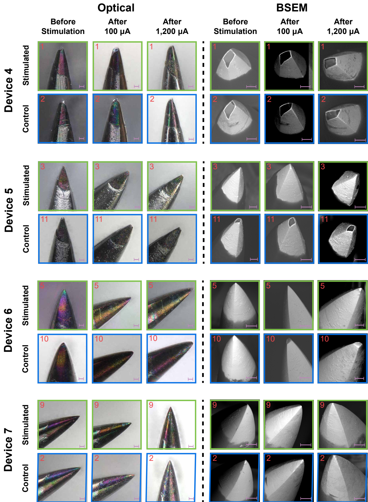
Fig. 9: Representative before and after stimulation optical and electron micrographs from the 100 and 1200 \mu A paradigms, including stimulated and control electrodes, where all scale bars are 10 \mu m. The imaging indicates that neither the paradigm's stimulation intensity was sufficient to produce a measurable impact on electrode metallization, which largely remained unaltered. The stimulated electrode from device 4 presents as a chipped electrode tips before stimulation where a degree of degradation occurs during the 1200 \mu A paradigm resulting in corrosion of the exposed silicon and a small degree of IrOx delamination.
