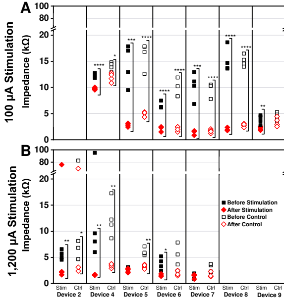
Fig. 10: Before and after impedances from the (A) 100 and (B) 1200 \mu\text{A} stimulation paradigm. In both stimulation conditions, all electrode impedances were initially higher with more variation, which typically decreased to lower to 2-3 k \Omega values with less variation after stimulation. Statistically significant changes from before to after stimulation are identified using standard notation for significance. Stimulated and control categories each had n=4 electrodes.
