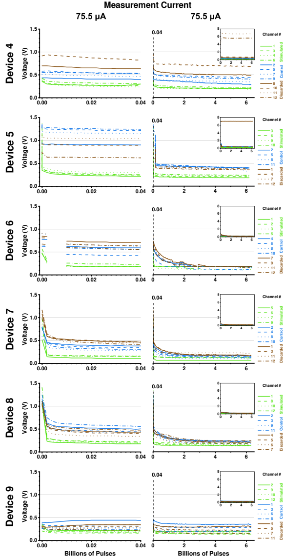
Fig. 11: Longitudinal stimulation voltage data up to 1.5 V for the 100 \mu A paradigm across (left) the initial 40 Mpulses and (right) the full 6.3 Gpulses for each device. Measurements are collected with a 75.5 \mu A current to conform with measurements from Maestro. The inset plot presents voltage data up to 8 V to capture open-circuit or high impedance channels. The traces for channels are categorized by stimulated (green), control (blue), and discarded (brown) for the 12 connected electrodes.
