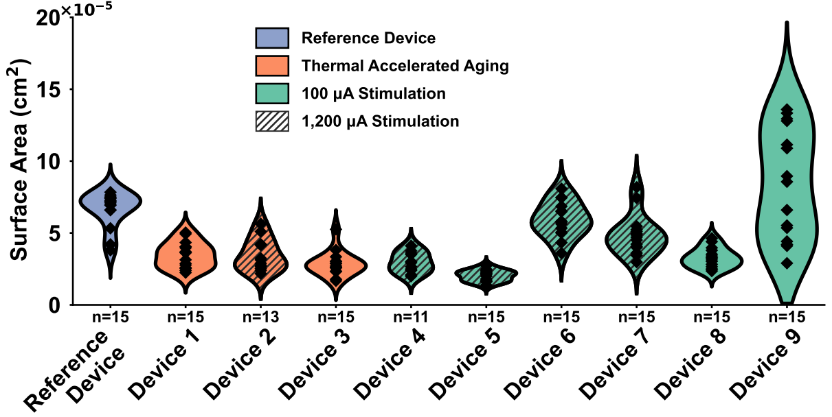
Fig. 5: Electrode tip geometrical surface area for all nine devices and baseline AN-USA assembly are presented as a violin plot. The average geometric surface area was 3.68 \times 10^{-5} \text{ cm}^2 . Color indicates the test protocol each devices was used for, and hatching indicates the five devices that underwent the additional 1200 \mu\text{A} stimulation paradigm.
