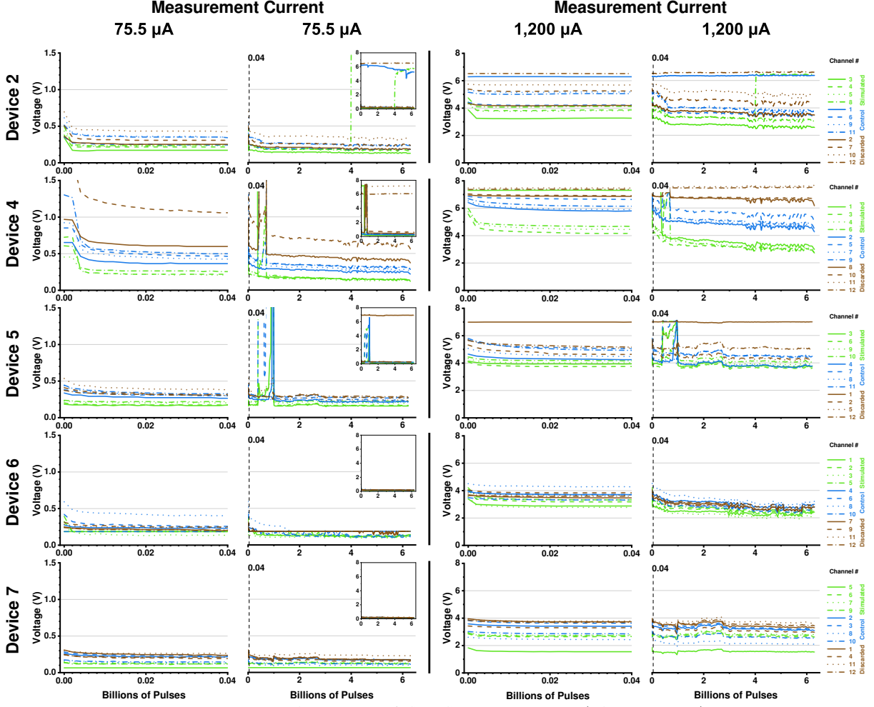
Fig. 12: Longitudinal stimulation voltages for the 1200 \mu\text{A} Stim-Stab paradigm with (left two columns) measurements collected using 75.5 \mu\text{A} pulses and (right two columns) 1200 \mu\text{A} pulses for each device. The plots measured with 75.5 \mu\text{A} facilitate observing abrupt voltage increases, while measurements using the actual 1200 \mu\text{A} stimulation intensity highlight the substantial driving voltages required during the paradigm for some devices. Each measurement condition include plots across 40 Mpulses and 6.3 Gpulses, and the 75.5 \mu\text{A} plot includes an inset that presents voltage data up to 8 V to capture open-circuit or high impedance channels. The traces for channels are categorized by stimulated (green), control (blue), and discarded (brown) for the 12 connected electrodes.
