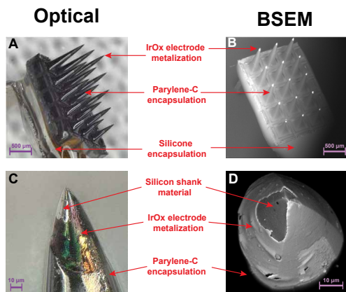
Fig. 2: Representative optical and backscattered scanning electron microscopy (BSEM) micrographs, presenting (A) an overview optical and (B) overview BSEM micrographs of AN-USA showing all 15 electrodes. (C) Higher magnification optical (500 \times ) and (D) BSEM (1250 \times ) micrographs of electrode tip. Red call-outs identify locations and contrast mechanisms associated with IrOx, Parylene-C, silicone, and silicon.
