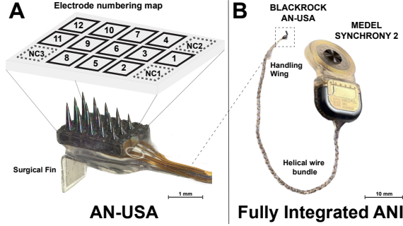
Fig. 1: Overview images of the ANI device including an (A) optical micrograph of the AN-USA electrode array and a projection of the corresponding electrode mapping. Electrically connected channels are labeled 1-12, while not connected ones are labeled NC1-3. The overmolded Pt-Ir Fin on the array’s backside used for surgical handling is identified. (B) Picture of a fully integrated ANI device comprised of a MEDEL SYNCHRONY2 stimulator connected by the helically wound lead to the Blackrock AN-USA. A silicone Handling Wing located 10 mm proximal to the array is labeled.
