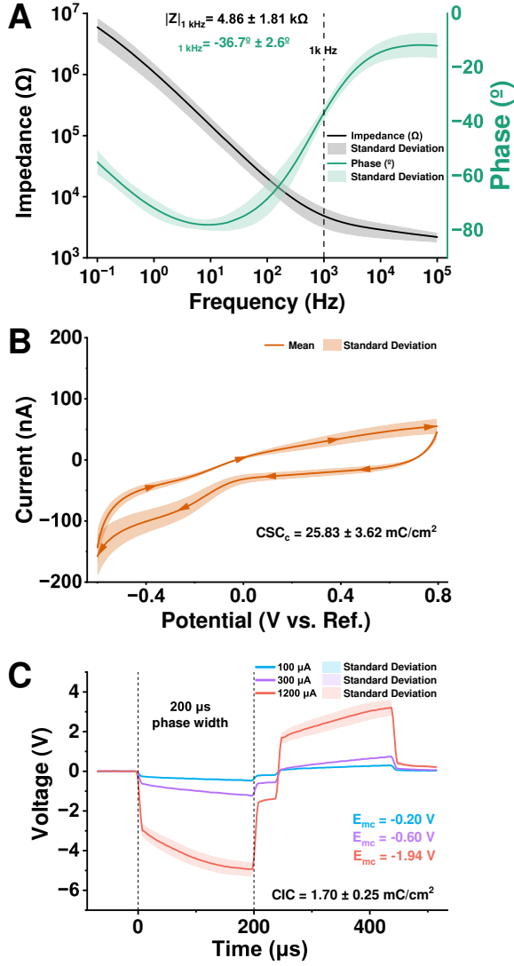
Fig. 6: Electrochemical characteristics of reference ANI assembly electrodes ( n=8 ). A) Electrochemical impedance spectroscopy (EIS) as a combined Bode plotted with average magnitude and phase as a function of frequency, with a 1 kHz the impedance of 4.86 \pm 1.81 \text{ k}\Omega and phase of -36.7 \pm 2.6^\circ . B) Averaged cyclic voltammetry (CV) waveform of potential sweeps within water window -0.6 to +0.8 \text{ V} vs \text{Ag—AgCl} , used to quantify a \text{CSC}_c of 25.83 \pm 3.62 \text{ mC/cm}^2 . C) Average voltage transient (VT) for the 100 \mu\text{A} (blue) and 1200 \mu\text{A} (red) stimulation conditions. A 300 \mu\text{A} (purple) waveform is shown where E_{mc} reached the water window ( -0.6 \text{ V} vs \text{Ag—AgCl} ) used to quantify an average \text{CIC} of 1.70 \pm 0.25 \text{ mC/cm}^2 .
