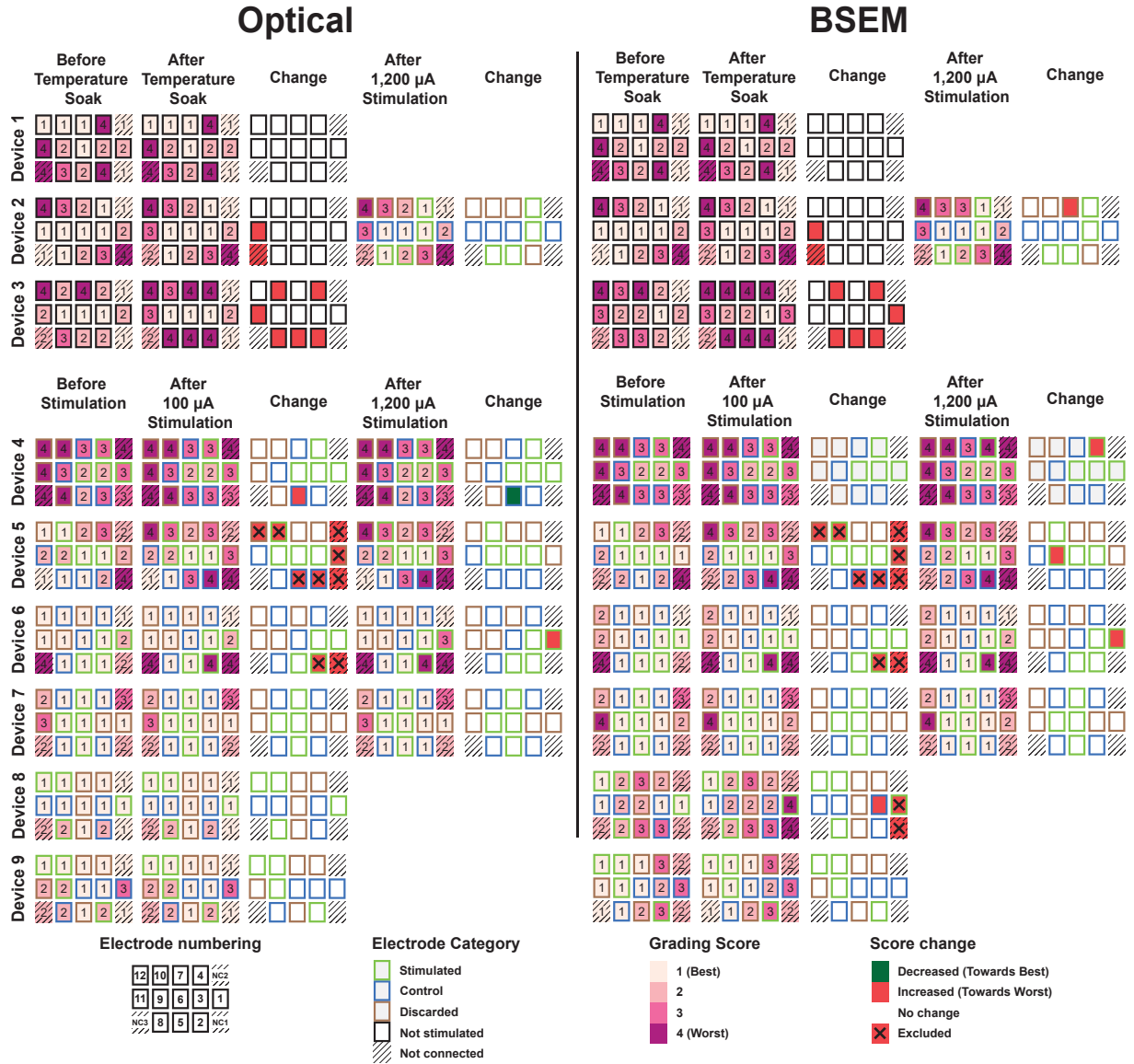
Fig. 8: Heatmaps of scores from 1 = Best (light pink) to 4 = Worst (dark pink) based on (left) optical and (right) electron imaging from before and after all testing paradigms. Electrode numbering for stimulated paradigm devices follows the same convention as Figure 1a and is schematically provided. Border colors represent stimulated electrodes (green), control (blue), discarded (brown), not stimulated (black), and not connected (hatched). Heatmaps quantifying the score Change during a paradigm use green squares to indicate a decreased score, red for an increase, and red with an X for an excluded electrode due to handling damage. All electrode micrographs can be found in supplemental materials S5-S13 .
