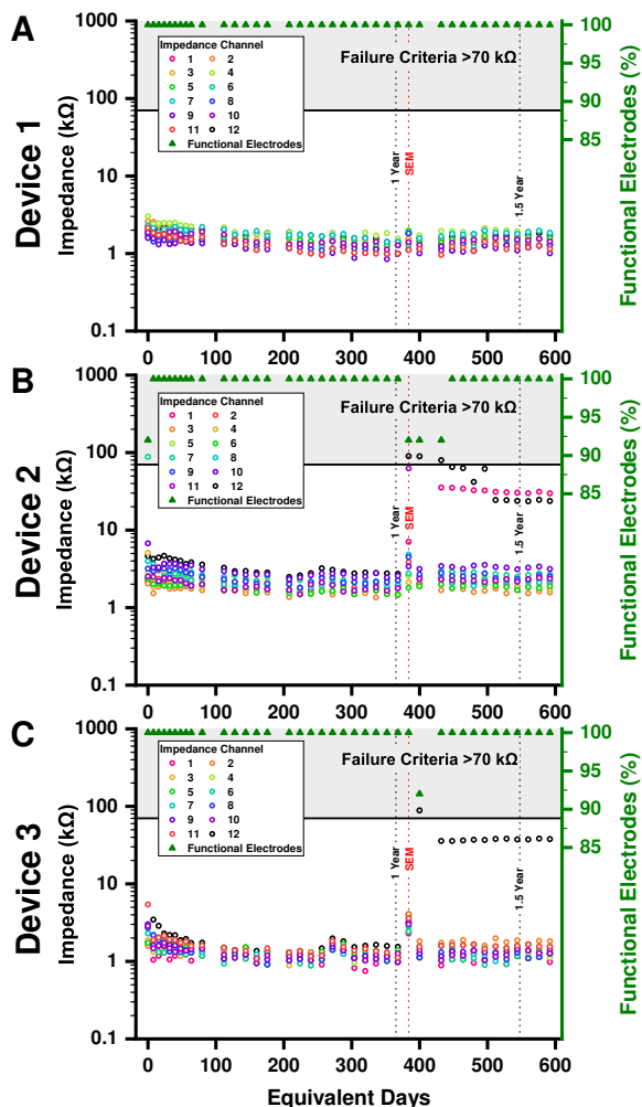
Fig. 7: Thermal Accelerated Aging (TAA) longitudinal impedances plotted for an equivalent 1.5 years, where all electrodes remained below 70 kΩ failure criteria at the endpoint. A) Device 1 electrodes had steady impedances with an average 1.54 \pm 0.20 kΩ, similar for all devices, while for B) Device 2, electrodes 7 and 12 transiently exceeded 70 kΩ failure criteria before returning to high but passing values, similar to C) Device 3 electrode 12.
