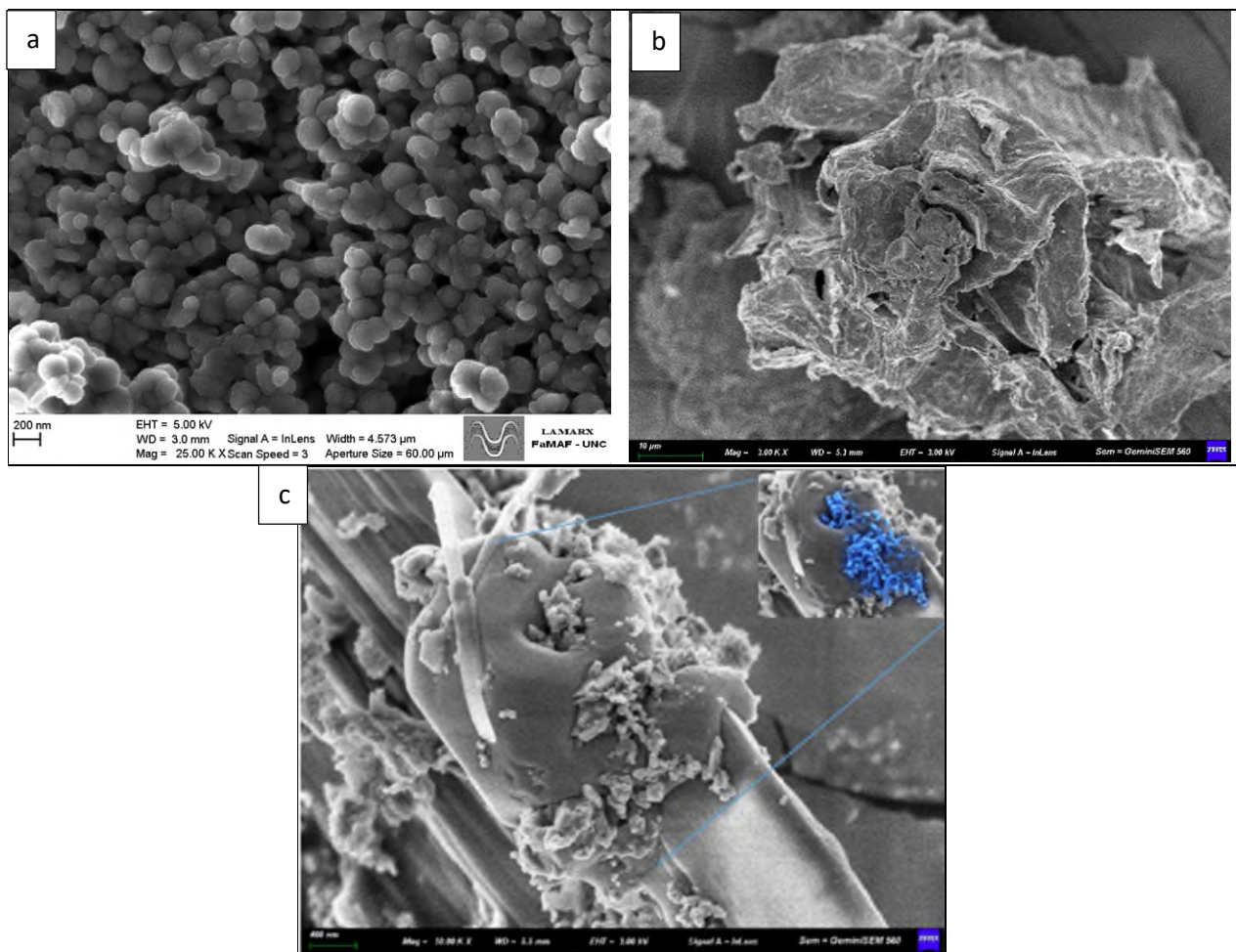
Figure 3. SEM images of: a) MNP, b) biochar and c) BMNP, Inset: magnified view of BMNP with the region containing nanoparticles highlighted in blue
