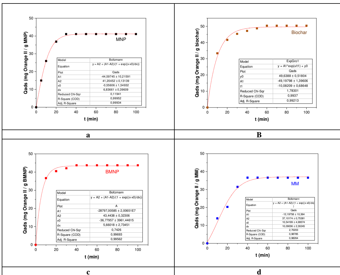
Figure 5. Effect of contact time on adsorption capacity of Orange II for the prepared samples: a) MNP, b) biochar, c) BMNP, d) MM
