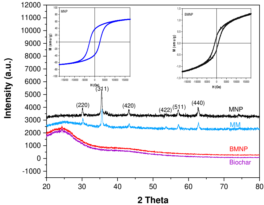
Figure 2. XRD diffraction patterns of biochar, MNP and the biochar-nanoparticle composites. Inset: Magnetic profiles of MNP (left) and BMNP (right)
