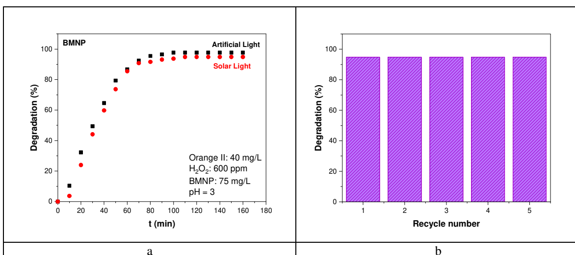
Figure 8. a) Comparison of Orange II degradation vs. time using BMNP as catalyst under artificial light and solar light irradiation; b) Reusability of BMNP (Orange II: 40 mg/L; catalyst: 75 mg/L; H 2 O 2 : 600 ppm; pH = 3; solar light irradiation)
