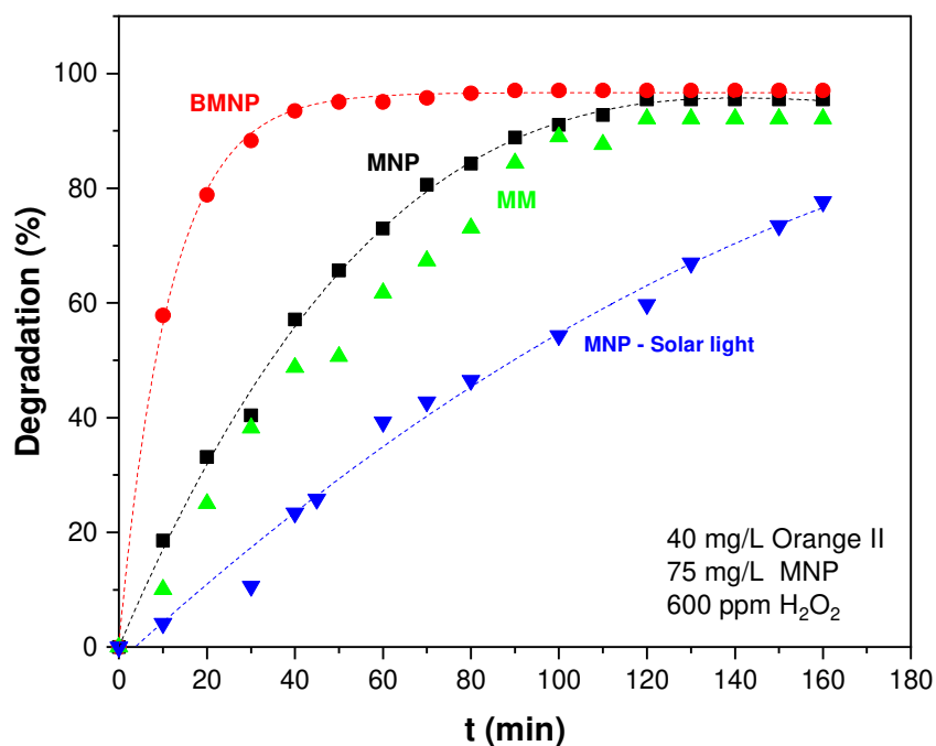
Figure 7. Comparison of Orange II degradation vs. time using MNP, BMNP and MM as catalysts under artificial light and MNP under solar light (Orange II: 40 mg/L; catalyst: 75 mg/L; \text{H}_2\text{O}_2 : 600 ppm; pH = 3)
