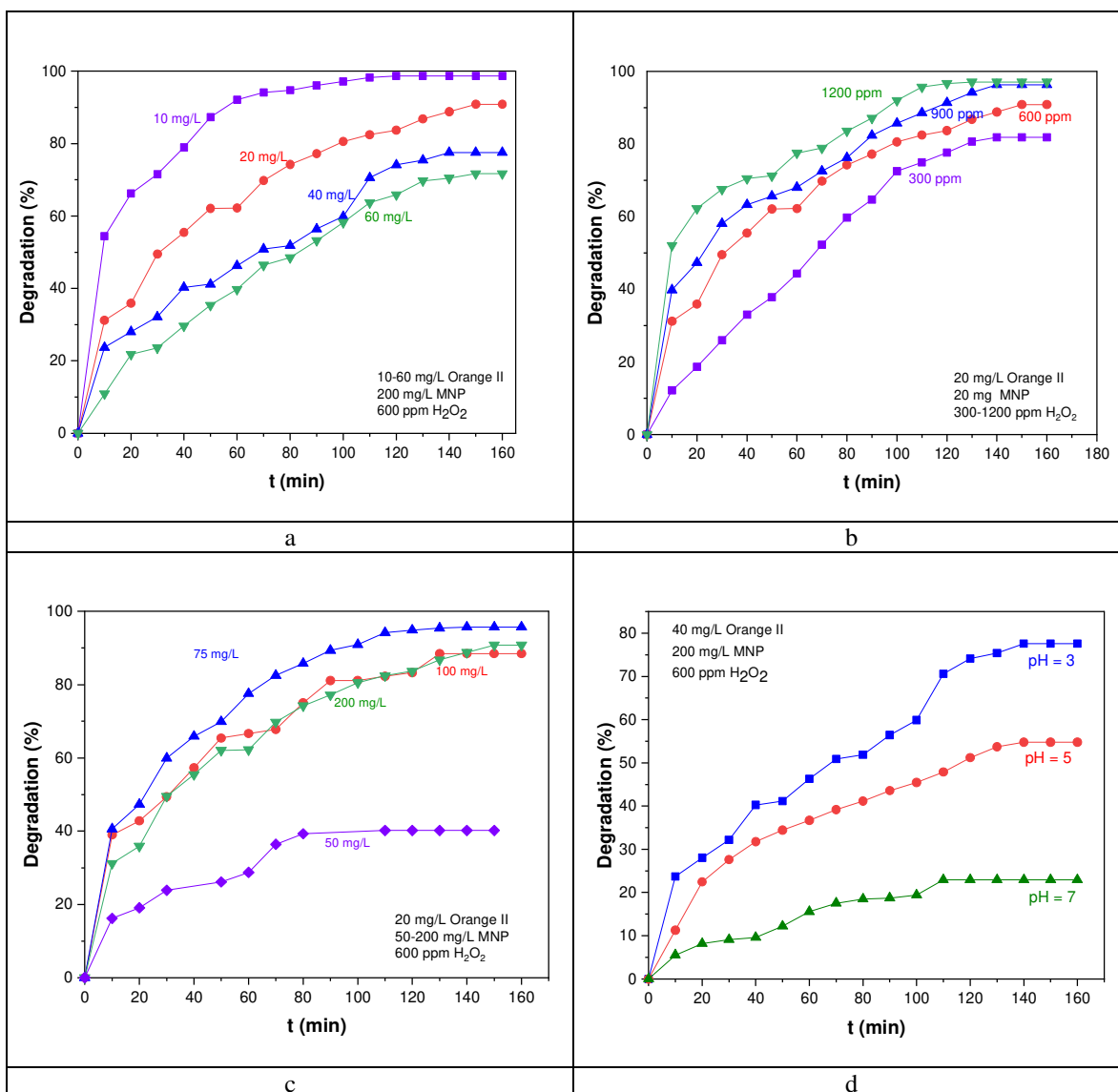
Figure 6. Degradation (%) of Orange II as a function of: a) dye concentration; b) H 2 O 2 dosage; c) catalyst dosage; d) initial pH
