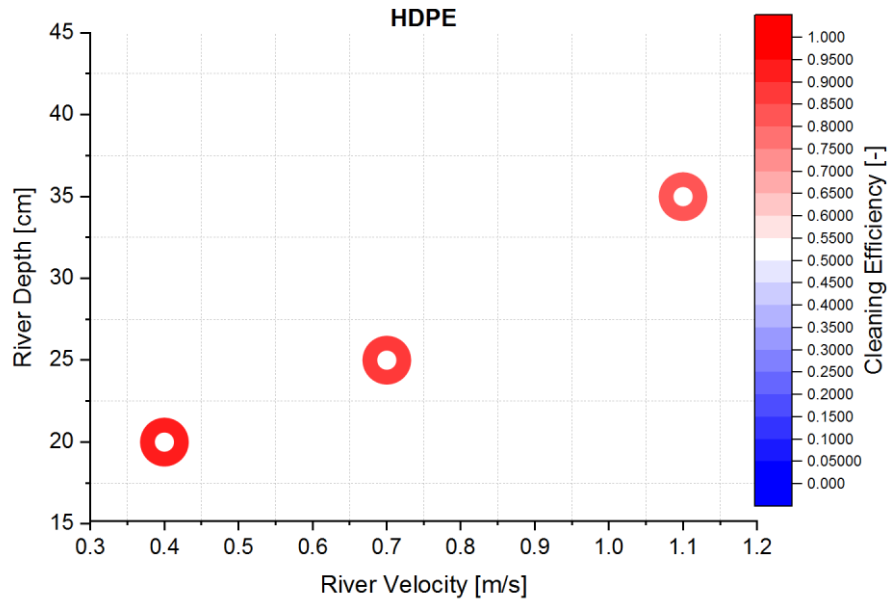
Fig. 21 Cleaning efficiency for HDPE waste at a specific river velocity and depth
