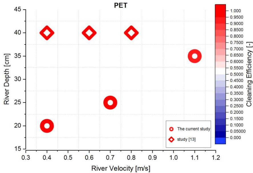
Fig. 27 Comparison of cleaning efficiency for PET waste
