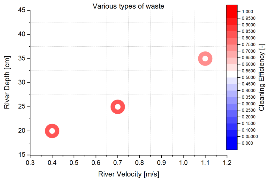
Fig. 18 Cleaning efficiency for Various Types of Waste (Table 1)
