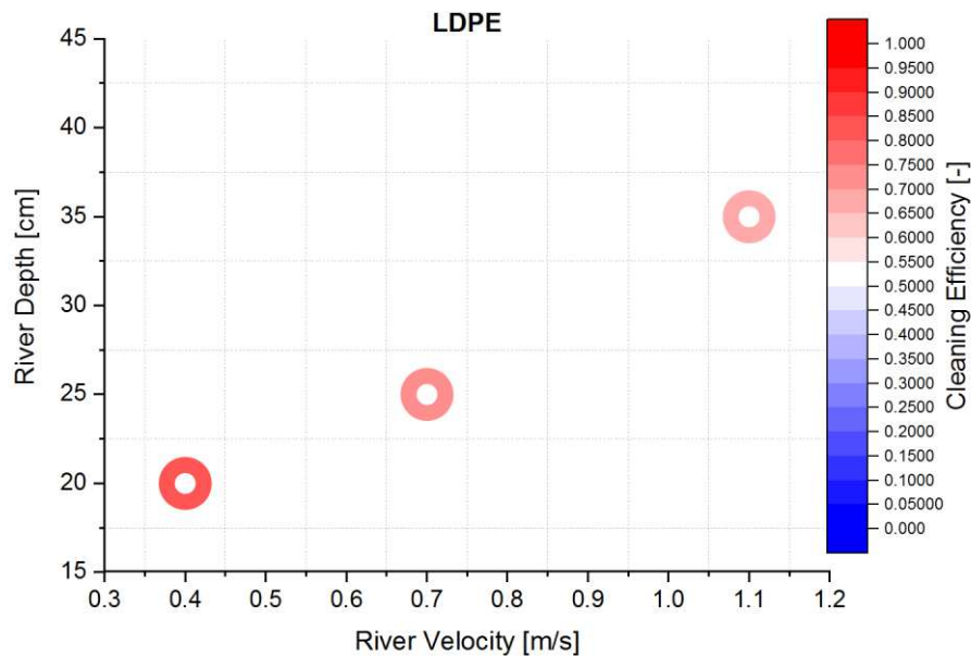
Fig. 20 Cleaning efficiency for LDPE waste at a specific river velocity and depth
