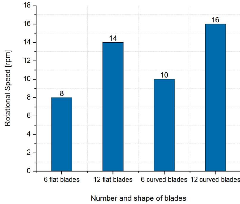
Fig. 17 Rotational speed of the rotating wheel at a flow velocity of 0.4 m/s
