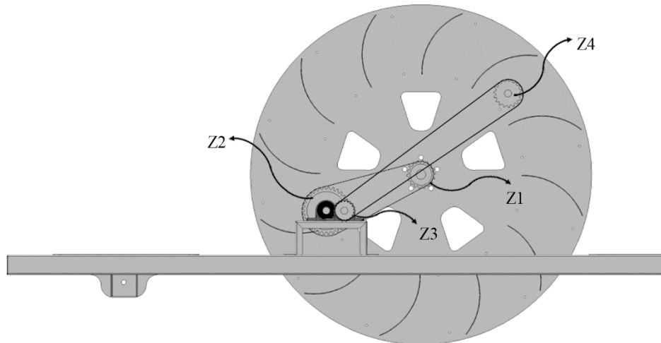
Fig. 2 The gears implemented 138 139 140
