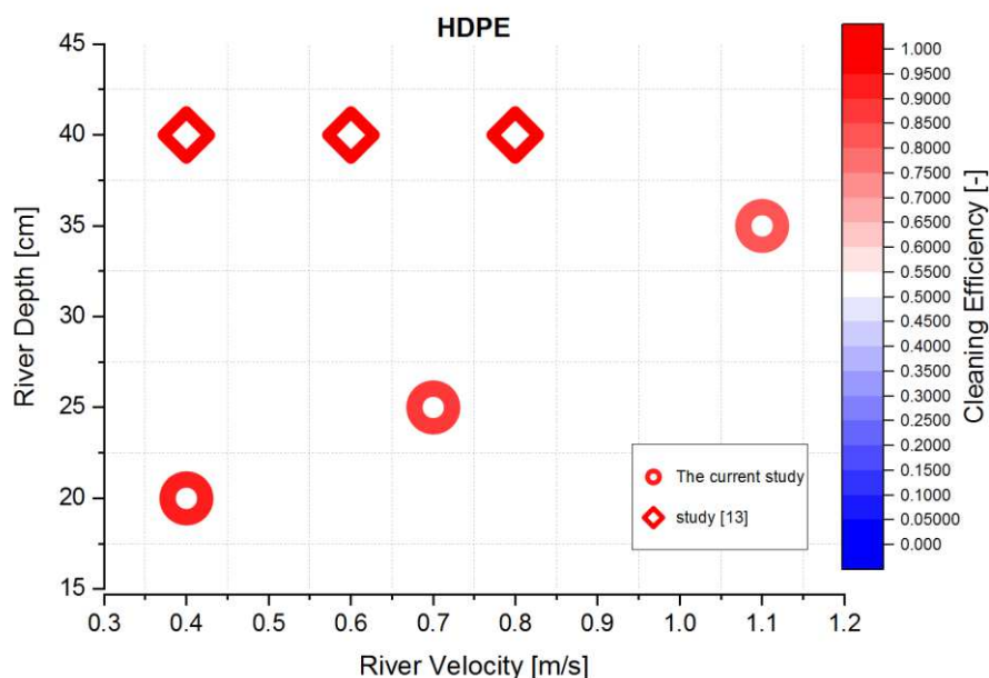
Fig. 25 Comparison of cleaning efficiency for HDPS waste
