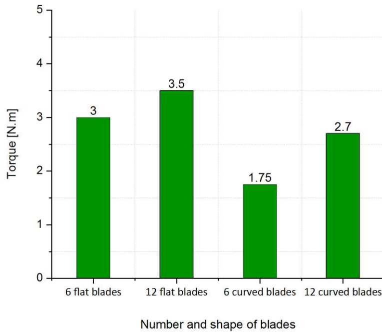
Fig. 16 The torque of the rotating wheel at a river flow velocity of 0.4 m/s
