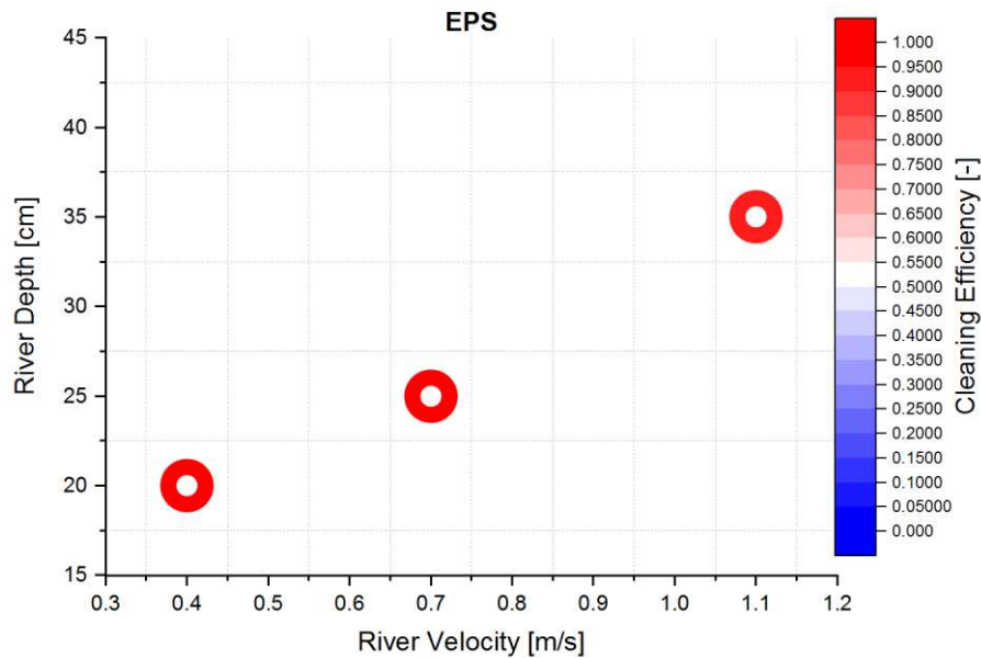
Fig. 22 Cleaning efficiency for EPS waste at a specific river velocity and depth
