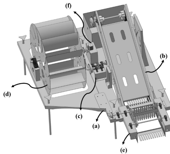
Fig. 1 Engineering Drawing, (a) Main Structural Frame, (b) Conveyor Belt System, (c) Direction Reversal and Torque Transmission, (d) Rotary Wheel and Blade Design, (e) Guiding Mechanism, (f) Stopping Mechanism
