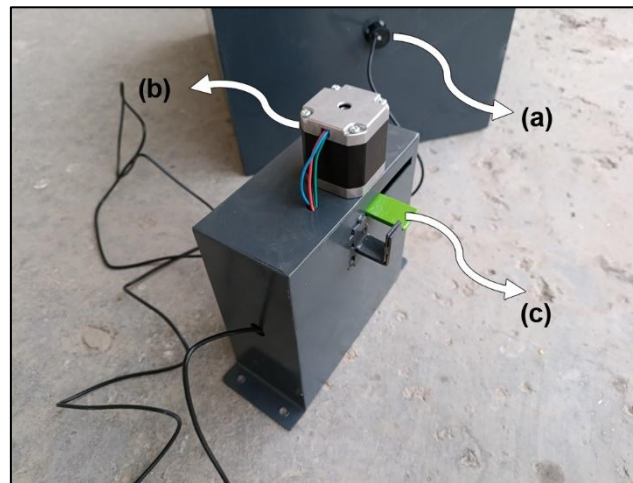
Fig. 4 Stopping mechanism, (a) Sensor, (b) Stepper motor, (c) Latch
