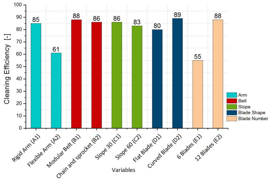
Fig. 15 Individual efficiency of each variable (number of successfully collected residues out of 20 released)
