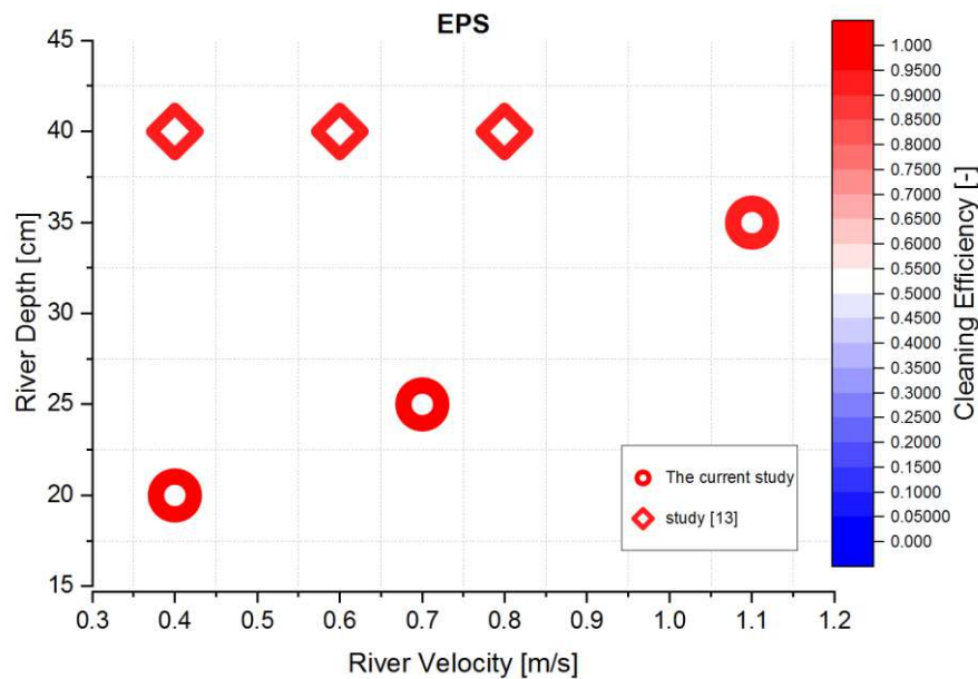
Fig. 24 Comparison of cleaning efficiency for EPS waste
