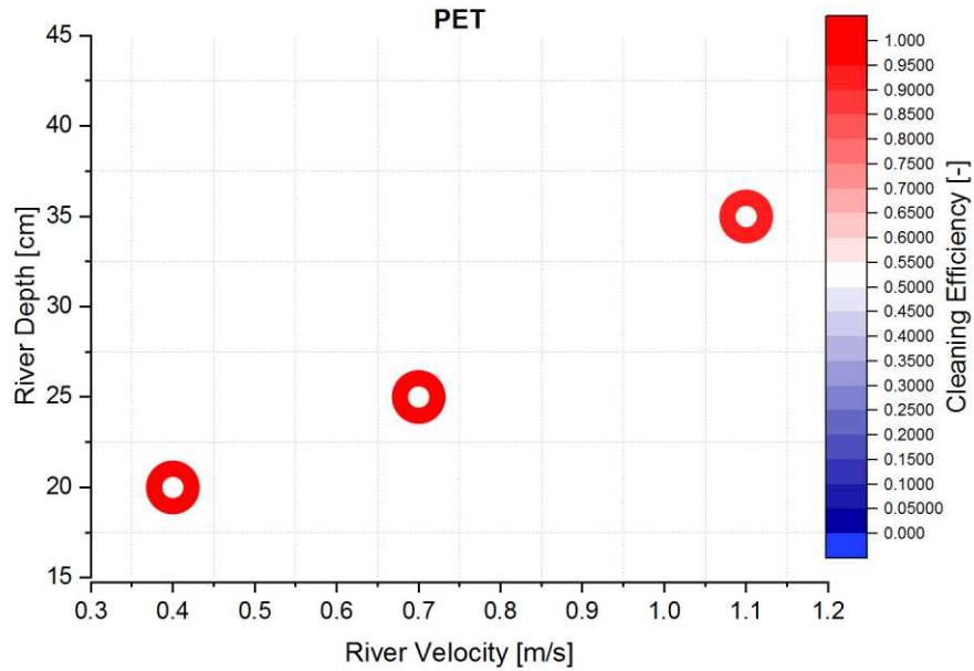
Fig. 19 Cleaning efficiency for PET waste at a specific river velocity and depth
