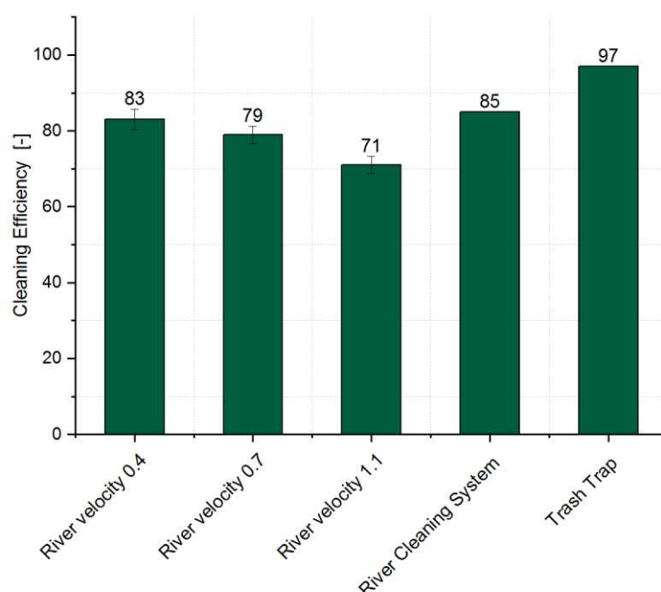
Fig .23 Comparison of cleaning efficiency for various types of waste (Table 1)
