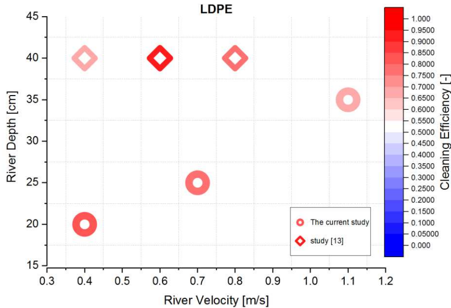
Fig. 26 Comparison of cleaning efficiency for LDPE waste
