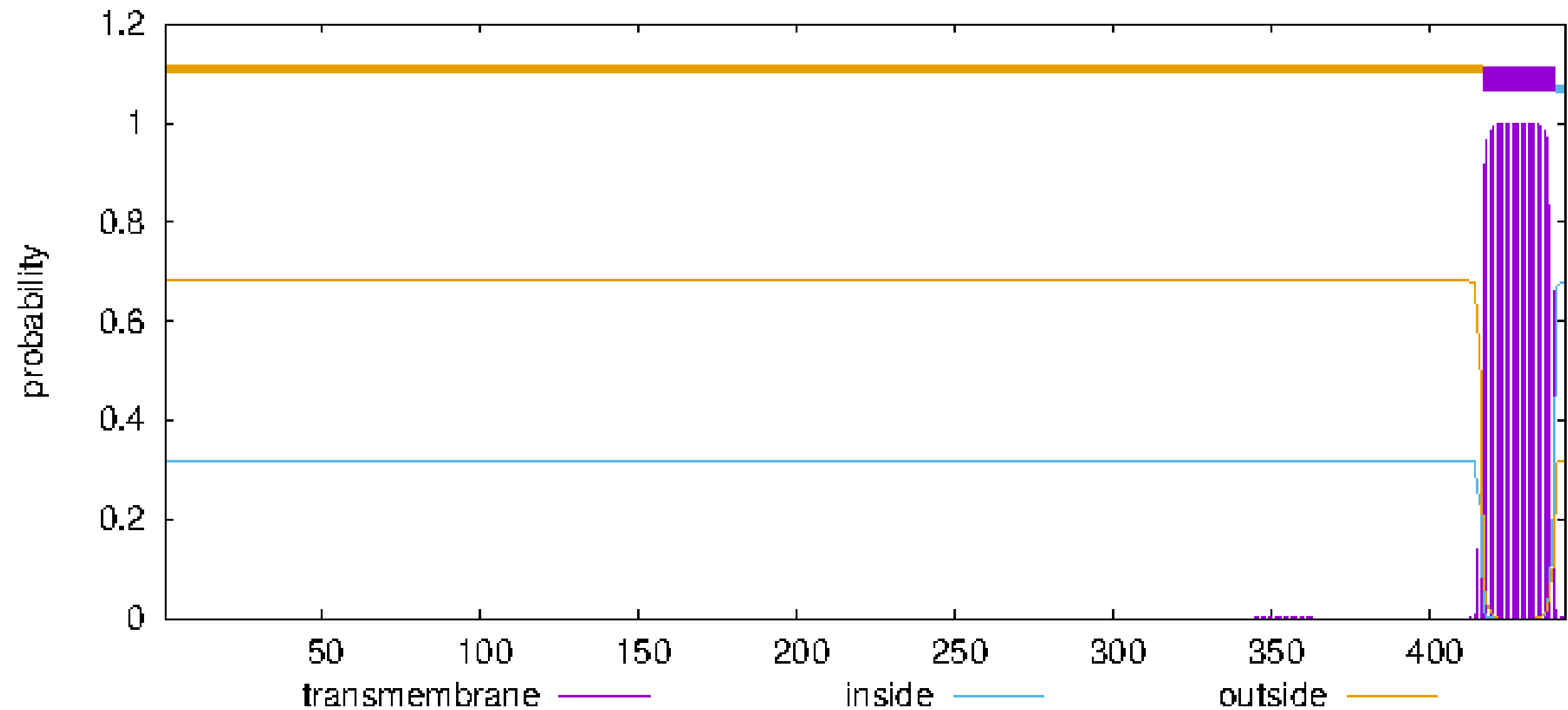
TMHMM posterior probabilities for SINAC38
