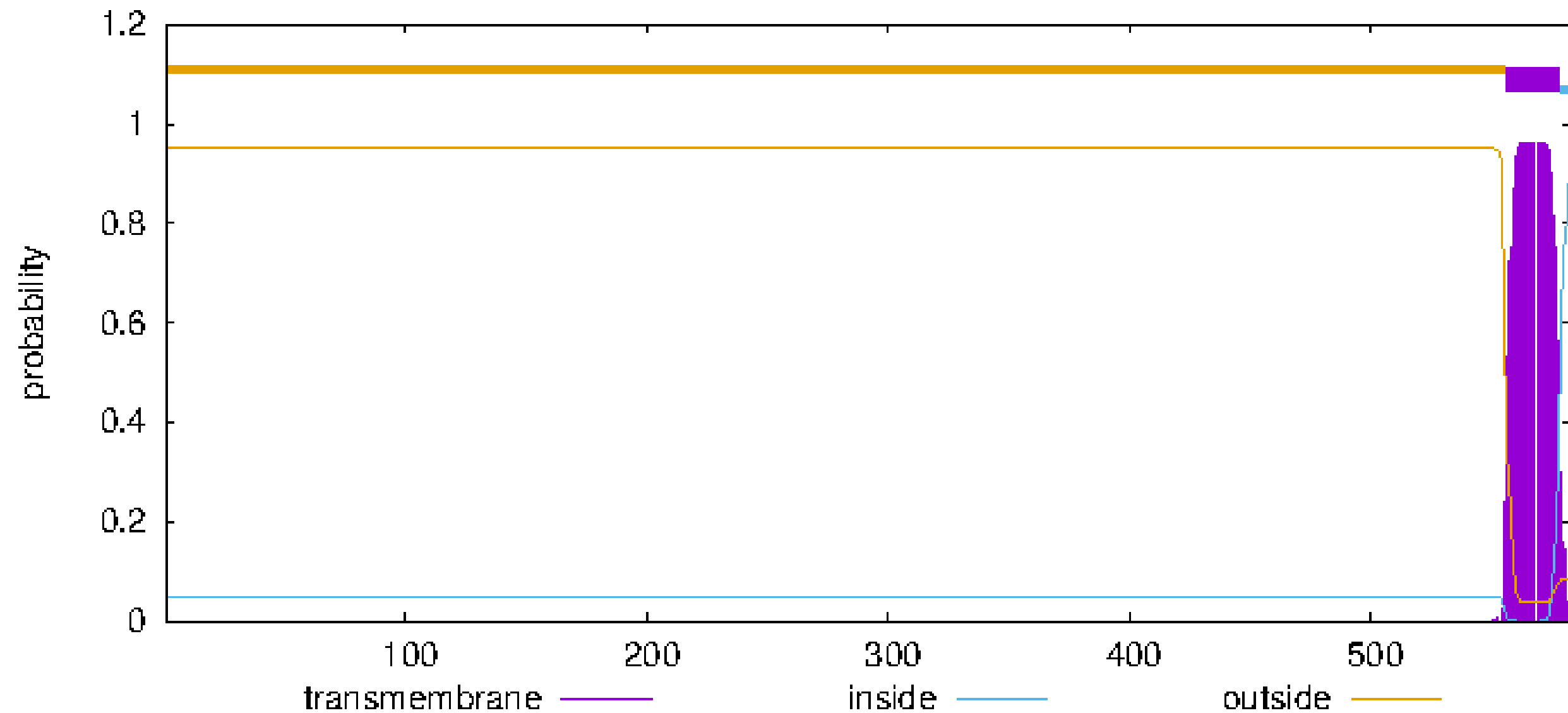
TMHMM posterior probabilities for SiNAC48
