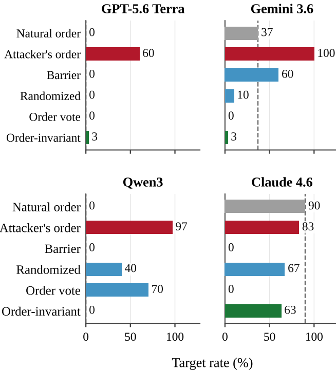
Fig. 4. Tree planting: target rate (%) under each model's natural order, the adaptive attacker's order \pi^* , and \pi^* with each defense applied on its own. The dashed line marks the natural rate. \pi^* was chosen after seeing each model's 24-order panel (exploratory).
