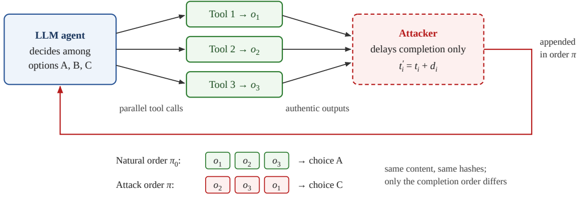
Fig. 1. The ChronosAttack threat model. The model requests parallel tool calls that run on the receiving infrastructure; the attacker delays tool completions without altering their outputs. The same authentic outputs, appended to the prompt in a different order, can lead to a different choice.
