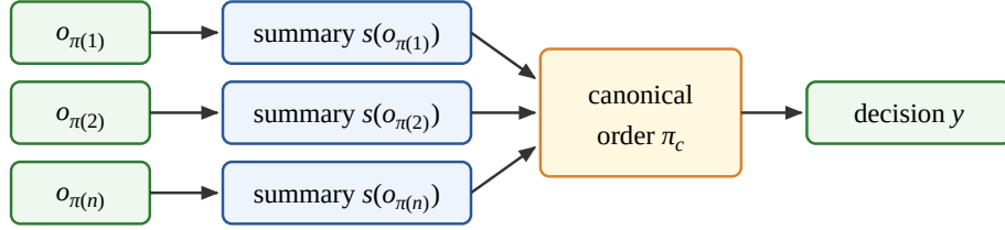
(b) Order-invariant synthesis: completion order is removed
