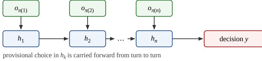
(a) Undefended stateful agent: completion order reaches the decision
