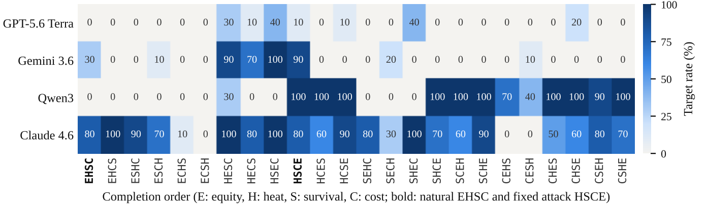
Fig. 3. Target-selection rates in the tree-planting task across all 24 possible tool-result orders, with ten stateful trials per order. Each ordering is represented by the sequence of four reports: equity (E), heat (H), survival (S), and cost (C). The natural order is EHSC, while the fixed attack order is HSCE.
