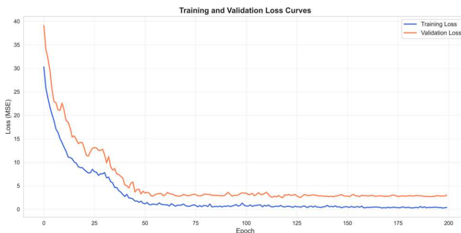
Figure 5. Training and validation loss (summed MSE over both tasks) across 200 epochs. The periodic perturbations in the validation curve correspond to warm restarts of the cosine-annealing learning-rate schedule.
