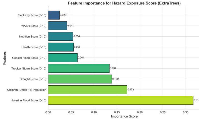
Figure 3a. Extra-Trees feature importance for the Hazard Exposure Score.
