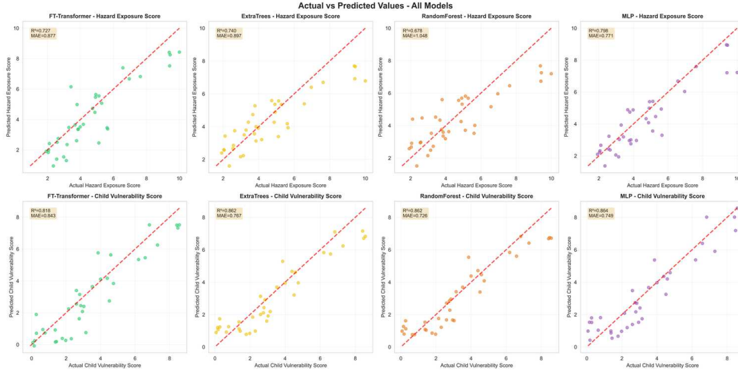
Figure 6. All four major models against both targets with predicted versus observed values. Hashed diagonal line indicates perfect prediction; the boxes in the inset graph report R^2 and MAE per panel.
