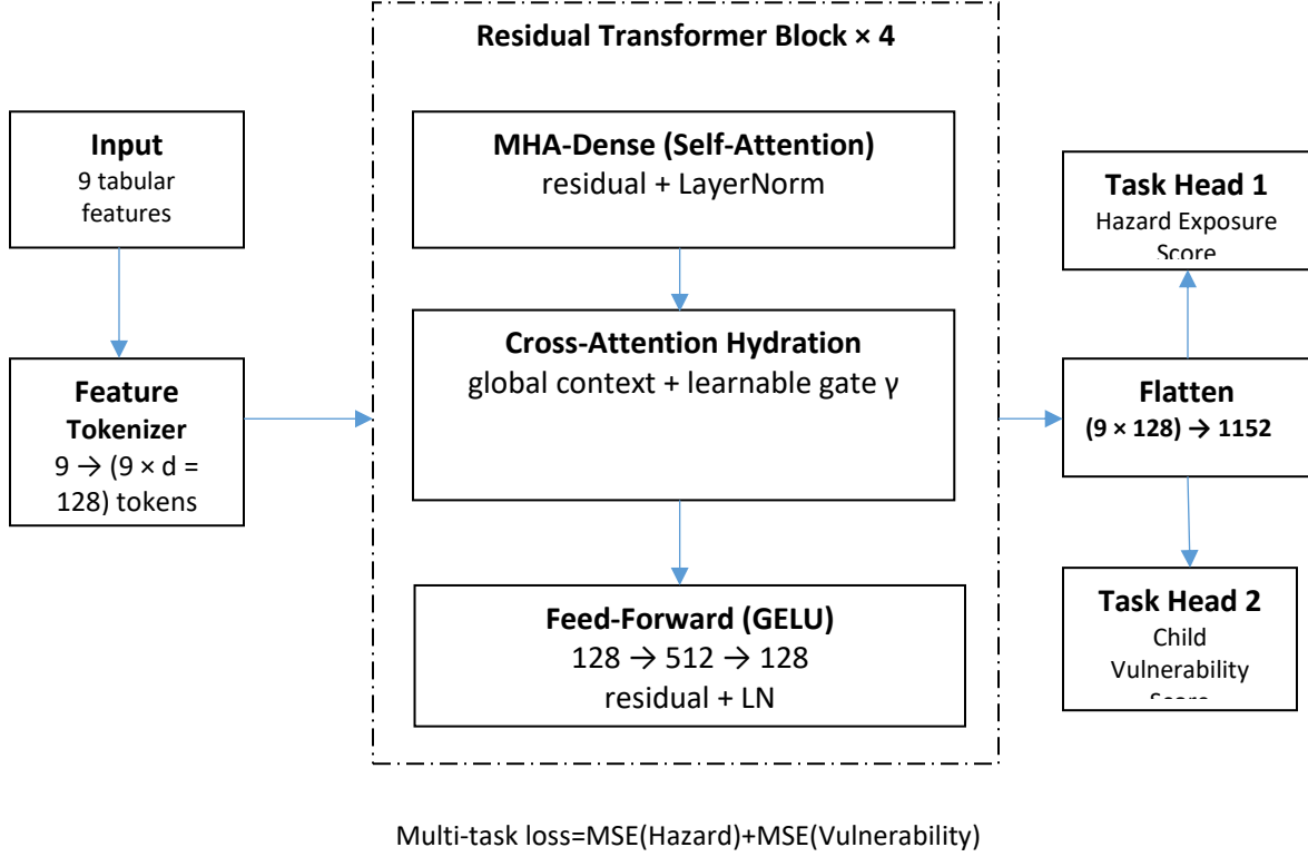
Figure 4. Schematic of the ResNet-FT-Transformer with Cross-Attention Hydration (MHA-Dense). Nine scaled indicators are tokenised into per-feature embeddings, refined by four residual transformer blocks (each combining MHA-Dense self-attention, gated Cross-Attention Hydration, and a GELU feed-forward sub-layer), flattened, and mapped to two scores through dedicated task heads under a summed-MSE objective.
