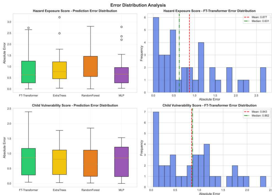
Figure 8. Error-distribution analysis: box plots of absolute error across all models (left column) and the proposed model’s absolute-error histogram (right column) for each target.
