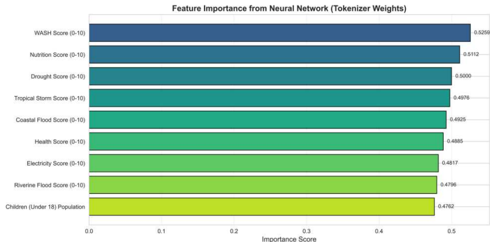
Figure 9. Feature importance derived from the magnitude of the neural feature-tokeniser weights. Larger values indicate features whose learned embeddings more strongly shape the model’s internal representation.
