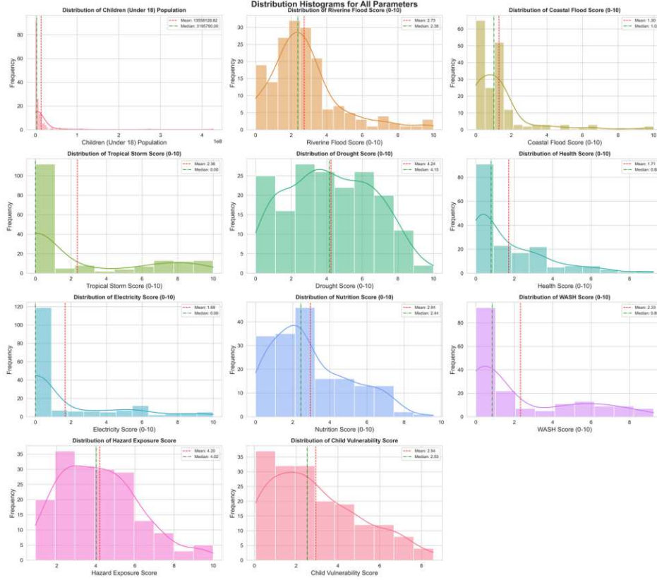
Figure 1. Distribution histograms with kernel-density overlays for all nine predictors and both targets. Dashed and dash-dot lines mark the mean and median of each variable; the separation between them indicates skew.
