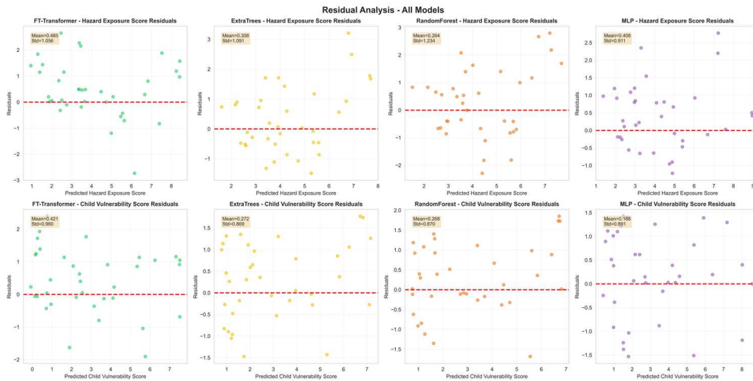
Figure 7. Residuals (observed minus predicted) against predicted values for all four primary models and both targets. Residuals scattered symmetrically about zero indicate well-calibrated central predictions.
