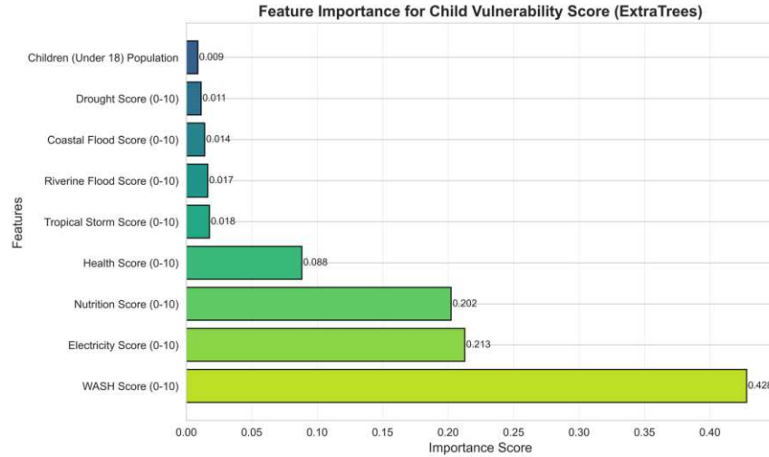
Figure 3b. Extra-Trees feature importance for the Child Vulnerability Score.
