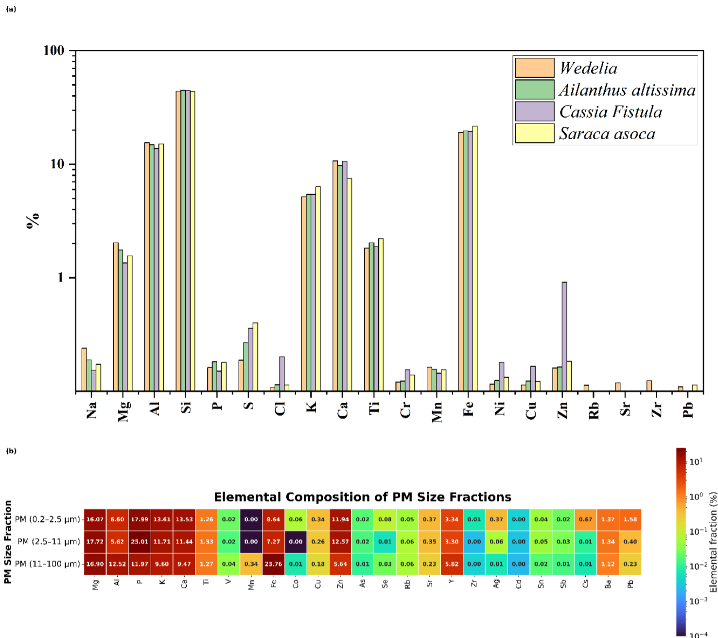
Figure 4 Elemental Composition of PM Across Plant Species and Leaf-Captured Size Fractions (a)Elemental composition of the PM 2.5 fraction deposited on leaves of the selected plant species determined by X-ray fluorescence (XRF) analysis. The relative abundance (%) of major and trace elements associated with the fine PM (0.2-2.5 \mu m) retained on the leaf surfaces of Wedelia , Ailanthus altissima , Cassia fistula , and Saraca asoca is presented, (b) Heatmap illustrating the elemental mass percentages (%) obtained via ICP-MS for acid-digested filter samples retrieved from three size categories (PM 0.2-2.5 , PM 2.5-11 , and PM 11-100 ). The heatmap illustrates the size-specific distribution of significant and trace elements, indicating an abundance of crustal elements (Mg, Al, Ca, and Fe) in larger fractions and relatively elevated levels of traffic and industry-associated trace metals (Cu, Zn, Sb, and Pb) in smaller fractions.
