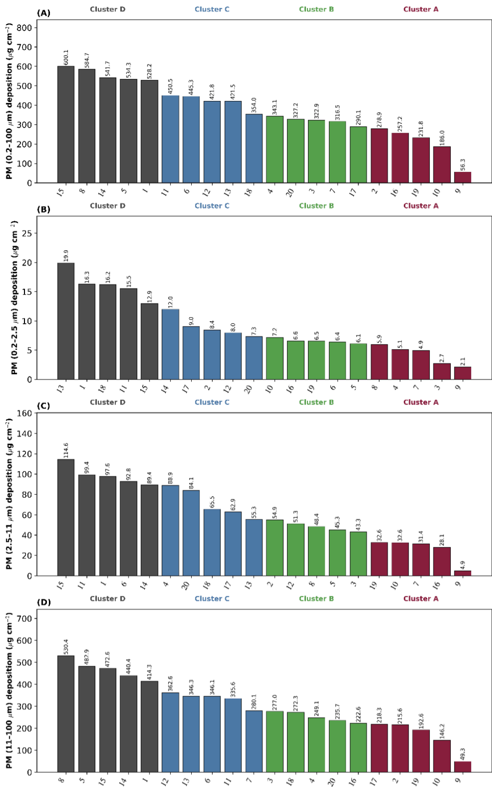
Figure 5 PM deposition capacity of twenty urban plant species at the leaf saturation (threshold) point. The bar plots presents the maximum total PM deposited on leaf surfaces ( \mu\text{g cm}^{-2} )for twenty common urban
