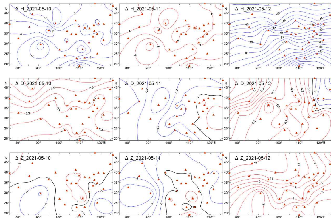
Figure 7 Spatial distribution of \Delta factors in Chinese mainland from May 10 to May 12, 2021
