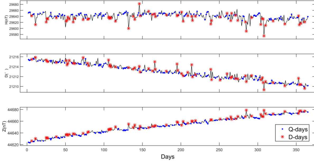
Figure 2 The time-series variation of midnight mean value of LYH observatory in 2021
