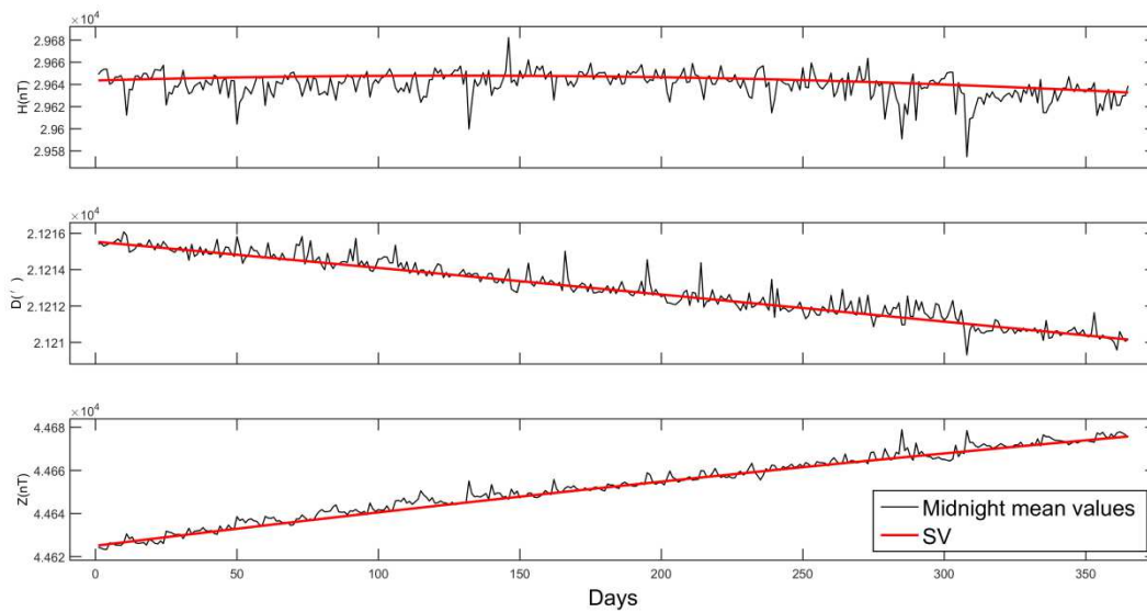
Figure 4 The result of midnight mean value correction
