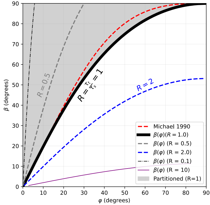
Extended Data Fig.2. Given \beta , \phi , and R (ratio between the average shear stresses on the megathrust ( \tau_t ) versus the strike-slip fault ( \tau_s ) in the upper plate), the analytic model predicts a grey shadowed region above the bold black curve (here assuming R=1 ) as the regime of ‘Partitioned’, in which the combination of obliquity and dip is favorable for the partitioned end-member regime. Hence under the model assumptions, this is a forbidden zone for megathrust earthquakes to exist because the trench-parallel component should be released by strike slip faulting in the upper plate until \alpha is below the ( R=1 ) curve. Note larger R values, indicate a relatively stronger megathrust, and lowering the possible megathrust earthquake slip obliquity.
