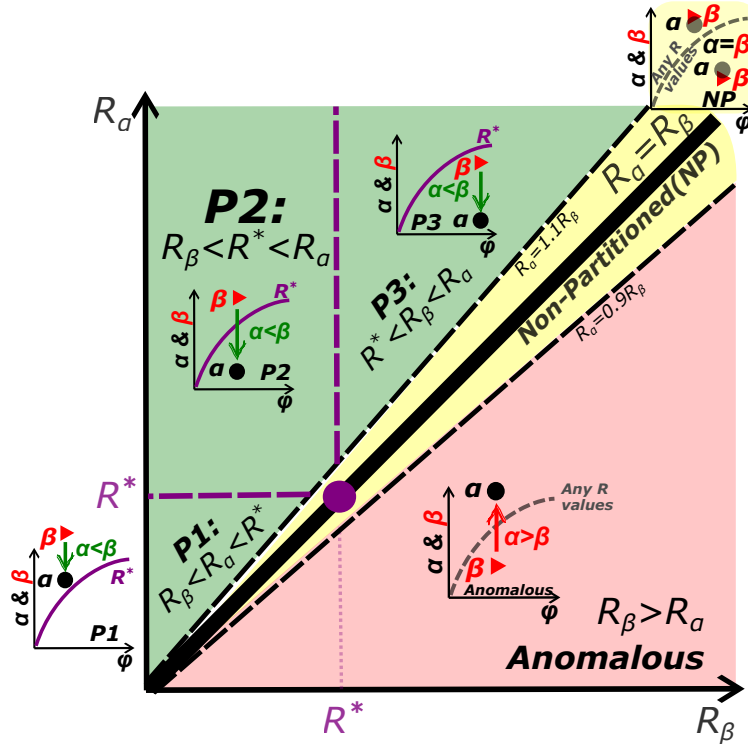
Extended Data Fig.4. Regime diagram. For each megathrust earthquake, given its measured \alpha , \beta and \phi , we can use the close form solution to calculate R_\alpha = \sin \phi / \tan (|\alpha|/2) and R_\beta = \sin \phi / \tan (|\beta|/2) . For each event, we can locate it in the R_\alpha - R_\beta regime diagram, where three major regimes arise: 1) Anomalous (red shaded) when R_\beta > R_\alpha , indicating |\beta| < |\alpha| , which might be due to local heterogeneity (e.g. subducted seamounts); 2) Non-Partitioned (NP, yellow shaded) where R_\alpha \approx R_\beta ( |\alpha| \approx |\beta| ). 3) Partitioned (green shaded) where R_\beta < R_\alpha and |\beta| > |\alpha| .
