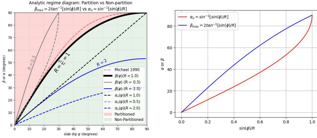
Extended Data Fig.3. Comparing regime boundary \beta_{max}(\varphi, R) (Methods: eq. 4) and \alpha_o(\varphi, R) over meaningful range of \sin \varphi / R .
