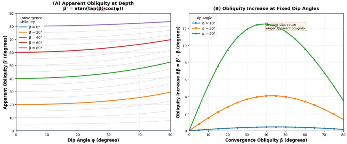
Extended Data Fig.5. Effects of convergence obliquity correction to \beta' as a function of local slab dip \varphi and uncorrected map-view convergence obliquity \beta .
