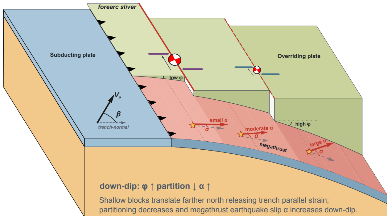
361 Fig. 4 | Schematic strain partitioning between megathrusts and upper plate strike-slip faults at 362 obliquely converging subduction zones. Natural subduction zones commonly have curved megathrusts 363 whose dip \phi increases with depth. In this geometry, shallow forearc blocks tend to be translated in the 364 trench-parallel direction due to upper plate strike-slip faulting. This strike-slip deformation releases much 365 of the trench-parallel component of the oblique plate convergence. The resulting megathrust earthquake 366 slip obliquity \alpha is low. Down-dip, increasing interface dip permits larger megathrust slip obliquity (larger 367 \alpha ).
