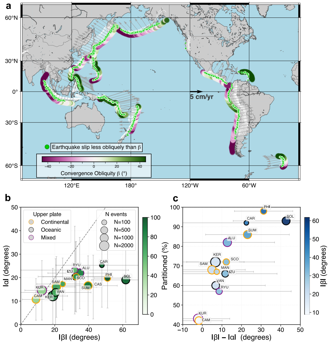
Fig. 1 | Global subduction zone convergence obliquity ( \beta ) versus megathrust earthquake slip obliquity ( \alpha ). a , The green dots in the global map show megathrust earthquakes that slip less obliquely than the local convergence. Plate velocities are calculated by ‘GAGE Plate Motion Calculator’ using GSRM v2.1 7 . Megathrust interface depth contours are from Slab2 8 . Map is plotted with GMT 24 . See SI for detailed maps of each subduction zones. b , Segment-averaged megathrust earthquake slip obliquity |\alpha| versus convergence obliquity |\beta| , colored by the percentage of total number of partitioned events ( \alpha < \beta ) over all thrust events on the megathrust. The dashed line indicates \alpha = \beta . c , Percentage of partitioned events versus difference between |\beta| and |\alpha| , colored by |\beta| . For b & c , circle sizes reflect total number of events considered. Circle outline colors show major upper-plate arc volcanic rock types inferred from Smithsonian Global Volcanism Program volcano rock-type records 25 .
