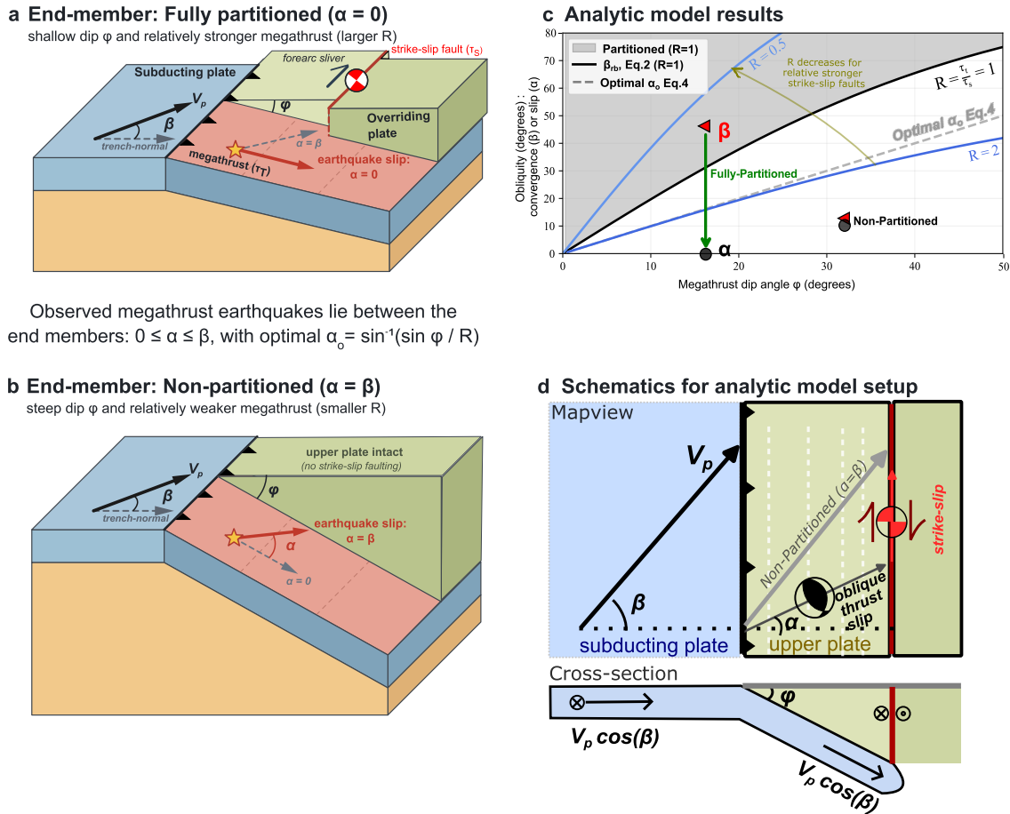
Fig. 2 | Analytic model for limits of megathrust earthquake slip obliquity. a , Fully partitioned end member, in which the trench-parallel component of oblique convergence is fully accommodated by upper-plate strike-slip faulting with average resistance \bar{\tau}_S , resulting in trench-normal ( \alpha = 0 ) earthquake slip on the megathrust interface with average resistance \bar{\tau}_T . This configuration is favored for shallow megathrust dip \phi and/or relatively stronger megathrust resistance, corresponding to larger R = \bar{\tau}_T / \bar{\tau}_S . b , Non-partitioned end member, in which the upper plate remains intact, and the megathrust accommodates all trench-parallel component of the oblique convergence ( \alpha = \beta ). This configuration is favored for steeper megathrust dip and/or relatively weaker megathrust, corresponding to smaller R . c , Given \phi and R , the analytic model predicts a ‘Partitioned’ regime shown as the grey shaded region above the regime boundary \beta_{rb} (Eq.2 assuming R=1 ). This ‘Partitioned’ regime is a forbidden zone for megathrust earthquake slip obliquities ( \alpha ) because when convergence obliquities \beta are above the obliquity limit \beta_{rb} , the trench-parallel strain is predicted to be preferentially released by strike-slip faulting in the upper plate until the remaining trench-parallel strain results in a megathrust earthquake slip obliquity \alpha below the regime boundary \beta_{rb} . Note that larger R values indicate relatively stronger megathrust and lowering the maximum possible megathrust earthquake slip obliquity \alpha . Two end member scenarios are illustrated with the schematic pairs: red triangles for convergence obliquities \beta and the associated black circles for the slip obliquities \alpha at the same dip angles of 16 or 32 degrees. d , Schematic analytic model setup in mapview and cross-section view. The megathrust earthquake slip obliquity is \alpha , convergence obliquity is \beta and the dip angle of the subduction is \phi . Partitioning transfers part of the trench-parallel component to upper-plate strike-slip faulting.
