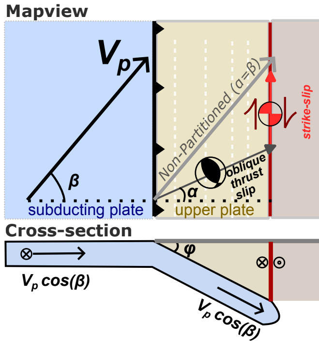
Extended Data Fig.1. Mapview and cross-section view of a simplified oblique subduction zone. The oblique motion can be partitioned into pure normal and upper plate strike-slip motions or solely accommodated on the subduction interface by oblique thrusting. The convergence obliquity is \beta and the dip angle of the subduction is \phi .
