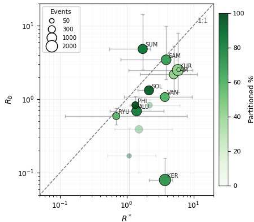
Extended Data Fig.6 | Correlation between the inferred R^* ( R^{\#} here) in the framework of the analytic model (Methods: M1.6 & M2.6) and the b-value-derived stress ratio R_b (Methods: M2.9). Horizontal bars show the R^* range capturing 90% of partitioned events, and vertical bars show the 16–84% uncertainty range of R_b . Symbol size scales with the number of megathrust earthquakes analyzed, and color indicates the percentage of partitioned events. Faded symbols indicate computed but weakly constrained R_b estimates due to low event counts or uncertain completeness magnitude (see Methods: M2.9).
