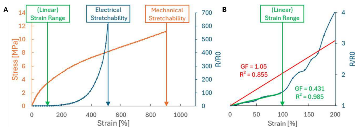
Figure S1. (A) Sensing behavior comprises the mechanical (stress, orange) and electrical (normalized resistance, blue) behavior 27 . When stretchability is reported, it might refer to mechanical stretchability (maximum observable strain before mechanical fracture) or electrical stretchability (maximum observable strain before an electrical open circuit, e. g. due to fracture of the percolation network). (B) When considering the inherently non-linear electrical behavior, a smaller strain range can be defined where the electrical behavior is sufficiently linear (e.g. R^2 above 0.98), giving the linear strain range. For comparison, the linear fitting of the same curve for less stringent linearity ( R^2 above 0.85) is represented in red, demonstrating larger strain range and sensitivity.
