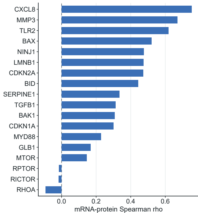
b Per-gene mRNA-protein concordance
