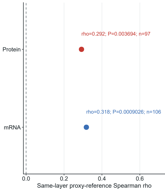
a Partial-panel covariance
