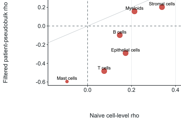
c Legacy coupling is null after BH correction
