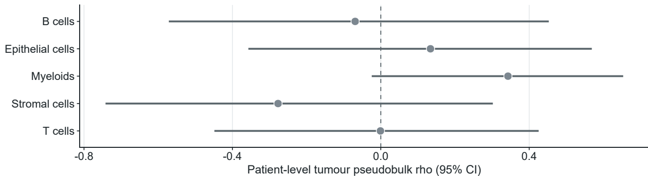
c Legacy coupling is null after BH correction
