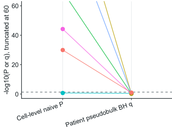
b Cell-level P values are anti-conservative
