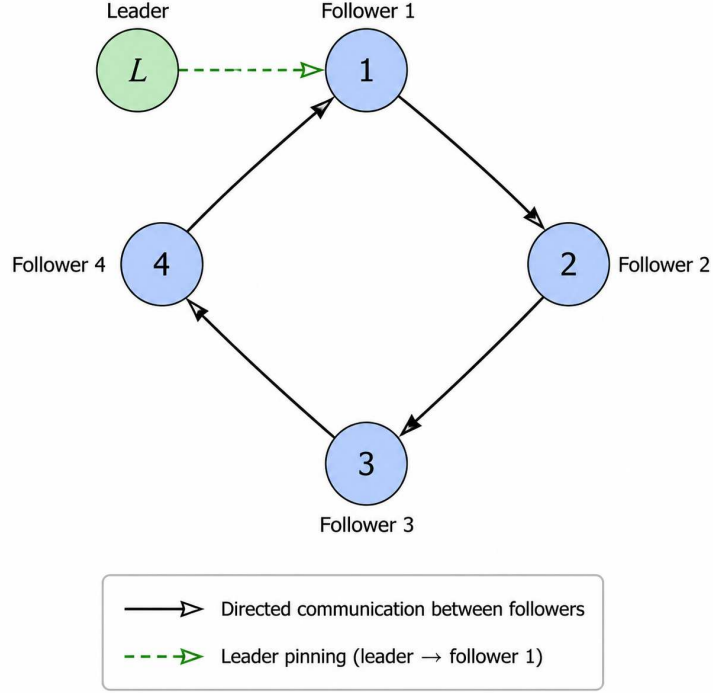
Fig. 2 Directed communication topology of the leader-follower network.
