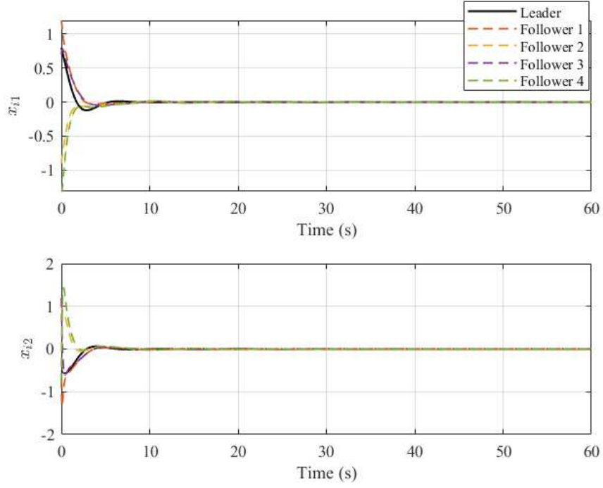
Fig. 3 State trajectories of the leader and heterogeneous followers in Example A.
