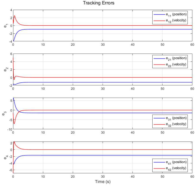
Fig. 9 Position and velocity tracking errors of the follower UGVs with respect to the leader in Example B.
