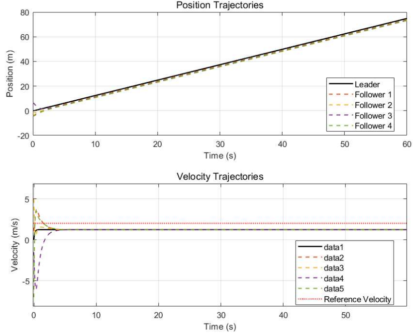
Fig. 7 Position and velocity trajectories of the leader and follower UGVs in Example B.
