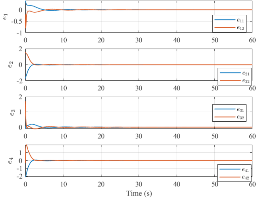
Fig. 4 Tracking errors of the four followers with respect to the leader in Example A.
