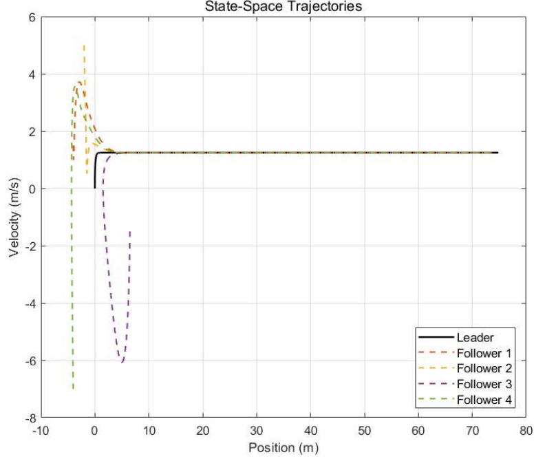
Fig. 8 State-space trajectories of the leader and follower UGVs in Example B.
