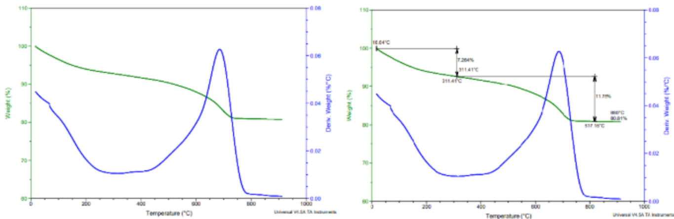
Figure 5 TGA/DTG curves of an internal section of a treated concrete sample from UHE Assis Chateaubriand (Acronal BS 796 + water + fumed nanosilica), at a heating rate of 10 °C/min
