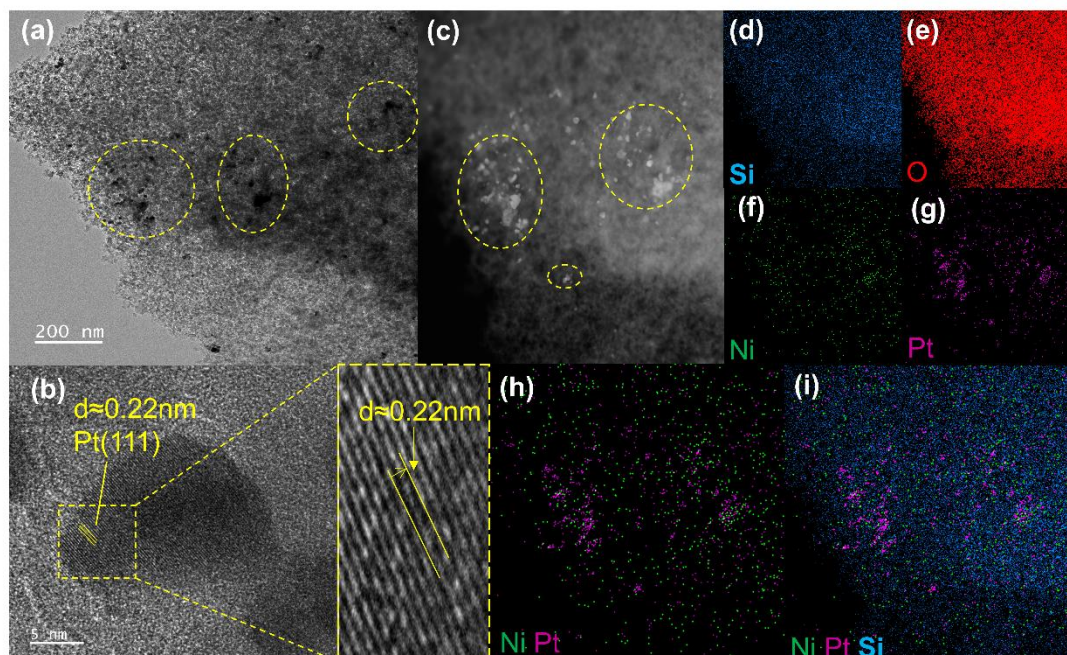
Fig. 3 TEM characterization of Pt/NiO x -SiO 2 catalyst. (a) TEM image; (b) HRTEM image with enlarged lattice fringe region; (c) HAADF-STEM image; (d-g) STEM-EDS elemental mappings of Si, O, Ni, and Pt; (h) Overlay elemental mapping of Ni and Pt; (i) Overlay elemental mapping of Ni, Pt, and Si
