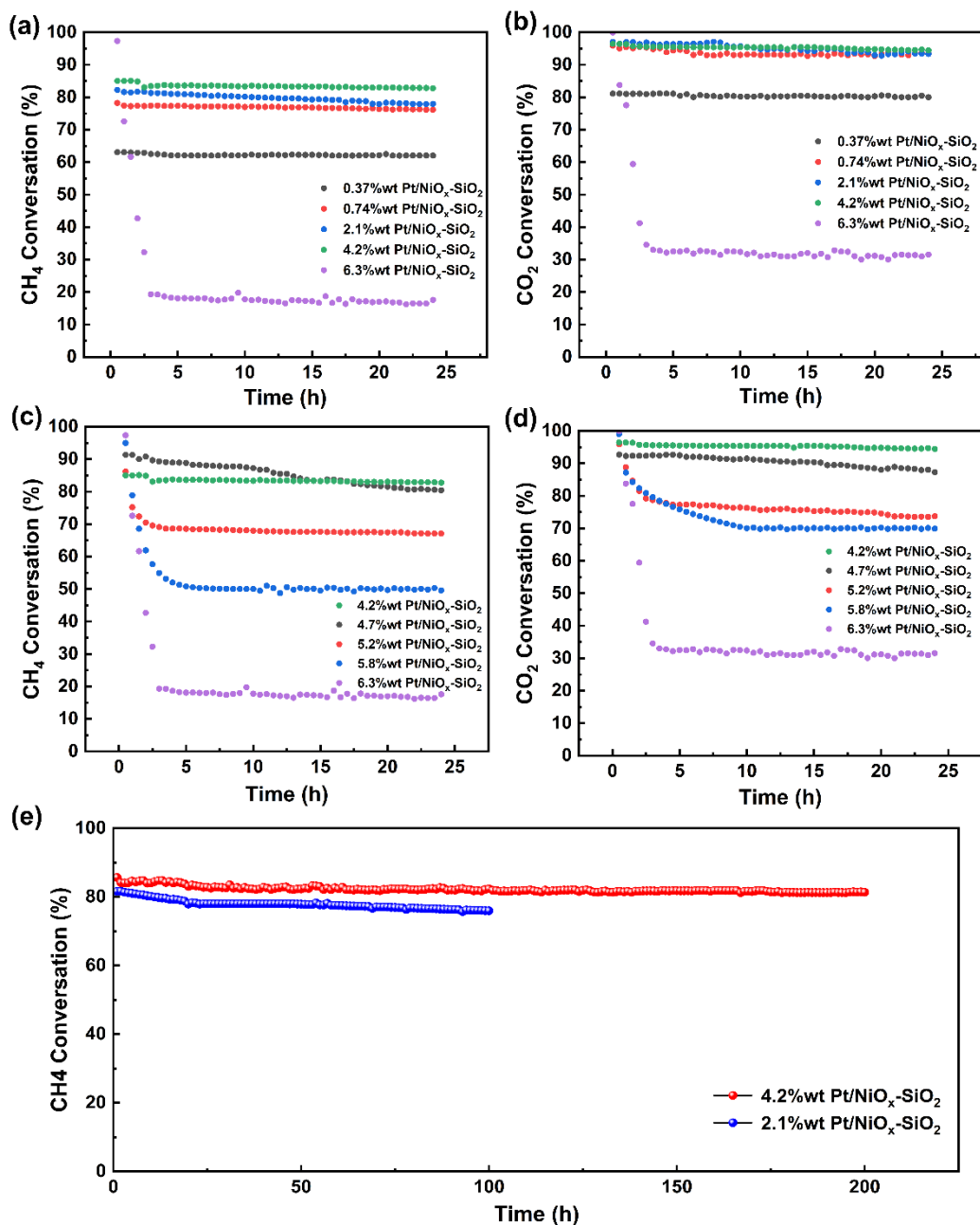
Fig. 6 DRM performance of Pt/NiO x -SiO 2 catalysts with different Pt loadings. (a) CH 4 and (b) CO 2 conversion over 24 h DRM for catalysts with broad Pt loading range (0.37-6.3wt%); (c) CH 4 and (d) CO 2 conversion over 24 h DRM for catalysts with optimized Pt loading range (4.2-6.3wt%); (e) CH 4 conversion over the 4.2wt% and 2.1wt% Pt/NiO x -SiO 2 catalysts during 200 and 100 h long-term stability tests
