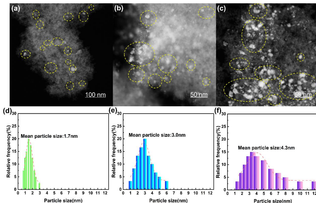
Fig. 4 HAADF-STEM images and corresponding particle size distributions of Pt/NiO x -SiO 2 catalysts with different Pt loadings. The particle size distribution was obtained by statistically analyzing approximately 50 Pt-containing particles from HAADF-STEM images. (a, d) 0.37wt% Pt/NiO x -SiO 2 ; (b, e) 4.2wt% Pt/NiO x -SiO 2 ; (c, f) 6.3wt% Pt/NiO x -SiO 2
