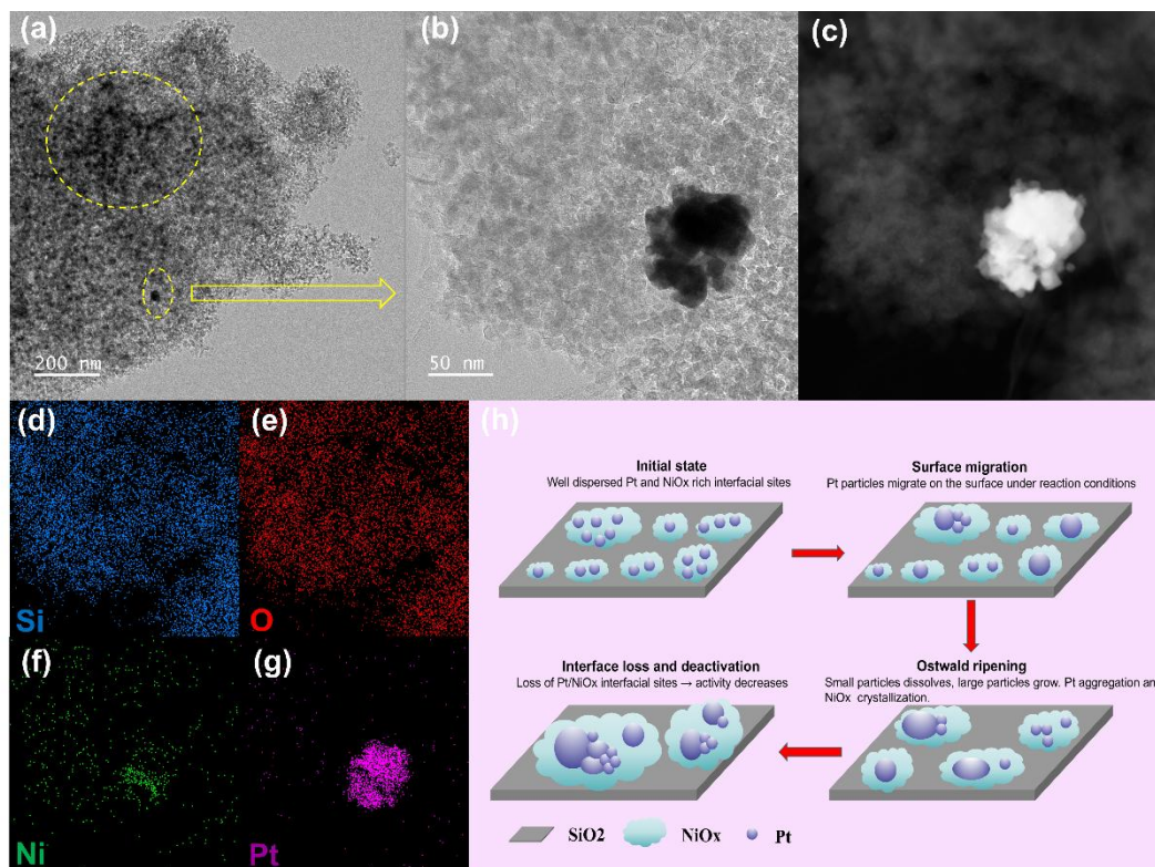
Fig. 9 Structural evolution and deactivation mechanism of high-loading Pt/NiO x -SiO 2 catalyst during DRM reaction. (a) TEM image, (b) enlarged TEM image, (c) HAADF-STEM image, and (d–g) STEM-EDS elemental mappings of Si, O, Ni, and Pt for the spent high-loading Pt/NiO x -SiO 2 catalyst after DRM reaction. (h) Schematic illustration of the proposed structural evolution and deactivation mechanism, involving Pt migration, Ostwald ripening, Pt aggregation, NiO x crystallization, and loss of Pt-NiO x interfacial active sites under DRM conditions.
