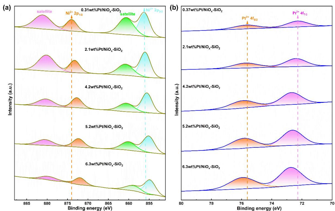
Fig. 5 XPS analysis of Pt/NiO x -SiO 2 with different Pt loadings. Fitting parameters of (a) Ni 2p and (b) Pt 4f XPS spectra for Pt/NiO x -SiO 2 catalysts with different Pt loadings
