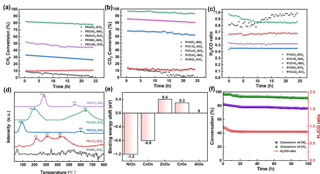
Fig.2 DRM performance, XPS Analysis and H 2 -TPR profiles of different oxide-supported catalysts. The DRM reaction conversion rates of the Pt/AlO x -SiO 2 , Pt/CrO x -SiO 2 , Pt/ZnO x -SiO 2 , Pt/NiO x -SiO 2 , and Pt/CoO x -SiO 2 catalysts for (a) CH 4 , (b) CO 2 , and (c) H 2 /CO; (d) Comparison of H 2 -TPR profiles of different oxide-supported catalysts; (e) Comparison of binding energy shifts of different oxide species relative to their standard oxide references; (f) CH 4 conversion, CO 2 conversion and H 2 /CO ratio of Pt/NiO x -SiO 2 for 100 h DRM reaction at 750 °C
