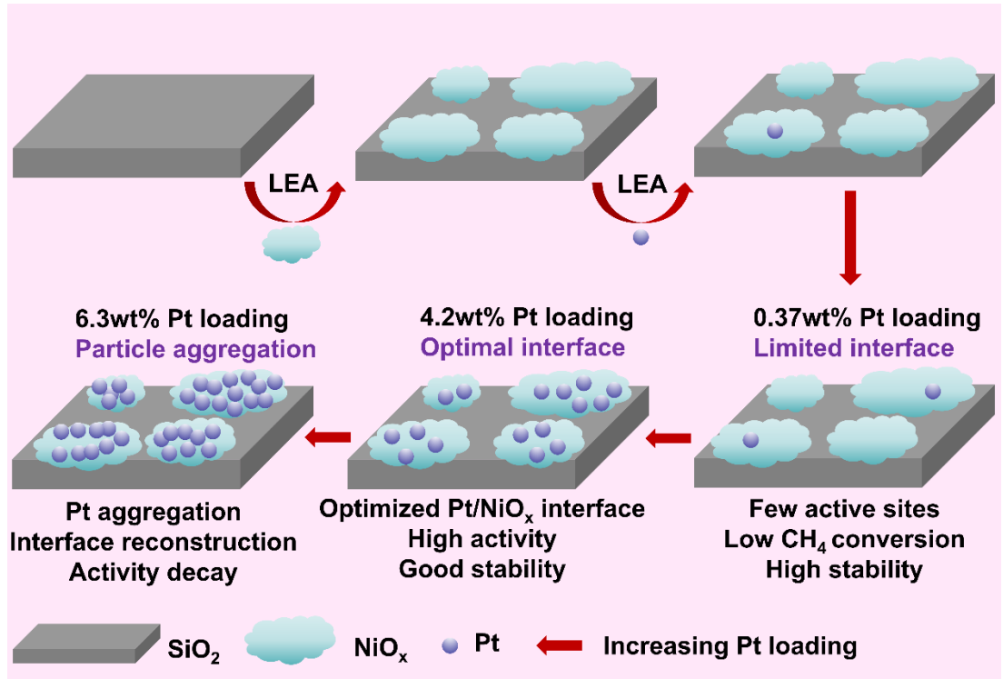
Fig.1 SANIs-inspired Pt catalysts via oxide modification and Pt loading optimization for regulating Pt dispersion, interfacial structure, and DRM performance
