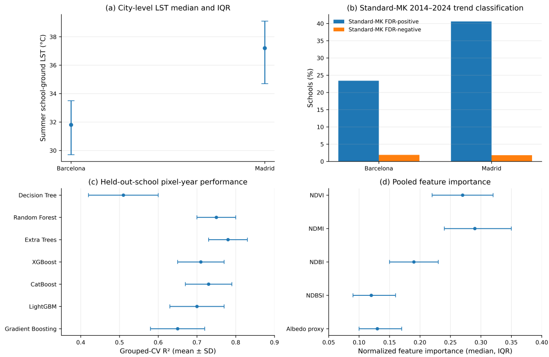
Figure 5. Core empirical results: (a) city median school-ground summer LST (IQR); (b) standard-MK FDR-positive/negative trend shares; (c) grouped-CV R^2 (mean \pm SD) for held-out-school pixel-year observations; and (d) Extra Trees feature importance (median, IQR).
