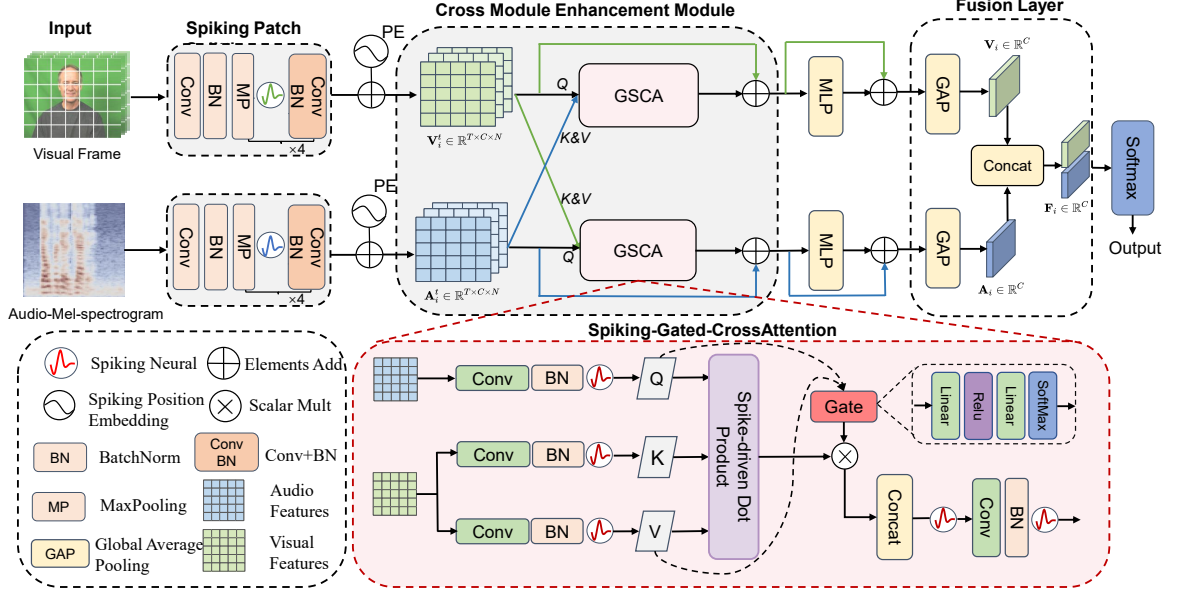
Fig. 2 Overview of GSCANet. Spikingformer-style Spiking Patch Splitting encoders process audio and visual inputs, followed by stacked bidirectional GSCA blocks with membrane-shortcut residual learning. The default G_4 gate uses JointQV to modulate attention outputs before spike firing; modality features are then pooled and concatenated for classification. Illustrative inputs are drawn from CREMA-D [2] and RAVDESS [19]
