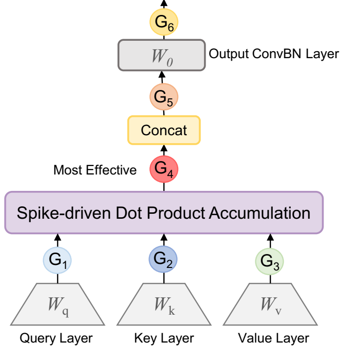
Fig. 1 Head-specific MLP bottleneck gating placements ( G_1 – G_6 ) in spiking cross-modal attention. The W_q , W_k , W_v , and W_o operators are kernel-1 ConvBN projections, and attention uses SDDPA without Softmax. Placements span Q/K/V projections ( G_1 – G_3 ), attention output ( G_4 ), concatenation ( G_5 ), and block output ( G_6 ); G_4 is the default
