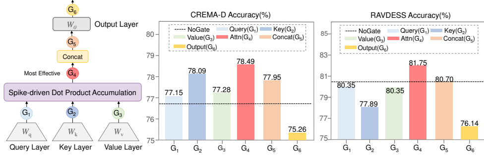
Fig. 4 Accuracy comparison of different gating placements on CREMA-D and RAVDESS. The compact labels Attn and Output denote attention-output ( G_4 ) and block-output ( G_6 ) gating, respectively. Attention-output gating achieves the best performance on these synchronized audiovisual emotion benchmarks
