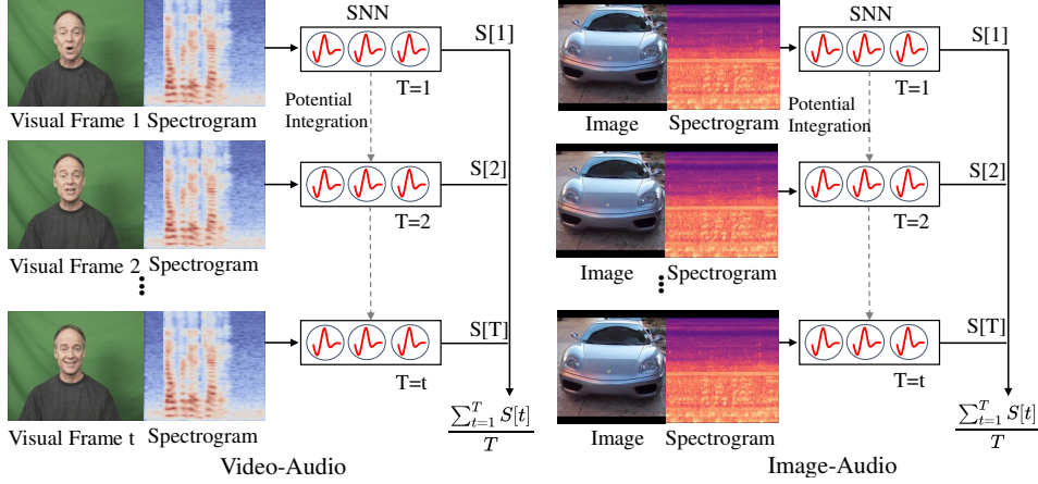
Fig. 3 Unified spiking encoding for heterogeneous audiovisual data. Left: video frames from CREMA-D [2] and RAVDESS [19] are aligned with simulation steps T . Right: static images from UrbanSound8K-AV and CIFAR10-AV [7] are replicated across T steps for temporal processing
