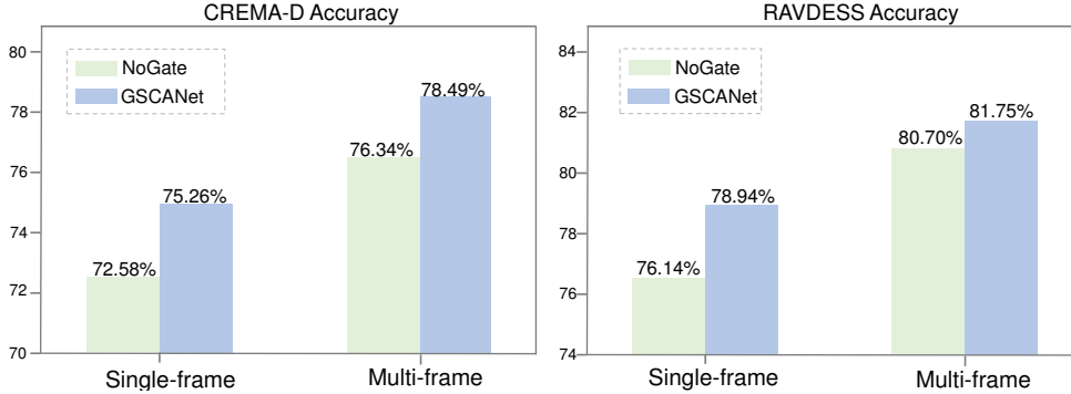
Fig. 5 Effect of single-frame vs. multi-frame visual input on CREMA-D and RAVDESS. Multi-frame input improves the baseline and synergizes with GSCA gating
