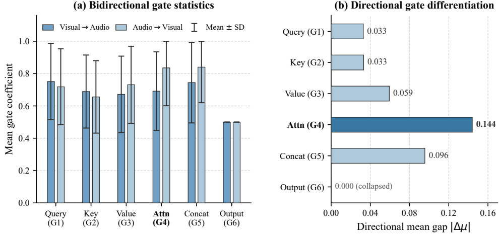
Fig. 6 Bidirectional gate statistics for G_1 – G_6 on RAVDESS. (a) Mean sigmoid coefficients for visual-to-audio and audio-to-visual modulation; whiskers show one standard deviation. (b) Absolute directional mean gap |\Delta\mu| = |\mu_{V \rightarrow A} - \mu_{A \rightarrow V}| . G_4 shows the largest gap, whereas G_6 collapses to 0.5; these values are descriptive diagnostics
